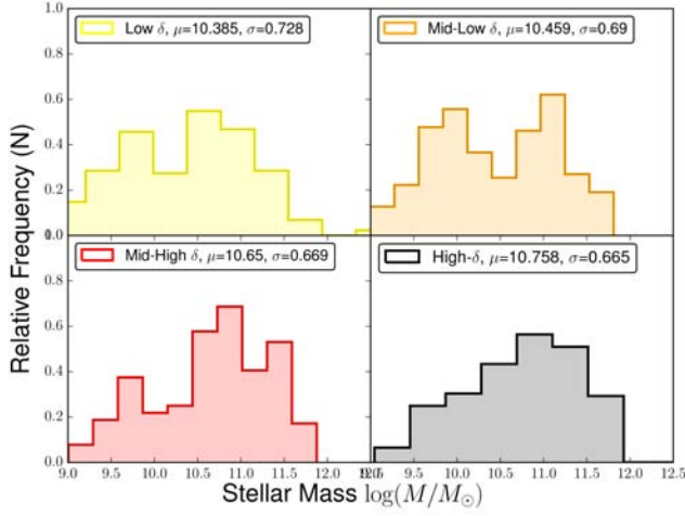
Figure 3. Distributions of stellar mass ( \log(M/M_{\odot}) ) for the four different environmental bins that make up the sample used in this work. Galaxy masses are drawn from the Nasa Sloan Atlas catalogue (NSA1). The mean \mu and 1-\sigma value of each distribution are quoted in the legend.
