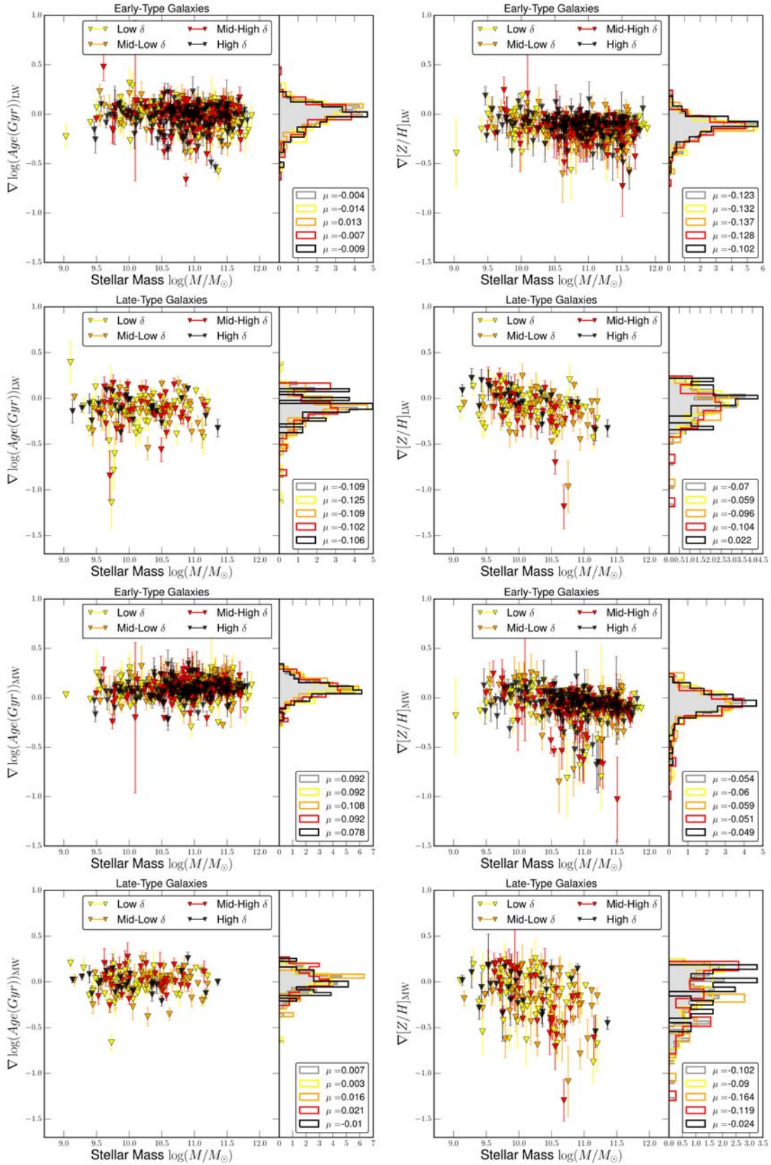
Figure 5. Light and mass-weighted stellar population gradients in age (left-hand panels) and metallicity (right-hand panels) as a function of galaxy mass for different local environmental densities. Plots with axis label subscripted ET are for early-type galaxies and LT represents late-type galaxies. The different marker colours indicate the four environmental densities described in Section 3.1. The right-hand sub-panels show the distribution of the gradients for the whole sample and for the four different environment bins. The median value \mu for each distribution is also quoted in the legend.
