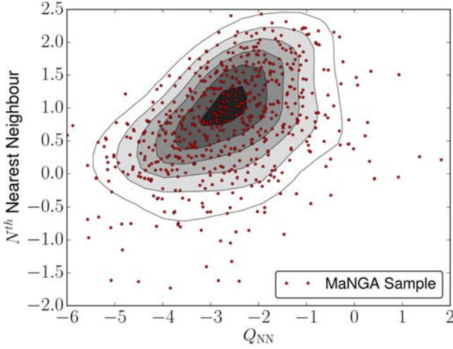
Figure 4. Figure showing the comparison between the environments calculated using the N^{th} nearest neighbour method and the Q parameter. The red points represent individual galaxies used in this work, the grey contours represent the density of points. The Spearman's rank correlation coefficient is 0.4.
