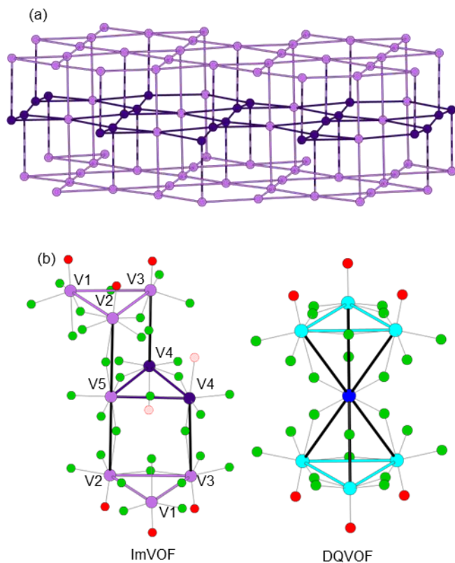
Figure 2. The tri-layer slabs of kagome-like networks in ImVOF are shown in (a) with V^{4+} and V^{3+}/V^{4+} sites in light and dark purple, respectively. The V^{4+} – V^{4+} contact pathways are shown by light purple solid lines and those of V^{4+} – V^{3+}/V^{4+} in striped light and dark purple. (b) The connectivity between the vanadium species in ImVOF (left) and DQVOF (right). In DQVOF, the V^{4+} cations are shown in cyan and V^{3+} cations in dark blue. The connectivity between different vanadium species in adjacent layers, which are linked through bridging fluoride ions, is depicted by the solid black lines.
