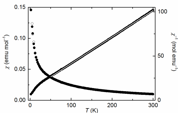
Figure 3. Magnetic (left) and inverse (right) susceptibilities of ImVOF measured in a 5 T field in a zero field cooled (closed circles) field cooled (open circles) cycle. The solid white line shows the Curie-Weiss fit applied to the inverse susceptibility data over the temperature range 50 – 300 K.
