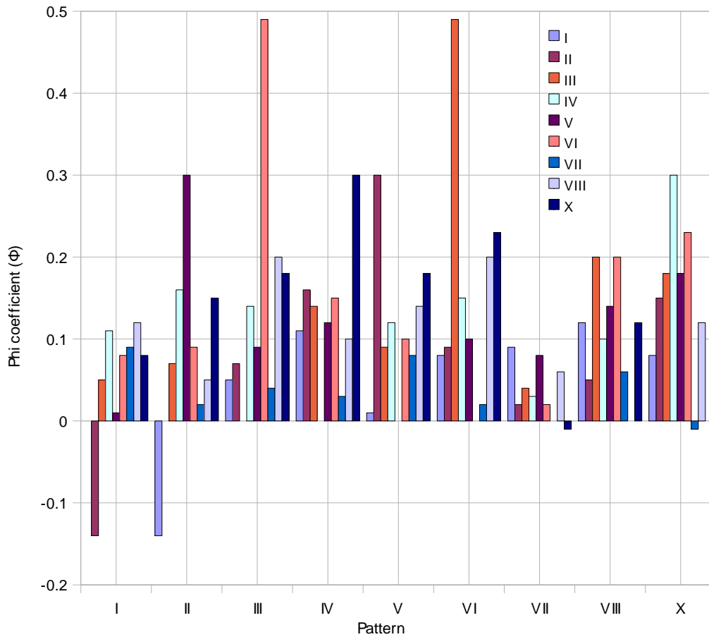
Fig. 1: Graphed phi coefficients for pattern co-occurrences (trilaterals)
