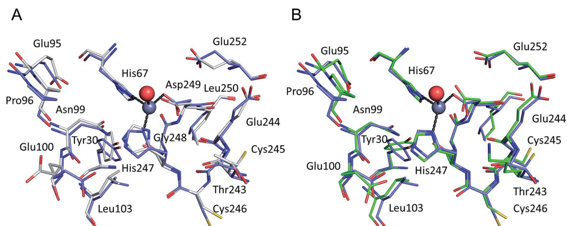
Fig. 2 The all-atoms superposition of residues within 8 Å from \text{Zn}^{2+} in site a of HSA– \text{Zn}^{2+} complex (5IJF, blue), and corresponding residues in (a) native HSA structure (1A06, white) and (b) ESA– \text{Zn}^{2+} structure (2.5 mM \text{Zn}^{2+} , pH 7.4 – 5IIH, green). Zinc ions are shown in grey, oxygen in red, sulfur in yellow, nitrogen in dark blue, coordination bonds with \text{Zn}^{2+} ion are marked with black dashed lines. Residue numbers refer to HSA.
