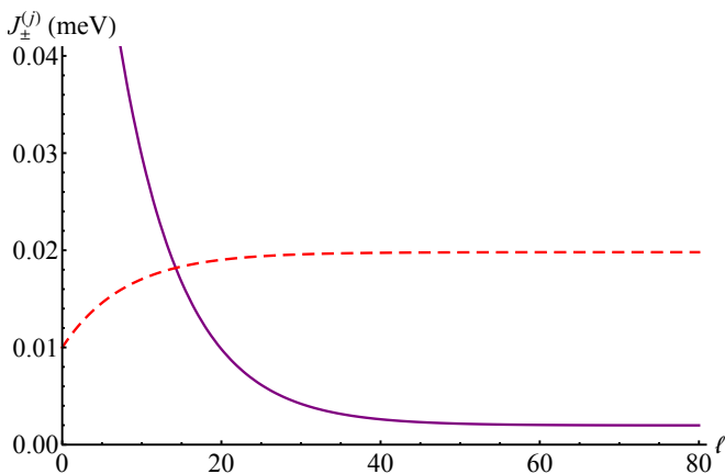
FIG. 4: Change in anomalous tunnel couplings, J_{\pm}^{(j)} , with scaling parameter \ell , as given by Eq. (3) for t_1 = 0.1\text{meV} , t_2 = 0.01\text{meV} and further parameters 65 based on a recent experiment. 45 The solid purple and dashed red lines show J_{\pm}^{(1)} and J_{\pm}^{(2)} , respectively. The vertical dashed black line is the value of \ell corresponding to the crossover temperature T_c . The couplings display a rapid, exponential change from their initial values of t_1 and t_2 as \ell increases. This high temperature sensitivity even far above T_c is due to the large ratio t_1/t_2 = 10 .
