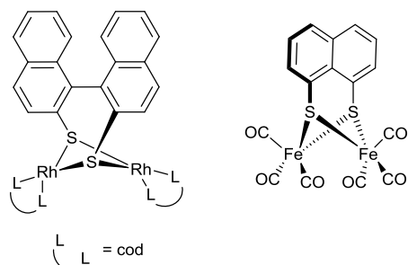
Figure 3 Examples of catalysts bearing dithiolato ligands [asymmetric hydroformylation (left) and electron transfer catalyst (right)]
