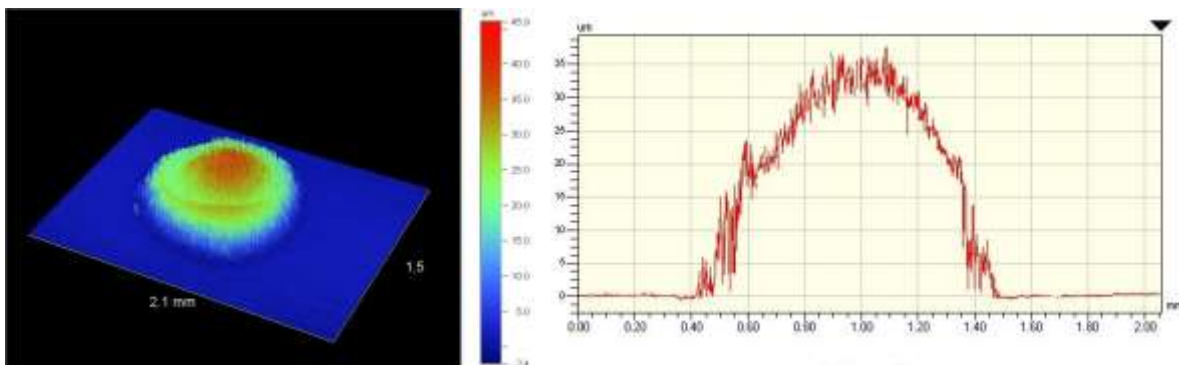
Figure 6. Left: 3D reconstruction of a scan using a white light interferometer of a foam. Right: A lineout taken through the centre of the foam to give a height profile above the level of the array mount.
