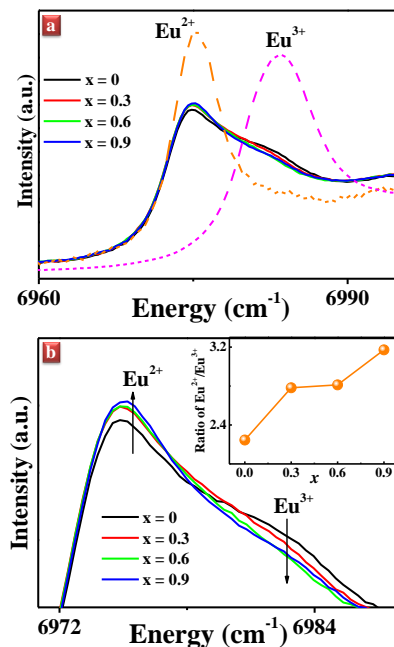
Figure 2. (a) Eu L 3 -edge XANES spectra of Sr x Ca 0.993-x AlSiN 3 :Eu 2+ 0.007 (x = 0 to 0.9). (b) Dependence of Eu 2+ /Eu 3+ within the range of 6970 cm -1 to 6990 cm -1 ; the relative intensity of Eu 2+ /Eu 3+ is shown in the inset.
