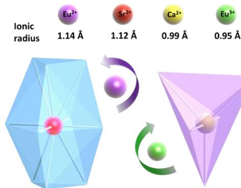
Figure 3. Schematic drawing of local structures. The charge variation of Eu 3+ activators at the selected Ca 2+ sites and Eu 2+ at the Sr 2+ sites is the proposed mechanism for cation substitution.
