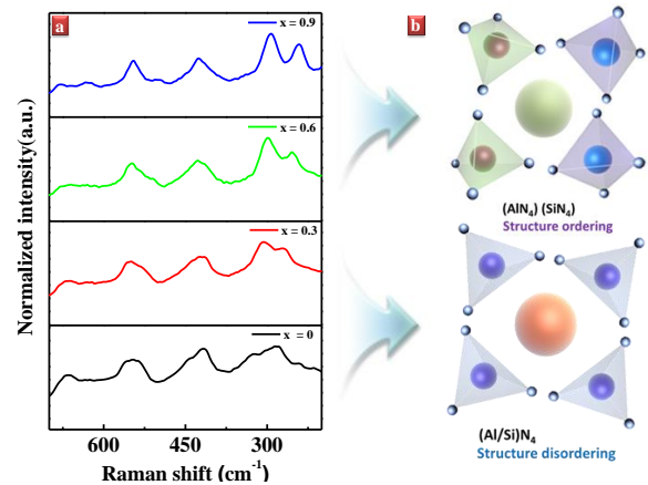
Figure 5. (a) Raman spectrum of \text{Sr}_x\text{Ca}_{0.993-x}\text{AlSiN}_3:\text{Eu}^{2+} ( x = 0, 0.3, 0.6, and 0.9 ). (b) Schematic graph of separate clusters in the lattice.
