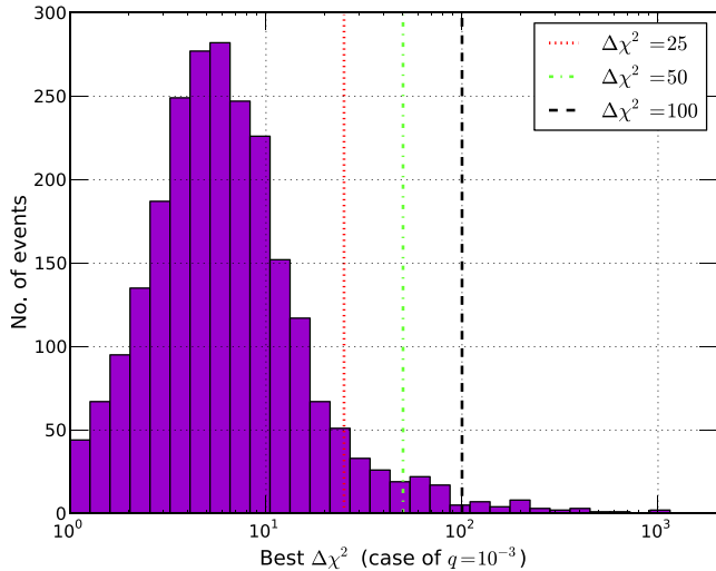
Figure 5. Distribution of the best \Delta\chi^2 (highest value in detection map) for the sample of 2433 light curves generated for a mass ratio q = m_p/m_* = 10^{-3} . The detection maps are generated for three threshold values which are marked with the dotted (red), dot-dashed (green) and dashed (black) lines.
