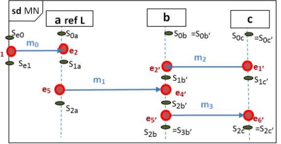
Fig. 5. A SD showing composition behaviour.
