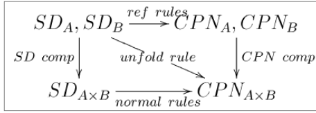
Fig. 7. SD to CPN transformation paths for complex behaviour.
