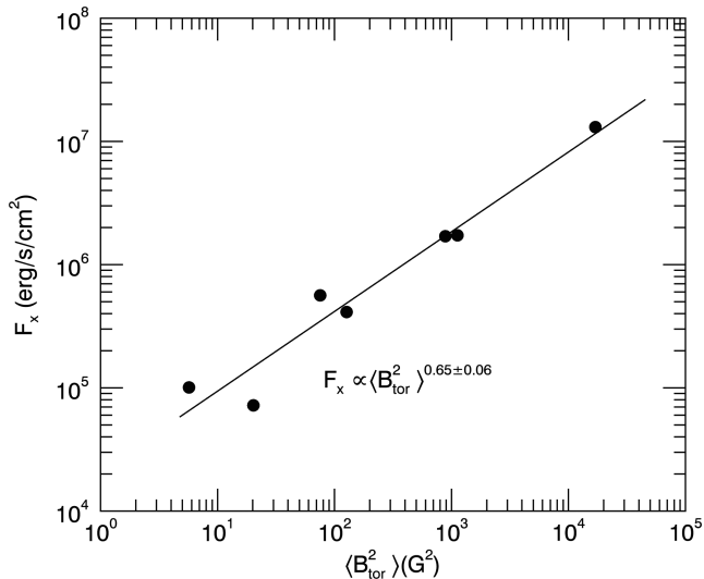
Figure 2. Relation between F_x and \langle B_{\text{tor}}^2 \rangle does not show a break at F_x \sim 10^6 erg cm ^{-2} s ^{-1} . Solid line is a power law fit the data. Because \langle B_{\text{tor}}^2 \rangle and \langle B_{\text{pol}}^2 \rangle are correlated (See et al. 2015), correlations between F_x and \langle B_{\text{pol}}^2 \rangle or \langle B^2 \rangle also exist (see Table 3).
