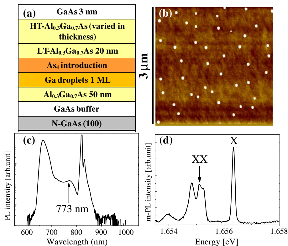
Figure 1 Schematics of structures, AFM image, and the PL peaks of low-density GaAs DE QDs. (a) Schematics of structures of low-density GaAs DE QDs as a function of thickness of HT- \text{Al}_{0.3}\text{Ga}_{0.7}\text{As} (2, 25, 50, 85 nm), (b) AFM image ( 3 \mu\text{m} \times 3 \mu\text{m} ) of low-density GaAs DE QDs (approximately 4 QDs/ \mu\text{m}^2 ) on \text{Al}_{0.3}\text{Ga}_{0.7}\text{As}/\text{GaAs} substrate, and (c) macro-PL (log scale) and (d) \mu -PL (exciton, biexciton peaks) spectra of low-density GaAs DE QDs with 105-nm capping at low temperature (12 ~ 16 K).
