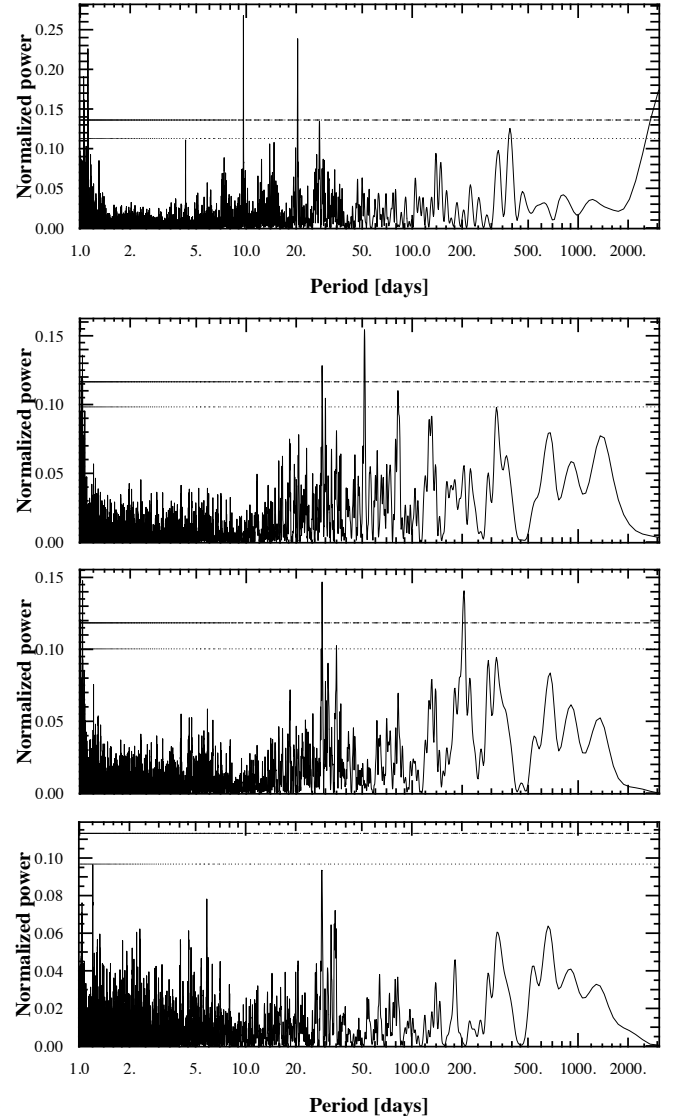
Fig. 10. Periodogram of the RV data of HD 40307 ( top panel ), and of the residuals around models with three ( second from top ), four ( second from bottom ), and five ( bottom ) Keplerian signals in addition to a cubic function to take into account the long-term trend produced by the magnetic cycle of the star. The horizontal dotted and dashed lines represent the 10% and 1% false alarm probability levels, respectively.
