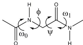
Figure 1: Dipeptide model dihedral angle representations.
