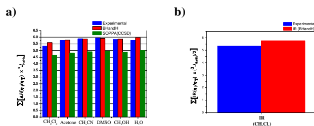
Figure 7: Sum of the weighted contributions [(n_i/n_T) \times J] for the ^3J_{\text{HaHb}} couplings of all Ac-Gly-NHMe conformers (obtained as ^3J_{\text{H10H11}} + ^3J_{\text{H11H13}}/2 ); SSCCs were obtained in different solvents (B3LYP-D3/aug-cc-pVDZ level optimisation) by using the IEF-PCM model. a) conformer contributions obtained from \Delta H populations and b) conformer contributions obtained from experimental IR populations in \text{CH}_2\text{Cl}_2 (using BHandH/EPR-III calculated ^3J_{\text{HH}} ).
