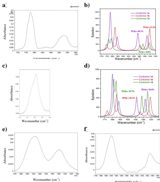
Figure 4: IR Amide I (C=O stretching) and II (N-H stretching) regions for 1 . a) Experimental spectrum in \text{CH}_2\text{Cl}_2 . b) Theoretical spectrum in \text{CH}_2\text{Cl}_2 . c) Experimental spectrum in \text{CH}_3\text{CN} (Amide I only), since \text{CH}_3\text{CN} absorbs strongly in the Amide II region. d) Theoretical spectrum in \text{CH}_3\text{CN} . e) Experimental spectrum in \text{H}_2\text{O} . f) Experimental spectrum in \text{D}_2\text{O} . Theoretical spectra from conformers 1a , 1b and 1d IR intensities/populations obtained at the B3LYP-D3/aug-cc-pVDZ level with the IEF-PCM model.
