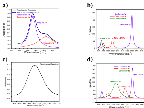
Figure 3: IR N-H bond stretching region for 1 . a) Experimental spectrum in \text{CH}_2\text{Cl}_2 . b) Theoretical B3LYP-D3/aug-cc-pVDZ spectrum in \text{CH}_2\text{Cl}_2 (IEF-PCM). c) experimental spectrum in \text{CH}_3\text{CN} . d) Theoretical B3LYP-D3/aug-cc-pVDZ spectrum in \text{CH}_3\text{CN} (IEF-PCM). Conformer populations are indicated in each spectrum. Theoretical populations obtained at [B3LYP-D3/aug-cc-pVDZ] level. Experimental IR populations were corrected by calculated conformer molar absorptivities.
