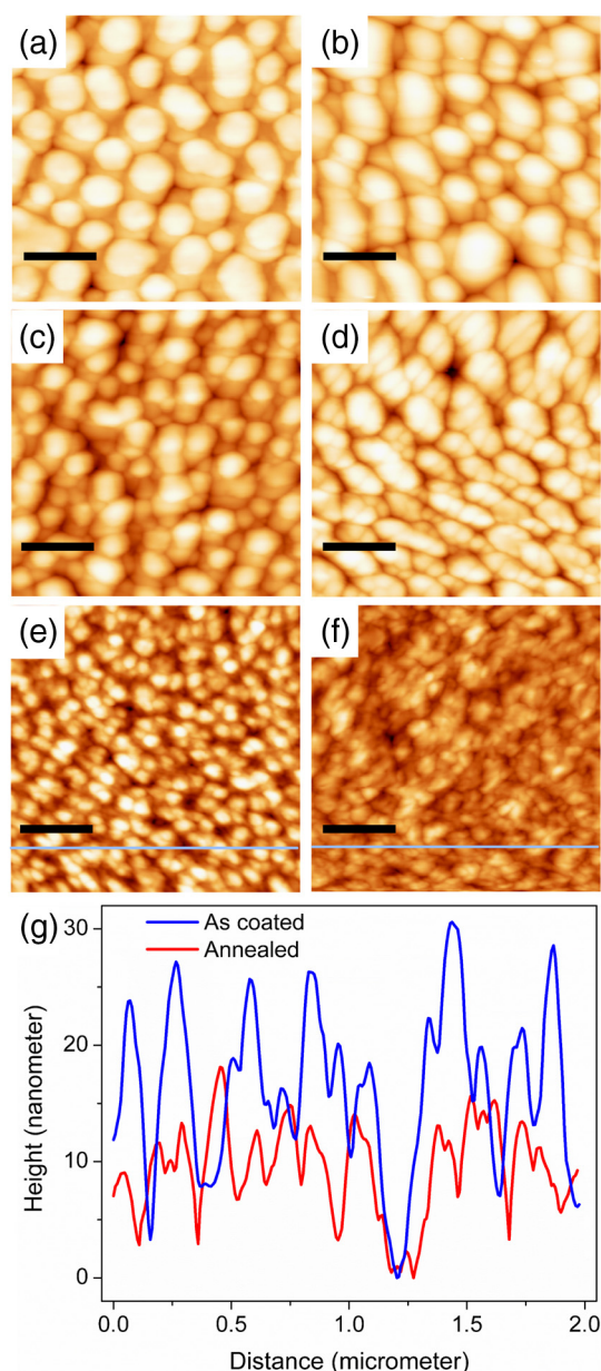
Fig. 9 AFM topography images of DPP-BZ:PC 71 BM blends: (a) and (b) with donor:acceptor (D:A) ratio of 1:2, z-scale of 95 nm, (c) and (d) with D:A ratio of 1:1.5, z-scale of 90 nm, (e) and (f) with D:A ratio of 1:0.7, z-scale of 40 nm. (a), (c), and (e) are as coated, and (b), (d), and (f) are annealed films. Scale bar = 0.5 \mu m. The height profile along the grey line of (e) and (f) is shown in (g).
