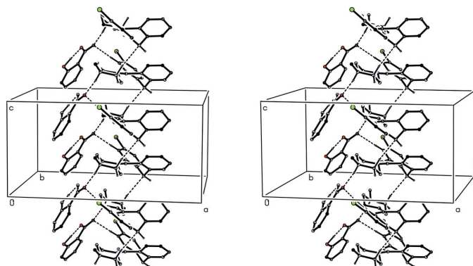
Figure 9 A stereoview of part of the crystal structure of compound (III) showing the formation of a hydrogen-bonded C(7)\ C_2^2(11)[R_3^2(19)] chain of rings running parallel to [001] . For the sake of clarity, H atoms bonded to the C atoms not involved in the motif shown have been omitted.
