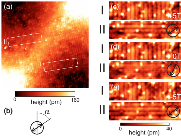
FIG. 7: Characterization of In-Plane component of Magnetization (a) STM image of a twin boundary (taken at field B = 0\text{T} ), the stripes are only seen on the right side of the boundary, (b) scheme explaining the symbol used in panels (c)-(e) for indicating the magnetization direction of the tip and the angle \alpha , (c)-(e) STM topographies cut out from images taken in the same location as (a) at magnetic fields of +5\text{T} , 0\text{T} , and -5\text{T} , all with the same tip ( V_b = 80\text{mV} , I_t = 100\text{pA} ). The in-plane magnetization direction of the tip extracted from the topographies is shown by a double arrow in the left panels (see b). Regions I and II shown in panels (c)-(e) are indicated by solid lines in (a), panel (d) is cut out from the image shown in (a).
