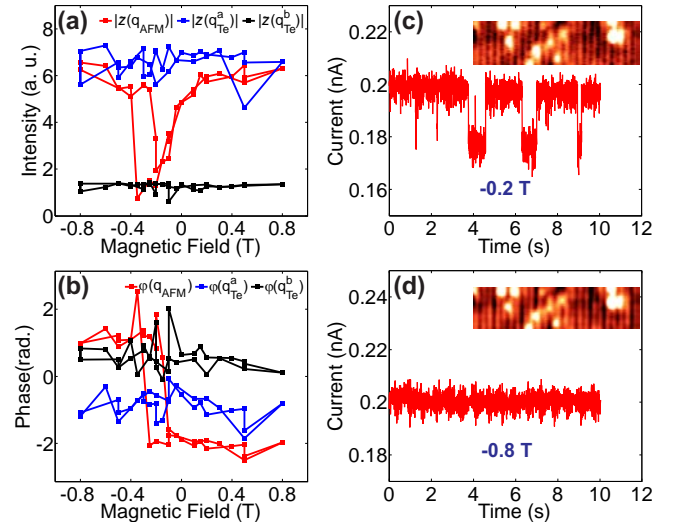
FIG. 6: Magnetization dynamics of a ferromagnetic tip. (a) Amplitudes |\tilde{z}(\mathbf{q}_{\text{AFM}}^a)| , |\tilde{z}(\mathbf{q}_{\text{Te}}^b)| and |\tilde{z}(\mathbf{q}_{\text{Te}}^c)| and (b) phase \varphi(\mathbf{q}_{\text{Te}}^a) , \varphi(\mathbf{q}_{\text{Te}}^b) and \varphi(\mathbf{q}_{\text{AFM}}) as a function of magnetic field for a magnetic tip which shows a phase shift at fields of -0.4\text{T} and -0.2\text{T} . (c) Tunneling current as a function of time measured at -0.2\text{T} , right at the field where the phase shift occurs, obtained at V_b = -80\text{mV} and with open feedback loop, it shows spontaneous transitions between two magnetizations of the tip, the noise also appears in topographic images taken at the same field as shown in the inset. (d) At slightly larger or smaller fields, the current does not exhibit the transitions, shown here for a magnetic field of -0.8\text{T} , the noise also disappears in topographic images.
