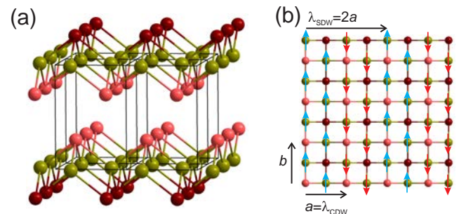
FIG. 1: Crystal structure of FeTe. (a) Crystal structure of FeTe showing four unit cells, Te atoms are shown in different red tones, Fe atoms in yellow. (b) Surface termination when cleaving between FeTe layers, the surface has a Te termination. The known magnetic structure obtained from neutron scattering is indicated by red and blue arrows[7, 12].
