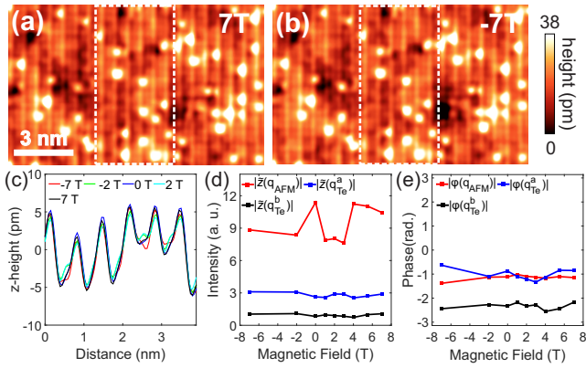
FIG. 3: Magnetic field dependence of images obtained with an antiferromagnetic tip. (a,b) STM topographies obtained at magnetic field of +7T (a) and -7T (b), both taken in the same location. The stripes due to the magnetic contrast maintain the same phase with respect to defects on the surface ( V_b = 80\text{mV} , I_t = 100\text{pA} ). (c) line cuts extracted by averaging in a direction normal to \mathbf{q}_{\text{AFM}} at selected fields from a series of images at the location marked by a white dashed rectangle in (a) and (b). (d) Field-dependence of the magnetic contrast, the amplitudes of the Fourier components of the magnetic modulation |\tilde{z}(\mathbf{q}_{\text{AFM}})| as well as for the atomic lattice vectors |\tilde{z}(\mathbf{q}_{\text{Te}}^{\text{a}})| and |\tilde{z}(\mathbf{q}_{\text{Te}}^{\text{b}})| are shown. (e) Phase \varphi(\mathbf{q}) = \arg(\tilde{z}(\mathbf{q})) of the Fourier components at \mathbf{q}_{\text{Te}}^{\text{a}} ( = \mathbf{q}_{\text{CDW}} ), \mathbf{q}_{\text{Te}}^{\text{b}} and \mathbf{q}_{\text{AFM}} as a function of field.
