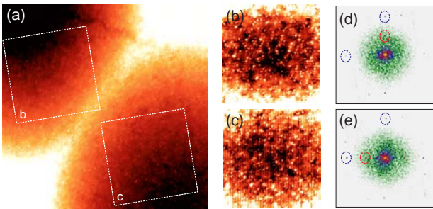
FIG. 5: Intensity of CDW peak (a) STM image of a twin boundary (taken at field B = 0\text{T} ), the stripes are mainly seen on the right side of the boundary. Letters b and c in panel (a) mark areas where topographies shown in (b) and (c) have been cut out, (d) and (e) show their Fourier transforms. It can be seen that the peaks of the atomic lattice (marked by blue ellipses) are more intense in the direction of the SDW wave vector (marked by a red ellipse). Since both are taken with the same tip, this asymmetry has to be related to a modulation of the charge density near the Fermi level ( V_b = 80\text{mV} , I_t = 200\text{pA} ).
