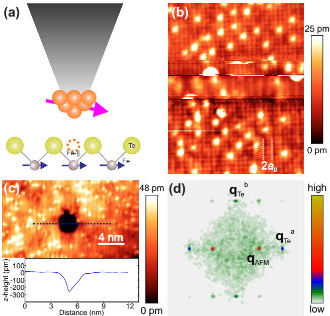
FIG. 2: Preparation of Magnetic tips on FeTe. (a) Schematic illustration of the process of picking up excess iron atoms on \text{Fe}_{1+y}\text{Te} to prepare a ferromagnetic tip. (b) Topographic STM image showing how a tip without magnetic contrast turns into one which exhibits magnetic contrast due to a tip change ( V_b = -80\text{mV} , I_t = 1.5\text{nA} ). Atoms are frequently moved or picked-up by scanning with a rather large tunneling current of up to a few nA. (c) STM image ( V_b = 90\text{mV} , I_t = 0.2\text{nA} ) of hole left behind due to a tip indentation. The line profile across the hole is shown. The hole indicates that an FeTe cluster was picked up. (d) Fourier transform \tilde{z}(\mathbf{q}) of a topography which exhibits magnetic contrast showing peaks corresponding to the square lattice of Te atoms ( \mathbf{q}_{\text{Te}}^a and \mathbf{q}_{\text{Te}}^b ) and the antiferromagnetic order ( \mathbf{q}_{\text{AFM}} ).
