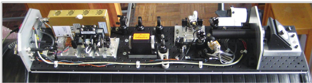
Figure 2. The lidar laser transmitter attached to the top of the receiver telescope, showing (left-to-right) the Nd:YLF pump laser, the OPO, the beam-expanding lenses and a 45° mirror to direct the output down onto the telescope axis.
