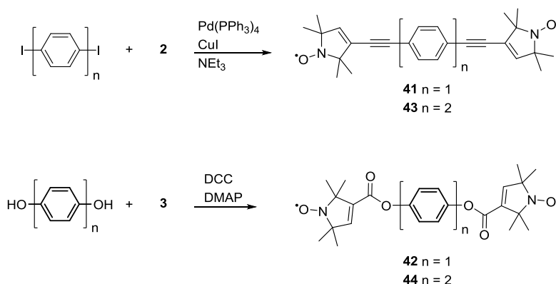
Scheme 5. Synthesis of biradical model systems with variable spacer length and conjugation.
