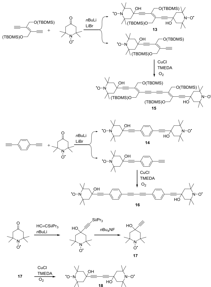
Scheme 2. Synthesis of a series of biradical model systems based on oxidative Hay couplings.
