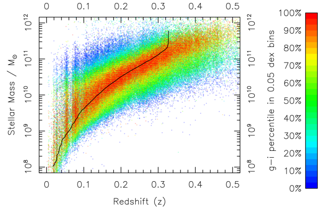
Figure 1. The variable stellar mass redshift selection limit. In each vertical M \pm 0.025 dex bin the cumulative density function (CDF) of apparent g - i colour is calculated. Depending on where a galaxy appears in the CDF given its stellar mass the colour of the data point is different: relatively bluer (redder) g - i colour galaxies are bluer (redder) data points. The black line shows the selection limit and is imposed at the 95th percentile for each bin.
