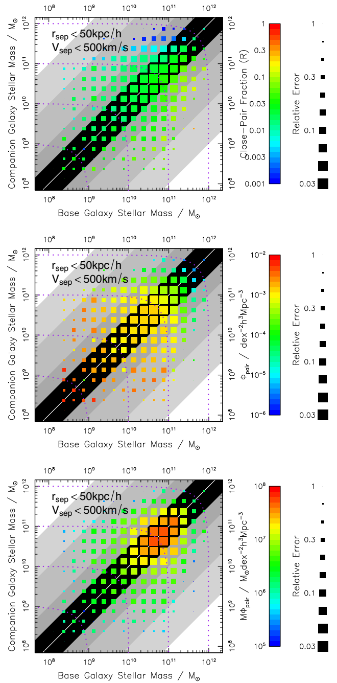
Figure 8. Pair properties for r_{\text{sep}} < 50 \text{ kpc/h} and v_{\text{sep}} < 500 \text{ km s}^{-1} sample ( PS_{r50v500} ) true pair corrected using the mock catalogues ( W_{\text{TP-mock}} , see Section 3.4). For more information see the caption for Fig. 7.
