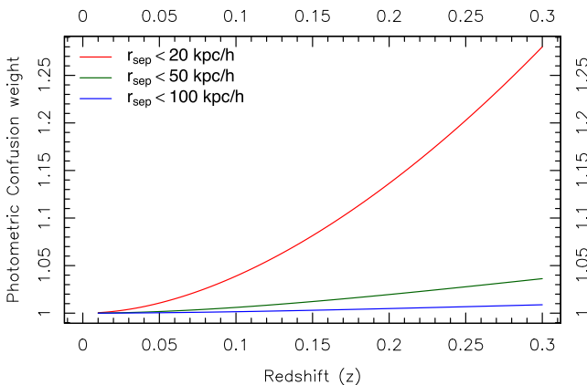
Figure 5. The weighting applied to an observed pair at a given redshift within specified projected separation limits. This accounts for the sharp fall in close pairs within 3 arcsec on the sky, which at a redshift of 0.3 can be a substantial fraction of the pair search radius.
