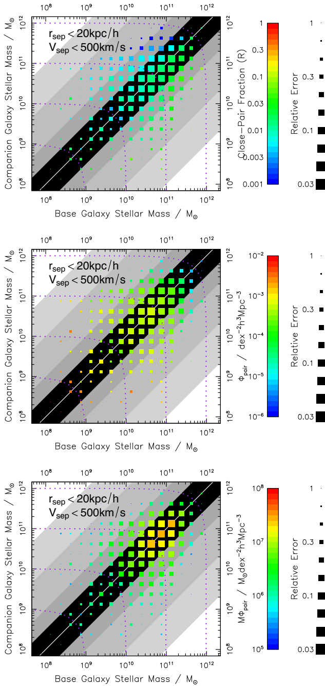
Figure 7. Pair properties for r_{\text{sep}} < 20 \text{ kpc/h} and v_{\text{sep}} < 500 \text{ km s}^{-1} sample ( PS_{r20v500} ) true pair corrected using the mock catalogues ( W_{\text{TP-mock}} , see Section 3.4). Top panel shows the observed pair fraction for the y-axis companion galaxy per stellar mass interval of the x-axis base galaxy. Middle panel shows the observed pair number density for the y-axis companion galaxy per stellar mass interval of the x-axis base galaxy. Bottom panel shows the observed minor accreting mass stellar mass density for the y-axis pair galaxy per stellar mass interval of the x-axis base galaxy (the number density of the pairs multiplied by the mass of the less massive galaxy in any close pair). In all panels the black background region shows the regime of major mergers (mass ratio within a factor of 0.5 dex), subsequent lightening grey regions show increasing decades in merger mass ratio. The purple lines show different merger mass products ranging from 10^8 to 10^{12} M_{\odot} .
