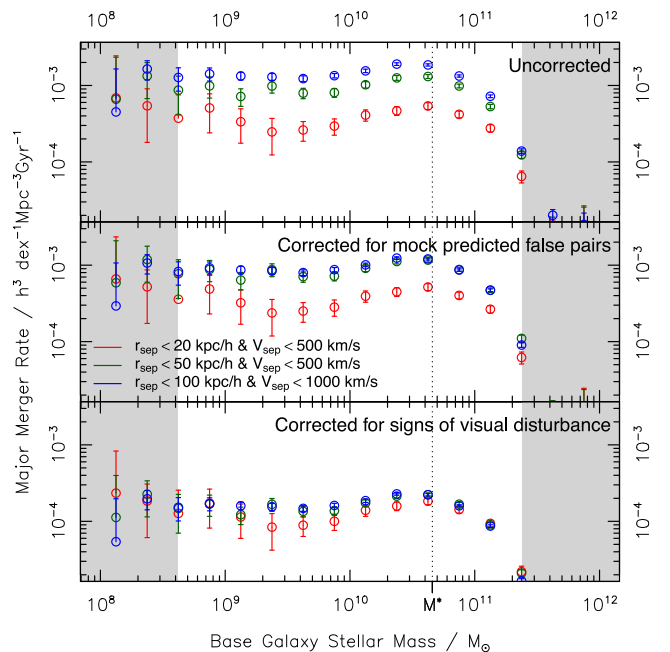
Figure 14. Major merger rates as a function of stellar mass for different dynamical pair selections. This is a simplified representation of the information presented in Figs 7–9 combined with estimates of merger time-scale for different stellar mass close pairs taken from Kitzbichler & White (2008). The Kitzbichler & White (2008) mappings naturally account for false close pairs due to their calibration to simulated data, so we expect the top panel (applying it to our ‘uncorrected close pair fractions’) to be the most representative of the true merger rates.
