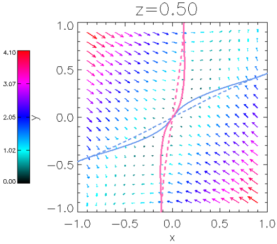
Fig. 3: Arrows display the initial Lorentz force in the plane z = 0.5 for the main experiment with initial current j_{sep} = 1.5 . The pale-blue/pink lines indicate where the separatrix surfaces from the lower/upper nulls of the initial (dashed) and equilibrium (solid) magnetic fields intersect the plane. The arrows indicate the strength (by their size and colour) and direction of the Lorentz force in the plane. The length of the arrows has been normalised to the maximum value of |\mathbf{j} \times \mathbf{B}| in the domain.
