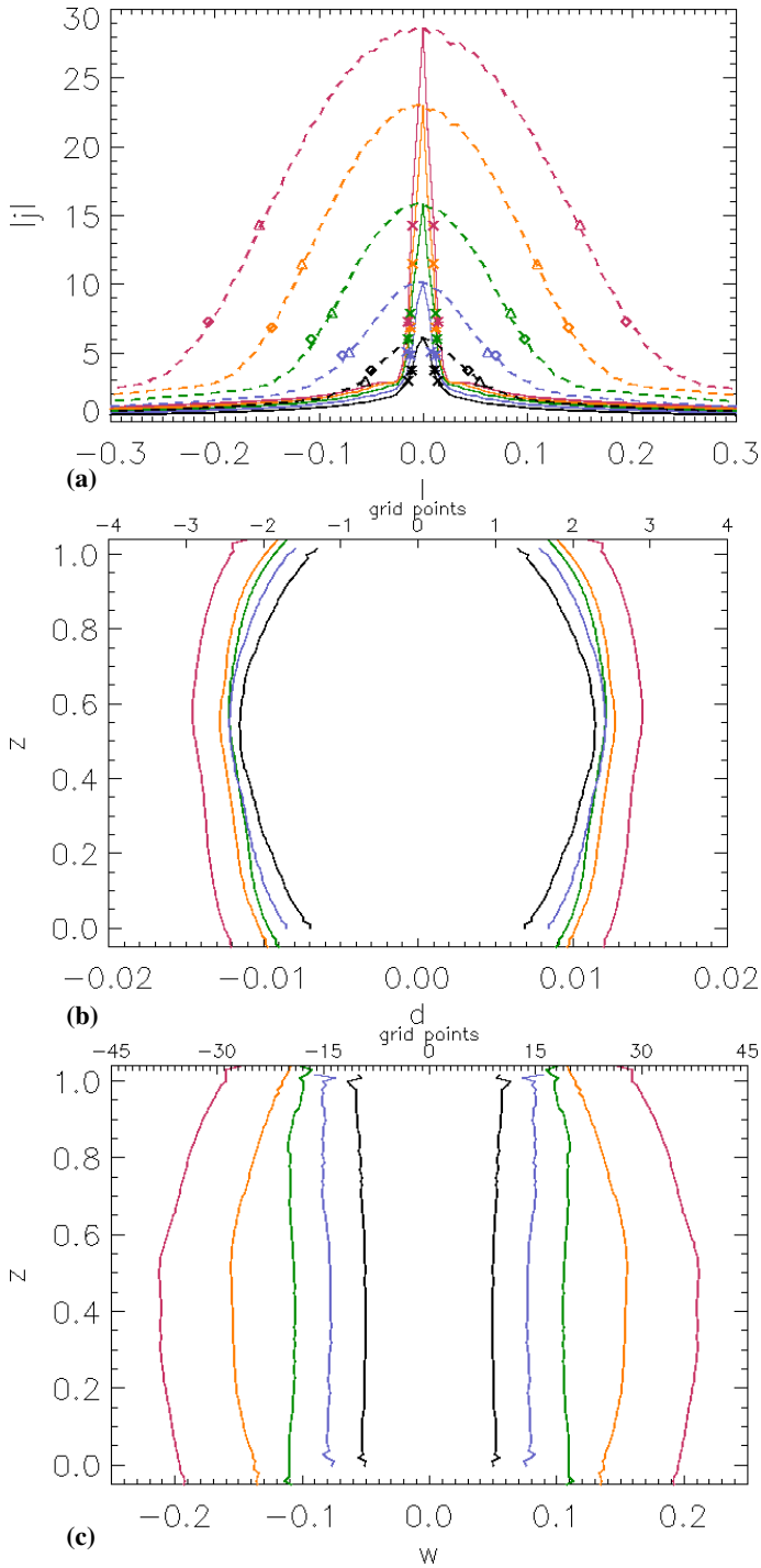
Fig. 10: (a) |j| in a cut through the depth (solid) and across the width (dashed) of the current layer in the plane z = 0.5 with asterisks and diamonds representing the values of the current contour used to determine the depth and the width of the current layer at this cut for the contour method and the crosses and triangles for the FWHM method, respectively. (b) Outline of the depth and (c) width of the current layer. The colours represent initial current j_{sep} = 0.75 (black), 1.00 (blue), 1.25 (green), 1.5 (orange) and 1.75 (red).
