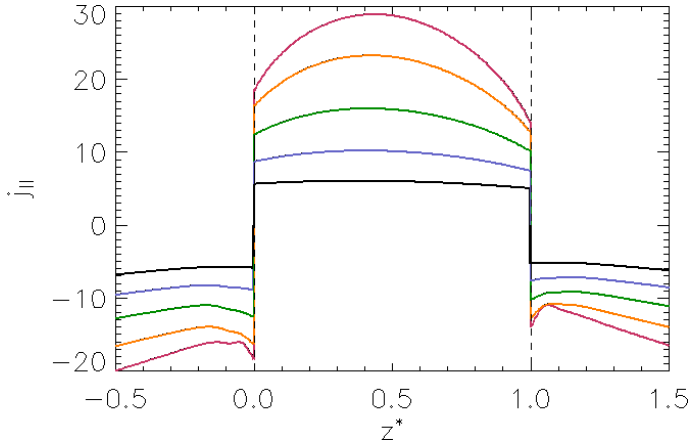
Fig. 9: j_{||} along the z -axis normalised to the length of the respective separator for experiments with initial current j_{sep} = 0.75 (black), 1.00 (blue), 1.25 (green), 1.5 (orange) and 1.75 (red).
