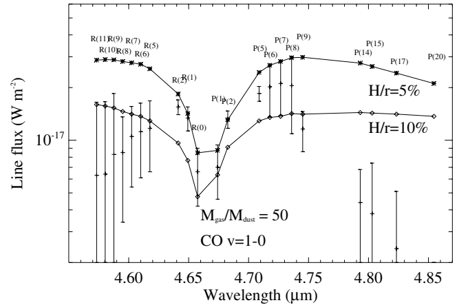
Fig. 16. Some modeled CO fundamental ro-vibrational fluxes compared with the observed fluxes taken from Brittain et al. (2007) . The error bars are 3\sigma uncertainties. The identification of the lines are labelled. The two models have a gas-to-dust-mass ratio of 50. The opening angles are 5% and 10%.
