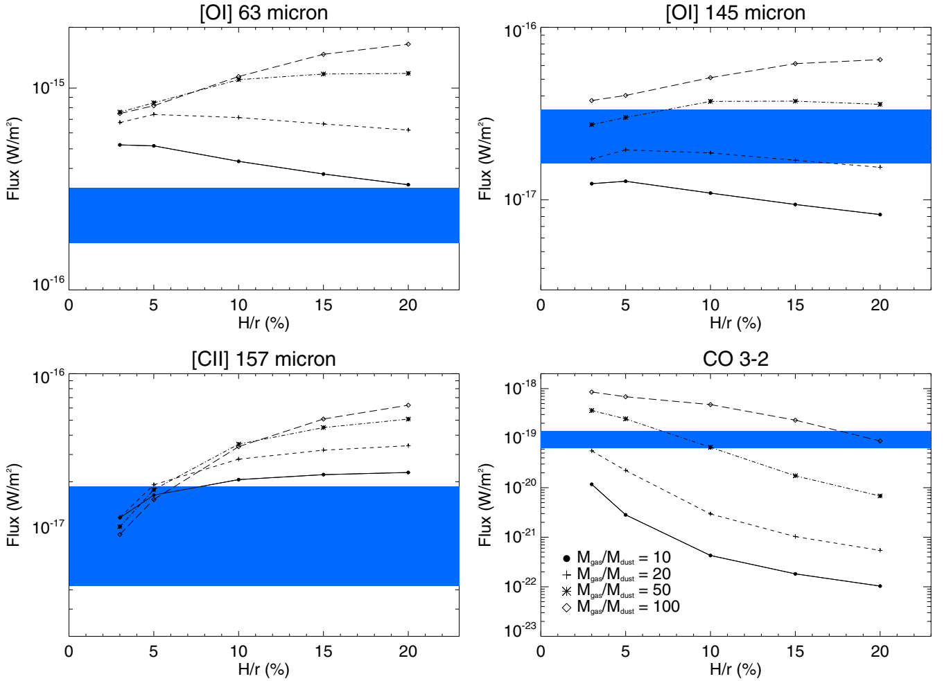
Fig. 12. Predicted [O I] 63 and 145 \mu\text{m} , [C II] 157 \mu\text{m} fine-structure and CO 3–2 fluxes as a function of the gas scale-height parameter for four different gas-to-dust-mass ratio. The observed fluxes are overplotted in blue boxes with the 3\sigma error and 30% calibration error taken into account. No model fits the [O I] 63 \mu\text{m} line.
