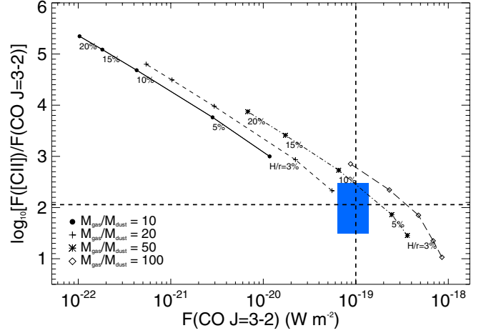
Fig. 15. Observed [C II] / CO J = 3-2 line flux ratios as a function of the CO J = 3-2 line flux for different models with varying opening angles H/r (3%, 5%, 10%, 15%, and 20% as indicated on the plot) and disk gas-to-dust-mass ratios. The blue box encircles the observed ratio and flux, including the uncertainties.
