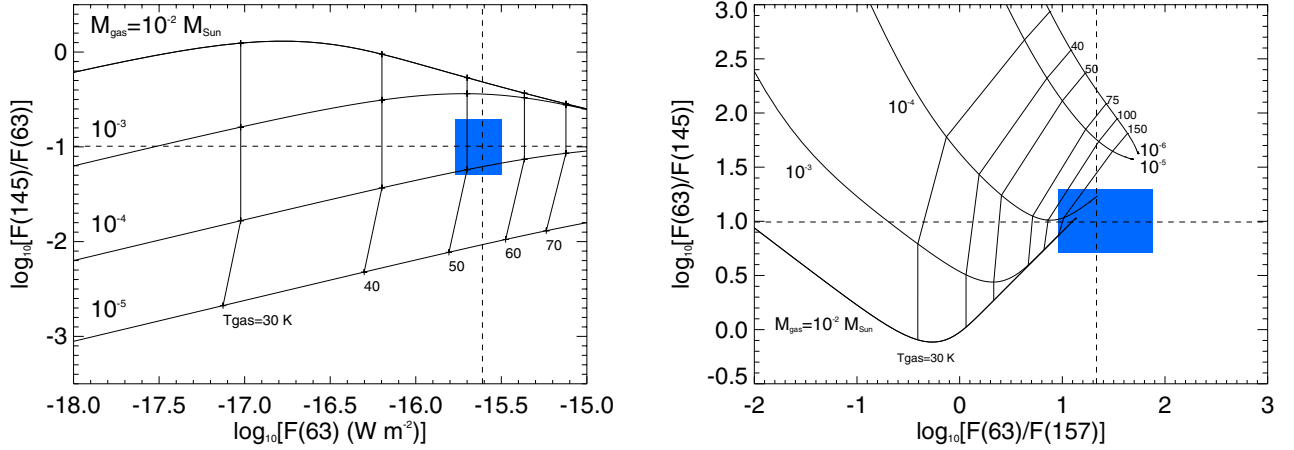
Fig. 3. Oxygen fine-structure line flux ratio as a function of [O I] 63 \mu\text{m} is shown in the left panel. The right panel shows the [O I] 63/[O I] 145 ratio versus the [O I] 63/[C II] 157 ratio. The blue boxes indicate the observed flux ratios. All ratios suggest a gas mass of a few 10^{-4} M_{\odot} and a disk-averaged temperature of 75–150 K.
