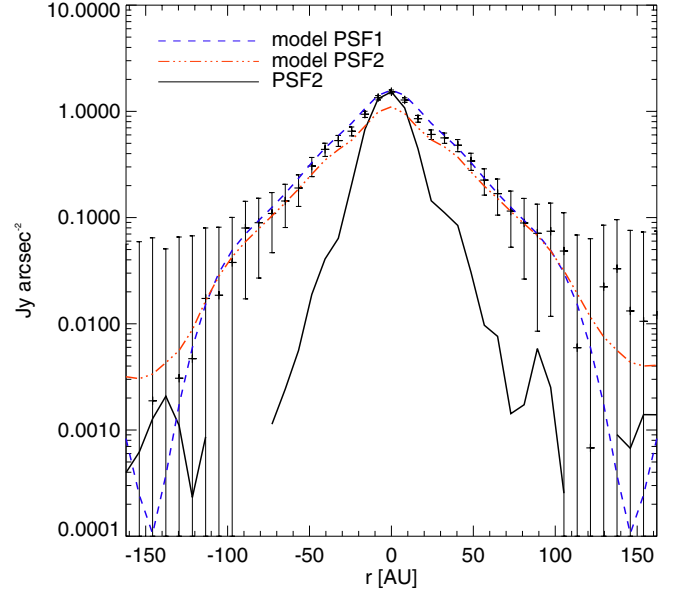
Fig. 8. Fit to the PAH radial emission profile at 8.6 \mu\text{m} along the major axis obtained with VISIR at the VLT. The same model has been convolved with the observed or theoretical noise-free PSF. The theoretical PSF fits the core of the observed function. The model succeeded in fitting the profile.
