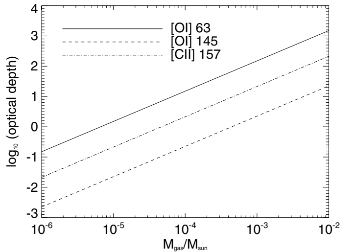
Fig. 4. [O I] 63 and 145 \mu\text{m} and [C II] 157 \mu\text{m} line optical depths as a function of the gas disk mass at T_{\text{gas}} = 60 \text{ K} .
