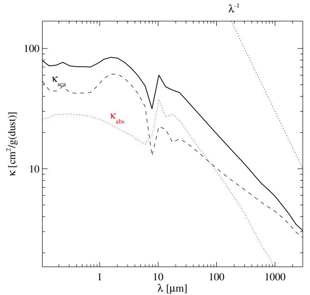
Fig. 5. Dust opacity. The dust grains are made of astronomical silicates.
