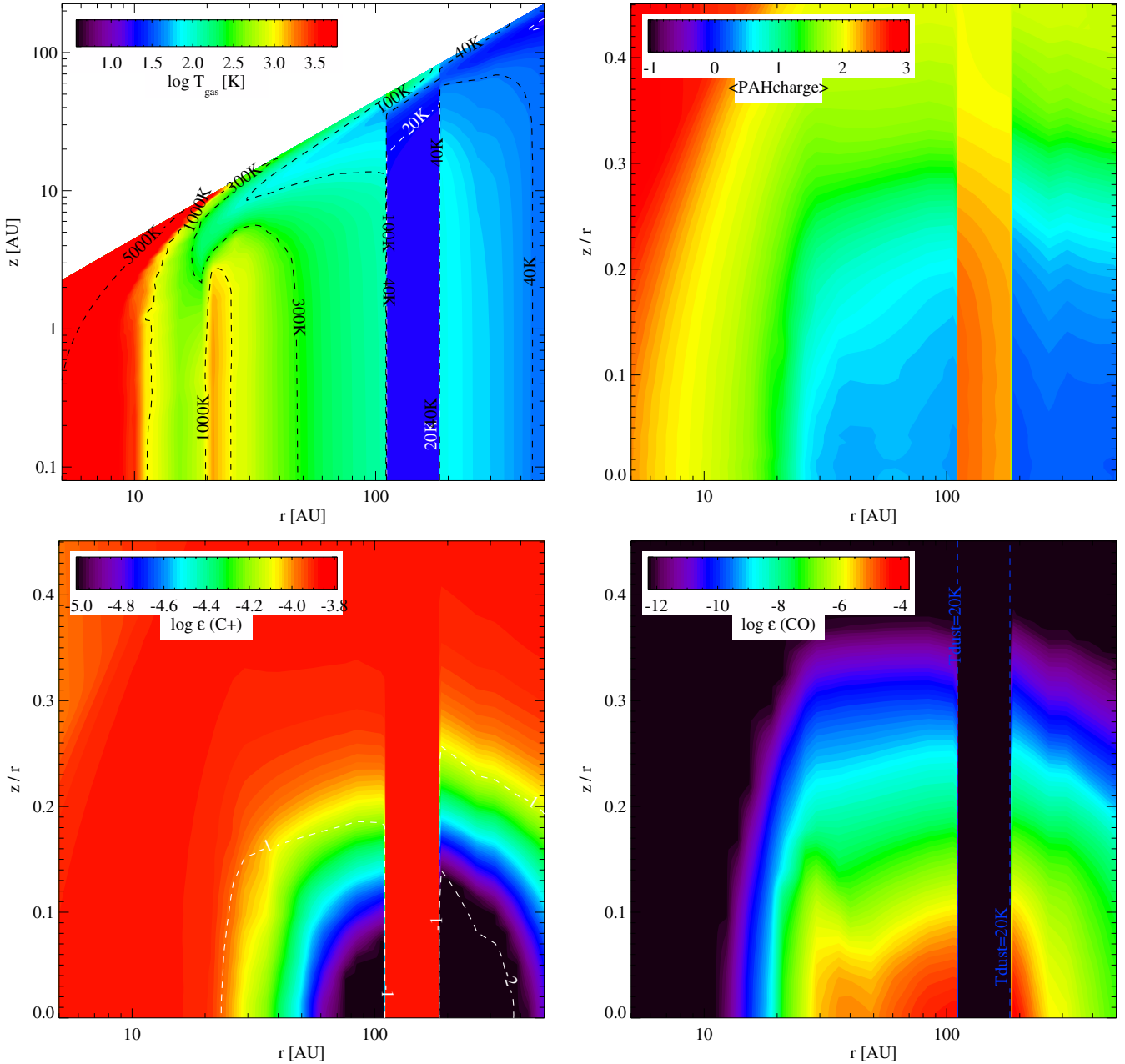
Fig. 10. Gas temperature structure ( upper-left panel ), PAH average charge ( upper-right panel ), C^+ abundance ( lower-left panel ) and the CO abundance ( lower-right panel ) for the model with H_0 = 5\% and a gas-to-dust-mass ratio of 100. The gap between 100 and 185 AU is not empty but is filled with a very low density gas. The computation of the gas temperature in the low gas density gap is not reliable.
