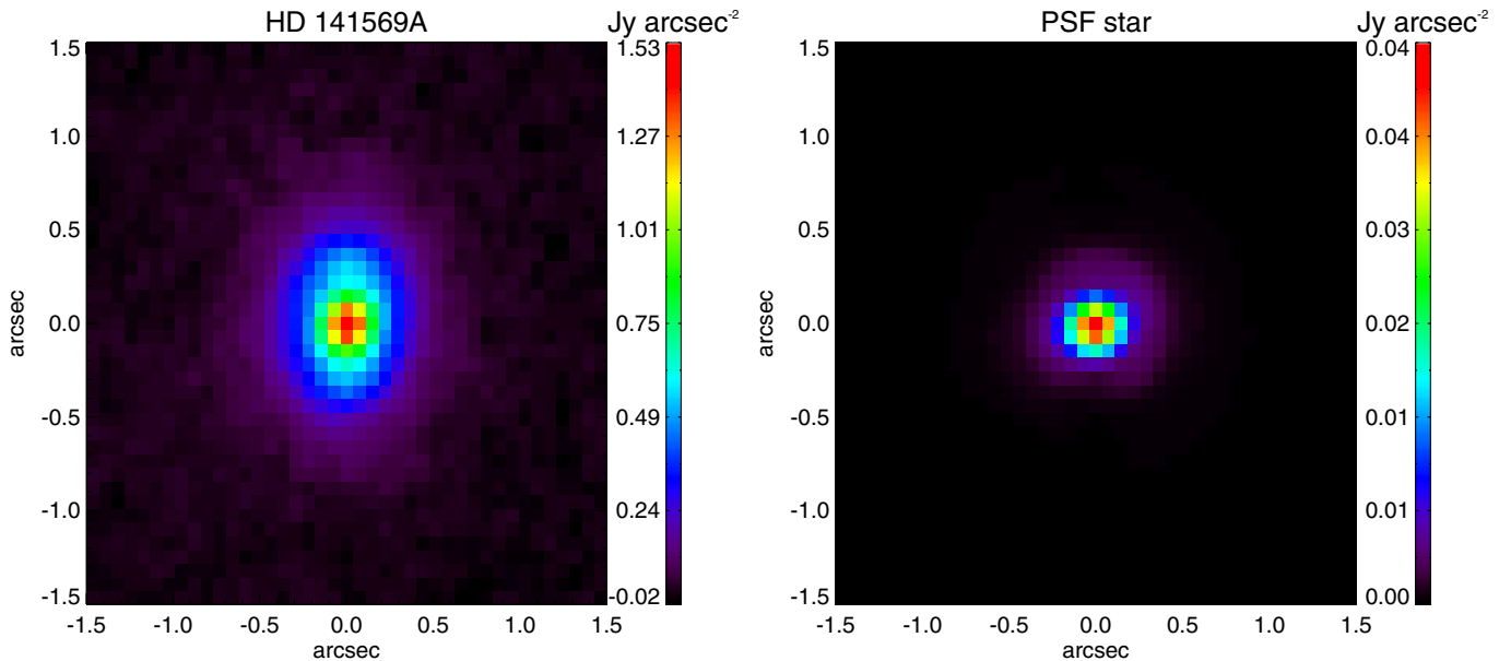
Fig. 7. Observations at the VLT with the VISIR instrument and the 8.6 \mu\text{m} filter (up is North, right is West). The left panel shows the image of HD 141569A and the right panel the PSF star HD 146791. The disk around HD 141569A is well resolved along its major axis in the north-south direction.
