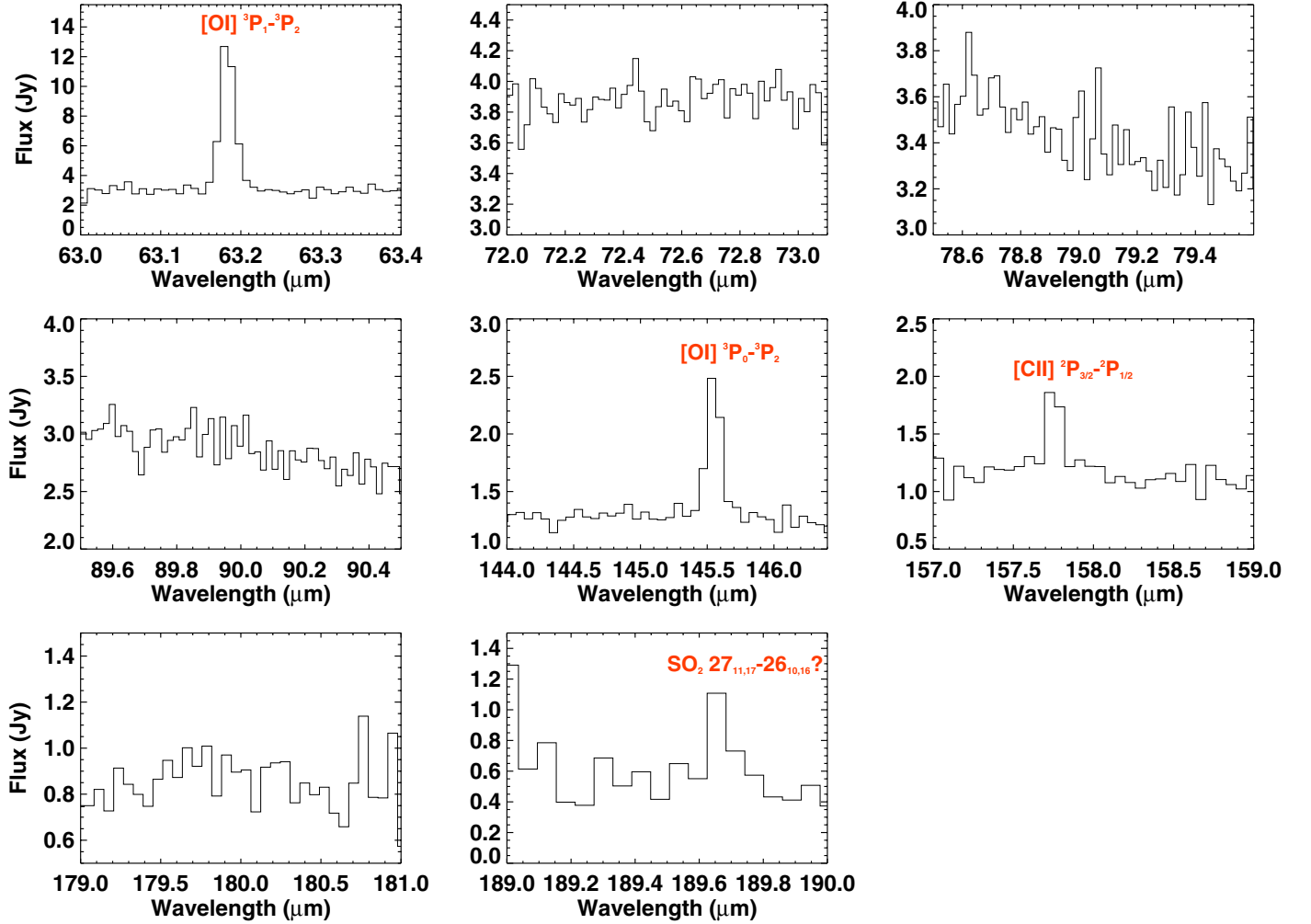
Fig. 1. Herschel spectra toward HD 141569A. The peak at 189.7 \mu\text{m} , which may correspond to a \text{SO}_2 line is most likely an artifact.
