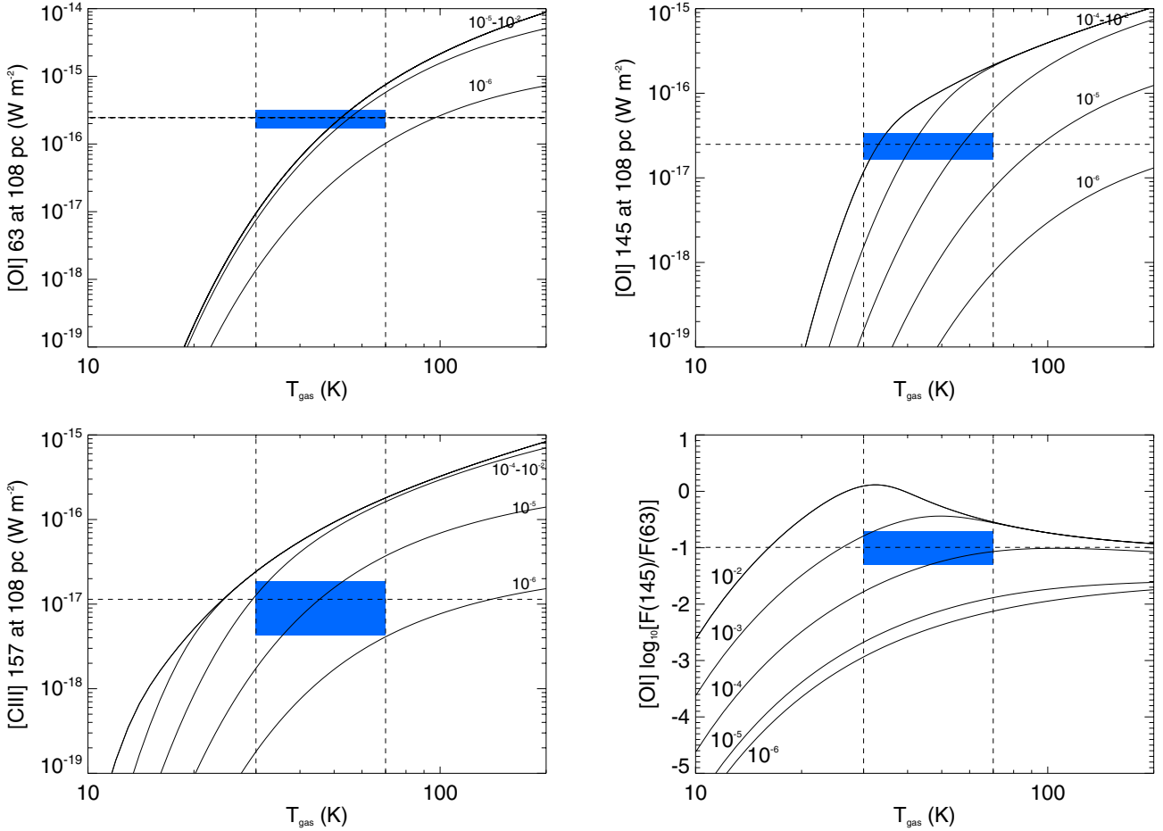
Fig. 2. Predicted [O I] 63 and 145 \mu\text{m} and [C II] 157 \mu\text{m} fine-structure fluxes as a function of the gas temperature. The fourth panel shows the predicted ratio between the [O I] 63 and 145 \mu\text{m} fluxes. The observed ratio is overlotted by the horizontal dashed lines. The total disk gas masses in M_{\odot} are indicated. The blue box encompasses gas temperatures between 30 and 70 K and the observed [O I] at 63 \mu\text{m} , [O I] at 145 \mu\text{m} , [C II] at 157 \mu\text{m} , and the F([\text{O I}]145 \mu\text{m})/F([\text{O I}]63 \mu\text{m}) flux with 3\sigma error bars.
