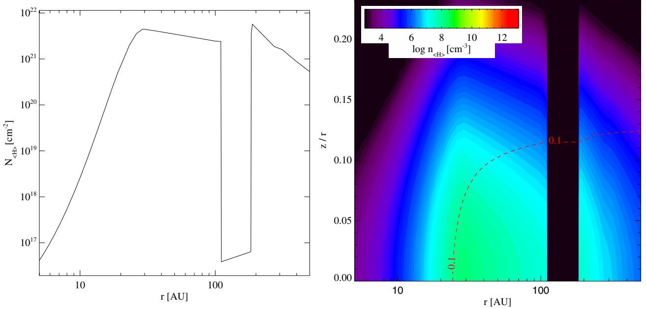
Fig. 6. Adopted half-disk surface density profile ( left panel ) and gas density structure for a H_0 = 5\% opening and a gas-to-dust-mass ratio of 100 disk, i.e. M_{\text{gas}} = 4.9 \times 10^{-4} M_{\odot} ( right panel ). The gap between 110 and 185 AU is not entirely devoid of gas and dust.
