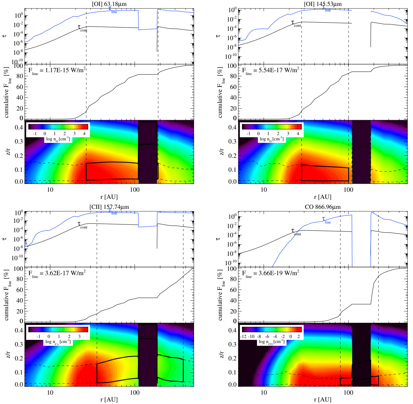
Fig. 11. [OI] emission at 63 \mu\text{m} (upper-left panel), at 145 \mu\text{m} (upper-right panel), C II emission at 157 \mu\text{m} (lower-left panel) and the CO 3–2 emission (lower-right panel) for the model with H_0 = 5\% and a gas-to-dust-mass ratio of 100. The upper part in each panel shows the line center and continuum vertical optical depth as function of the disk radius. The middle part is the cumulative flux as function of the radius. The lower part shows the species volume density in \text{cm}^{-3} . The line fluxes are computed by ray-tracing from the opposite side of the disk toward the observer. The black boxes in the lower panels represent the regions where the vertical cumulative fluxes are at 15% to 85% of the fluxes that are emitted for half a disk. The fluxes are given for a disk seen face-on. For a given disk inclination, optical depth will change the emitted fluxes.
