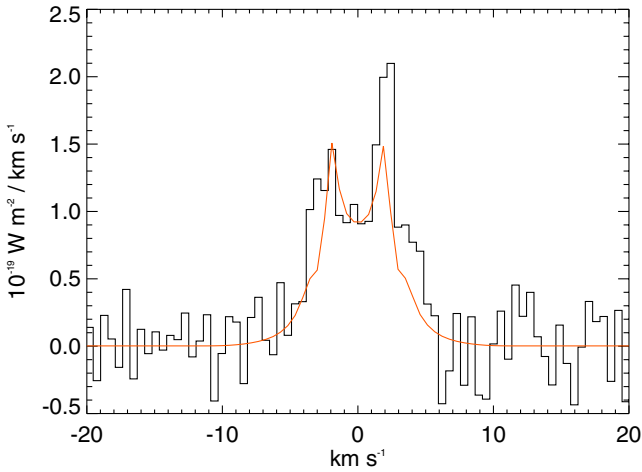
Fig. 14. Observed CO J = 3-2 line profile (histogram black line) compared with the disk model-predicted profile (continuous red line). The model has an opening angle of 5% and a gas-to-dust-mass ratio of 100.
