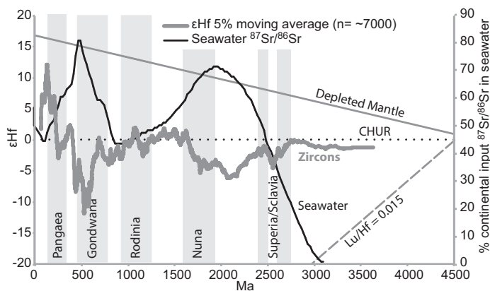
Figure 1. Normalized seawater ^{87}\text{Sr}/^{86}\text{Sr} curve (Shields, 2007) plotted with 5% running average of initial zircon \epsilon Hf (i.e., 5% of total number, n , in database is used for period of running average) from global database of modern and recent river sediments (see Dhuime et al., 2012, for references). Time periods of Grenville and Pan-African orogenic events (Bradley, 2011) are outlined (CHUR—chondrite uniform reservoir).
