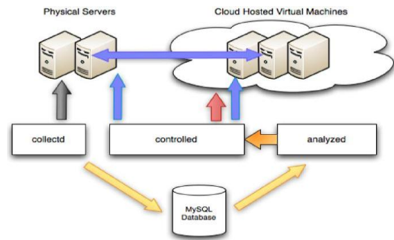
Figure 3: CLAWS: CCloud Aware Virtual World System
