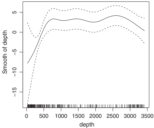
Fig. 4. Plot of the effect on the response of depth, given location (from the model with both depth and location smooths). Note that it is possible to draw a straight line between 750 and 3000 m within the confidence band (between the dashed lines), so the wiggles in the smooth may not be indicative of any relationship. What is clear is that there the estimated number of dolphins increases up to a water depth of about 500 m. The rug ticks at the bottom of the plot indicate we have good coverage of the range of depth values in the survey area. Note that the y axis in such plots is on the scale of the link function (log in this case), so care should be taken in their interpretation.
