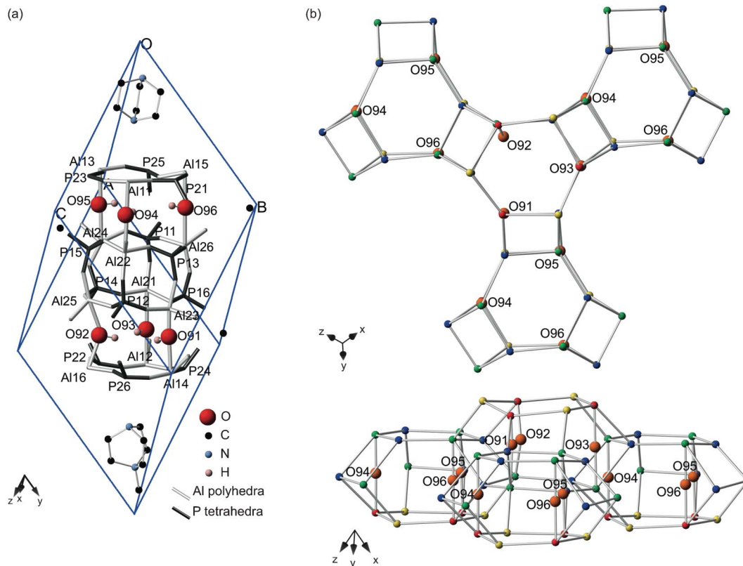
Fig. 4 (a) Unit cell corresponding to dehydrated STA-2(BDAB), showing the distinct Al and P species, and the six possible hydroxyl locations. (b) Part of framework structure of dehydrated STA-2(BDAB), shown as a wireframe model, indicating the proximity of the hydroxyl groups. Atoms in the BDAB template are not shown for clarity.
