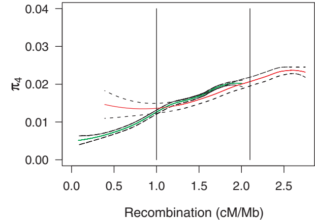
Fig. 2. Effective recombination rate versus 4-fold synonymous diversity ( \pi_4 ) for the autosomes and 4-fold synonymous diversity multiplied by 4/3 ( \pi_4 corrected) for the X chromosome. Bold lines represent Loess regression lines, in green for the autosomal genes and in red for the X chromosome genes. Dashed lines represent the CIs for the lines. The two vertical lines indicate the lower and upper ends of the overlap region.
