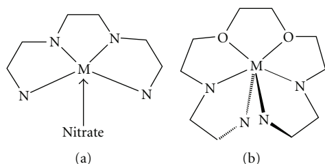
SCHEME 2: A schematic representation of the coordination of the Schiff base ligands used, to lanthanides. (a) References 18–21, (b) This work.
