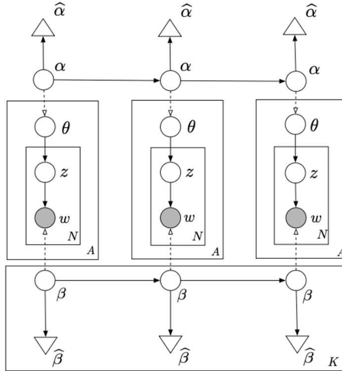
Figure 3: This is a graphical depiction of the variational version of the Dynamic Topic Model across three-time intervals. \theta , z , w , and \mathbf{N} are all the same as in Figure 2. \mathbf{A} is now the number of tweets. \mathbf{K} is number of topics hyperparameter. \alpha is now mean parameter of the logistic normal distribution at each time interval, while \beta is the multinomial distribution parameters for each topic, which are now able to evolve over time. \hat{\alpha} and \hat{\beta} are the variational approximation outputs (Adapted from Blei and Lafferty, 2006, Pgs. 2 – 3) [89].
