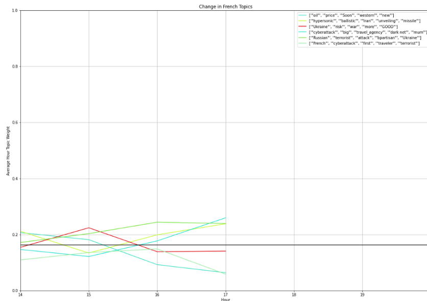
Figure 10: French Topics generated and tracked for June 6 th , 2023, from 14:00 to 17:00 GMT
