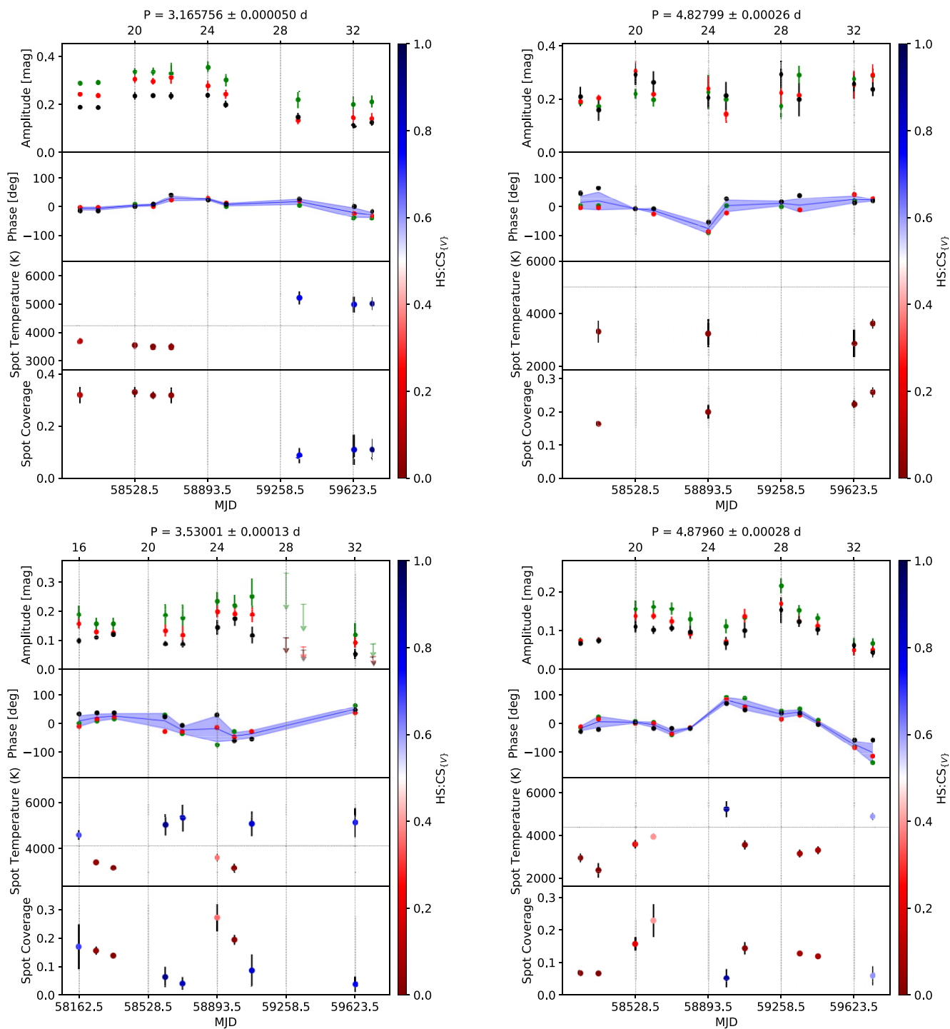
Figure 4. Result summary plots for the first four objects in our sample. The data for object 1 are shown in the top left panel, object 2 in the top right panel, object 3 in the bottom left panel, and object 4 in the bottom right panel. In each of the summary plots we show from top to bottom the peak to peak amplitudes, the maximum brightness phase positions, the determined spot temperatures, and the spot coverage against time. For more details, see the description in Section 5.1.
