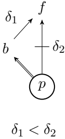
Figure 7.1: The Tweety Triangle. Circled propositions constitute the set of hard background information; the double arrow shows that (p \rightarrow b) is in the background information. A \delta -labeled arrow from one formula \varphi to another \psi means the default \delta = (\varphi \rightsquigarrow \psi) is among the available defaults. When a \delta -labeled arrow from \varphi to \psi is crossed out, it means that \delta = (\varphi \rightsquigarrow \neg\psi) is available. For the order \leq we omit reflexive loops and links obtainable by transitive closure to ease readability.
