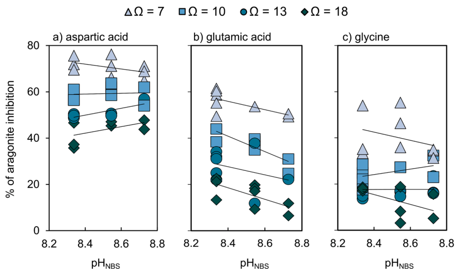
Fig. 6. Inhibition of aragonite precipitation by the addition of 2 mM a) aspartic acid, b) glutamic acid, and c) glycine as a function of pH and \Omega_{Ar} . Uncertainty in pH is <0.004 pH units (smaller than the symbols used). Multiple precipitations are shown under each set of conditions to indicate uncertainty in inhibition of precipitation rate.
