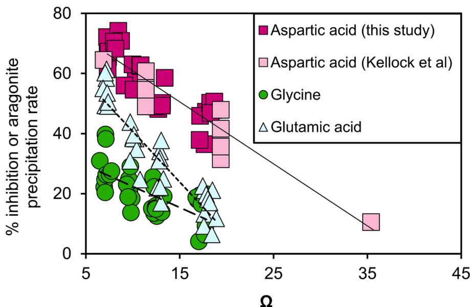
Fig. 5. Inhibition of aragonite precipitation rates by amino acids (2 mM) as a function of \Omega_{Ar} . We include the data from Kellock et al., (2020) which also measured inhibition of aragonite precipitation by 2 mM aspartic acid. Uncertainty in \Omega is smaller than the symbols used (see legend to Fig. 2) and multiple precipitations are shown under each set of conditions to indicate uncertainty in inhibition of precipitation rate.
