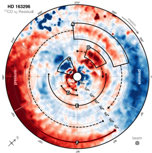
Figure 2. A zoom-in of Figure 1(c). A representative beam size is shown in the lower right; however, due to the elevated emission surface, the true angular resolution varies across the map. The figure extends out to 4''.4 , and the color scaling ranges between residuals of \pm 180 \text{ m s}^{-1} . Residuals due to the pressure gradient slowing the rotation of the disk are observed along the major axis, marked as “pressure.” Three regions of large velocity deviations are marked by black boxes, centered at (r, \phi) = (2''.85, 305^\circ) (A), (1''.65, 315^\circ) (B), and (0''.9, 220^\circ) (C), all of which have extended structure shown by the dashed lines. The outer feature, A, is associated with the planet identified by Pinte et al. (2018b), while the inner two, B and C, are likely associated with the potential “kink” reported by Pinte et al. (2020), or due to the asymmetry in the continuum emission (Isella et al. 2018). Two arc-like structures are also seen at radii of 1''.15 (116 au), and 1''.8 (182 au), shown by the solid lines, labeled D and E, respectively, in addition to a larger arc feature at 4''.1 (414 au), shown by the thick solid line with a faded end, annotated as F. It is unclear where this outermost arc ends, as the perturbation extends into a region dominated by pressure-modulated deviations.
