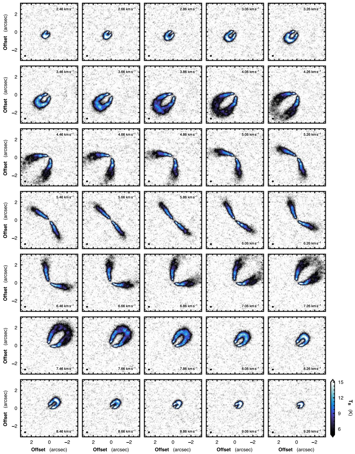
Figure 18. Same as Figure 16, but for C^{18}O J=2-1 emission.
