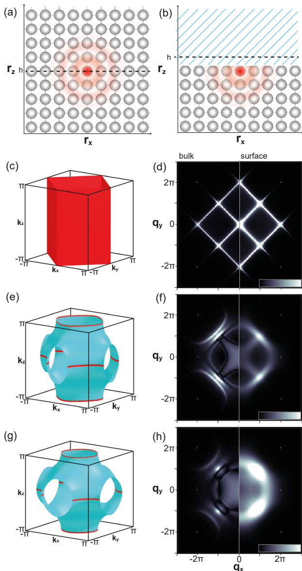
FIG. 1. Consequence of out of plane hopping on the bulk and surface QPI patterns. (a, b) Sketch of the two scenarios considered, (a) a defect situated in the bulk of a material, (b) a defect at the surface of a material. Here h refers to the 2D plane used to study the Fourier transformation of the local density of states. (c, d) 3D Fermi surface and cQPI \tilde{\rho}(\mathbf{q}_{\parallel}, \omega) at r_z = h , calculated for the bulk defect (left half) and surface defect (right half) for the nearest neighbour cubic model with t_x = t_y = 0.1 and t_z = 0 . (e, f) Equivalent simulations for t_z = 0.05 , (g, h) t_z = 0.1 (isotropic case). The surface projected spectral functions are plotted in Fig. S2 in ref. 25.
