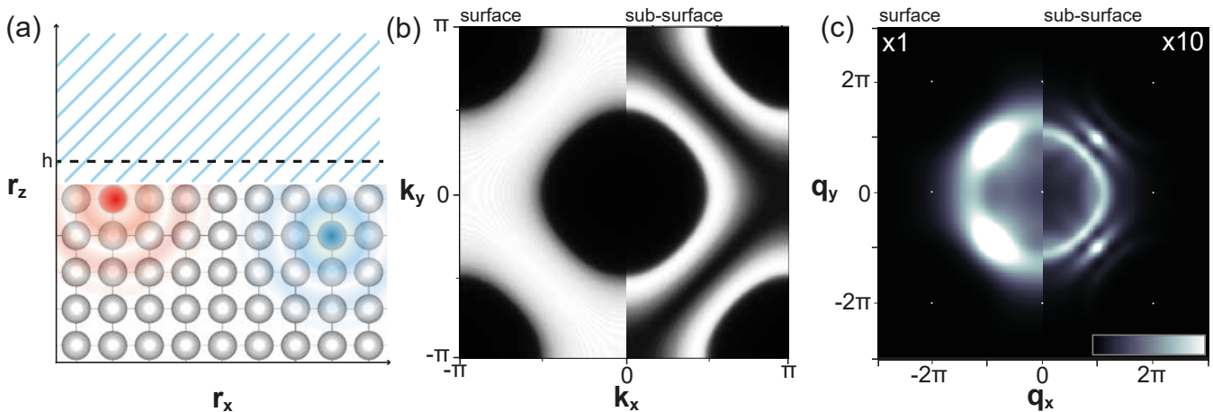
FIG. 2. Consequence of defect position for measured QPI. (a) Sketch of defects at different positions from the surface. (b) Partial spectral function of the surface layer (left half) and sub-surface layer (right half). (c) cQPI \tilde{\rho}(\mathbf{q}_{\parallel}, \omega) for a defect located at the surface (left half, red atom in (a)) and sub-surface (right half, blue atom in (a)). The intensity of the simulated cQPI due to a sub-surface defect has been enhanced by a factor of 10 for comparison with the surface cQPI pattern.
