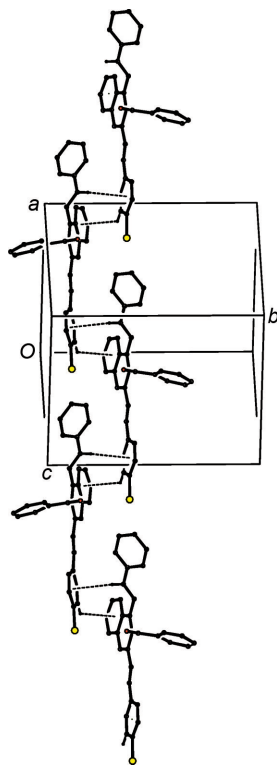
Figure 9 Part of the crystal structure of compound (IIc), showing the formation of a chain of rings running parallel to the [10\bar{1}] direction and built from two independent C-H\cdots\pi(\text{arene}) hydrogen bonds, which are drawn as dashed lines. For the sake of clarity, H atoms which are not involved in the motif shown have been omitted.
