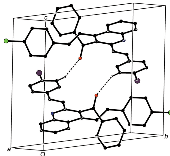
Figure 10 Part of the crystal structure of compound (IIId), showing the formation of a cyclic R_2^2(20) dimer built from C-H\cdots O hydrogen bonds, which are drawn as dashed lines. For the sake of clarity, H atoms which are not involved in the motif shown have been omitted.
