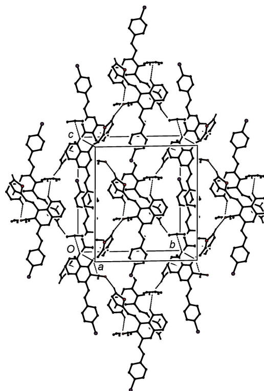
Figure 11 Part of the crystal structure of compound (IIe), showing the formation of a sheet lying parallel to \{100\} and built from a combination of C-H\cdots O and C-H\cdots\pi(\text{arene}) hydrogen bonds, which are drawn as dashed lines. For the sake of clarity, the minor-disorder component and H atoms which are not involved in the motif shown have been omitted.
