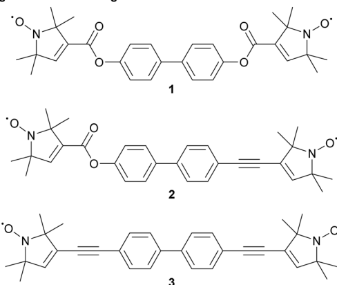
a) Rigid bis-nitroxide targets:
