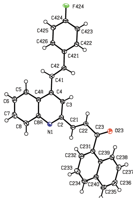
Figure 2 The molecular structure of compound (IVb), showing the atom-labelling scheme. Displacement ellipsoids are drawn at the 50% probability level.
