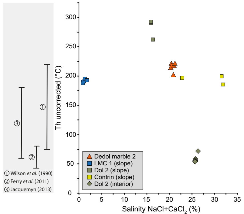
Fig. 8. Fluid inclusion salinity versus homogenization temperature ( T_h ) uncorrected plot for phase-specific fluid inclusions from the contact aureole, Latemar slope and interior. Dolomitization temperature ranges from former studies: ① dolomite fluid inclusion homogenization temperatures by Wilson et al. (1990); ② clumped isotope temperatures by Ferry et al. (2011); and ③ dolomite fluid inclusion homogenization temperatures by Jacquemyn (2013).
