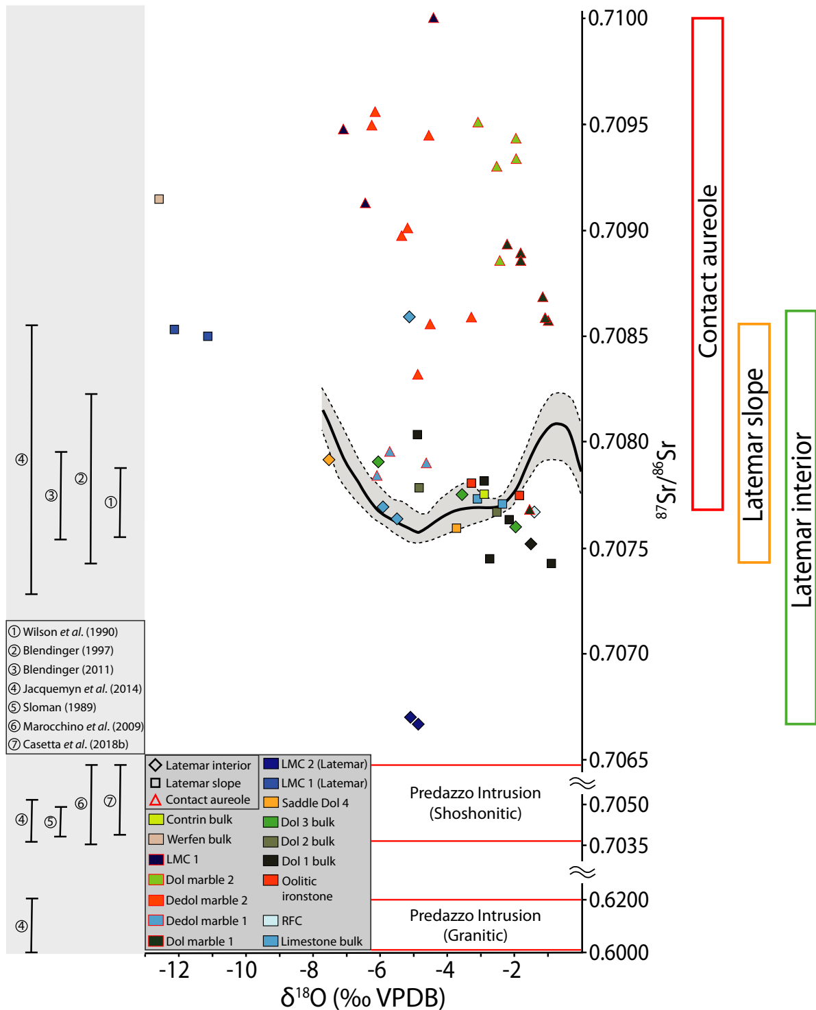
Fig. 15. Oxygen-isotope composition versus strontium-isotope ratios of dolomite and calcite phases compared to Middle/Late Triassic unaltered marine calcites from Korte et al. (2003) and ranges of former studies by Wilson et al. (1990), Blendinger (1997), Blendinger et al. (2011) and Jacquemyn et al. (2014). Except for some calcites and less radiogenic dolomites (0.7074), all Latemar samples fit in the Middle/Late Triassic range and agree with former studies. Some marbles from the contact aureole display Triassic values, while the majority are more radiogenic (up to 0.7100). This trend is counterintuitive as the intrusion displays values from 0.7036 to 0.7064 (shoshonitic units, Sloman, 1989; Marrocchino et al. , 2009; Jacquemyn et al. , 2014; Casetta et al. , 2018b) and 0.6000 to 0.6200 (Jacquemyn et al. , 2014). No marbles were analyzed at the Latemar slope/interior.
