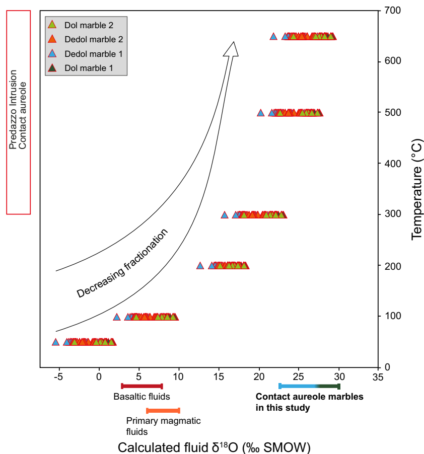
Fig. 14. Cross-plot of the isotopic composition ( \delta^{18}\text{O}_{\text{VSMOW}} ) of the formation fluid calculated from \delta^{18}\text{O}_{\text{VPDB}} values of the investigated marbles from the Predazzo Intrusion contact aureole by considering oxygen isotope equilibration based on Sheppard & Schwarcz (1970) and Friedman & O'Neil (1977) for dolomite and calcite, respectively. The distinct formation temperature ranges (50°C, 100°C, 200°C, 300°C, 500°C and 650°C) are exemplary for the metamorphic temperature range at the Predazzo Intrusion contact aureole obtained from Ferry et al. (2002) and potential late retrograde diagenesis. Note that the oxygen isotope fractionation between both dolomite and calcite, and the fluid is reduced at elevated temperature, thus at 600°C, the \delta^{18}\text{O}_{\text{carbonate-H}_2\text{O}} value is only about +1‰. The oxygen isotope composition of basaltic fluids and primary magmatic \text{H}_2\text{O} is derived from Harmon & Hoefs (1995), Giggenbach (1992) and Vho et al. (2019). The isotopic composition of contact aureole marbles is indicated below the x-axis in green (Dol marbles) and blue (Dedol marbles).
