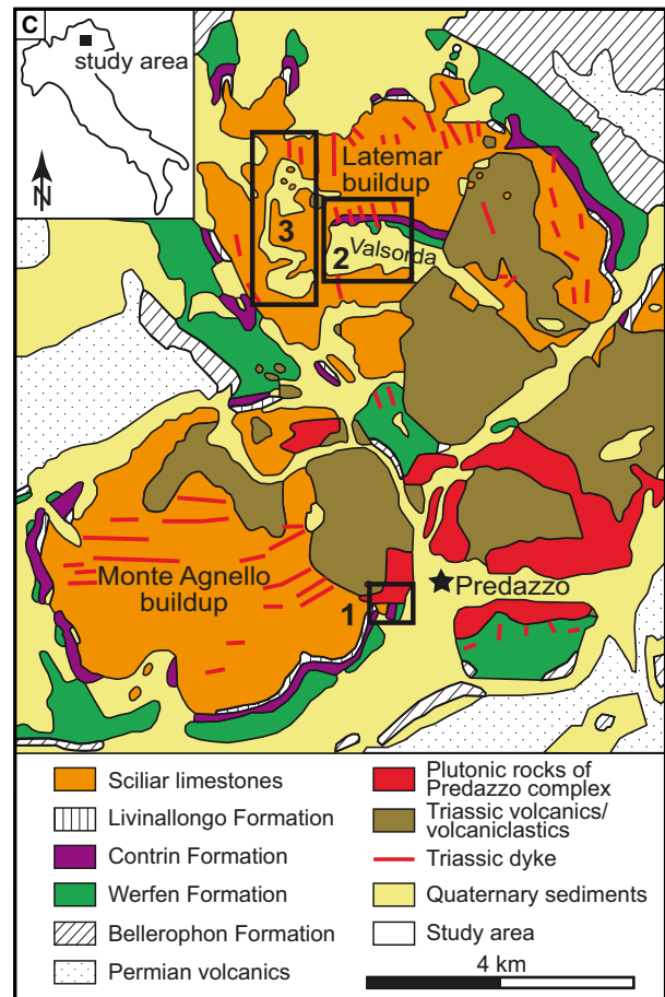
Fig. 1. Regional geological framework of the study area. (A) Map of the Dolomite Mountains in the south-eastern Alps (modified from Hardebol et al. , 2015). (B) A cross-section in the south-eastern Alps including the Dolomites based on Doglioni (1987) and modified from Hardebol et al. , 2015. (C) Distribution of sedimentary and igneous rocks covering the Latemar and Monte Agnello carbonate buildups near Predazzo in northern Italy. The study areas are marked by black boxes: 1 = contact aureole; 2 = Latemar slope; 3 = Latemar interior. Modified from Carmichael et al. (2008).
