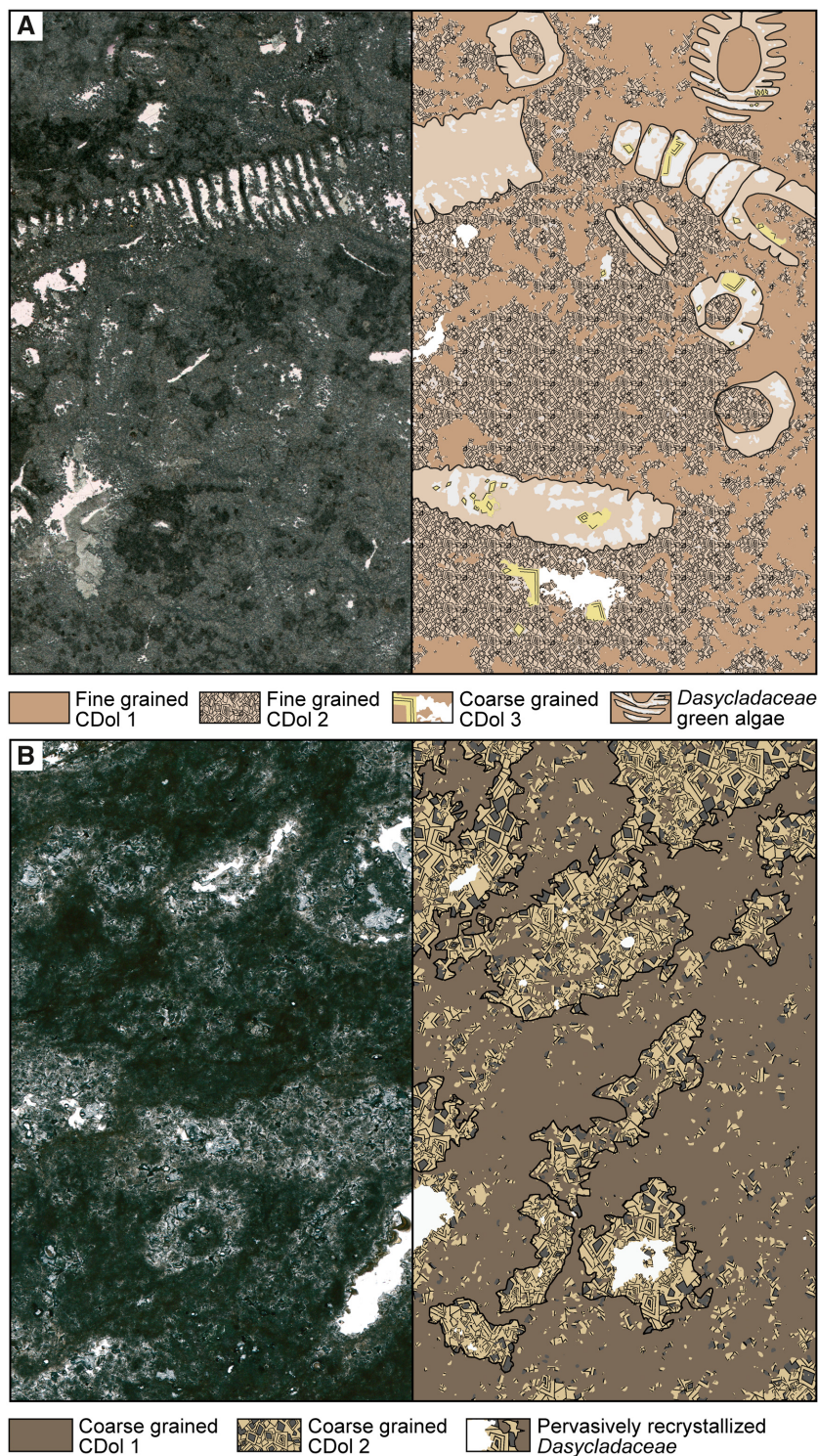
Fig. 16. Two examples of preservation in Contrin Formation dolostone. Transmitted light images (left) placed against redrawn features (right). The field of view is 2.5 \times 2.5 cm. (A) Fabric preserving dolomitization. Fine-grained, early diagenetic dolostone with well-preserved Dasycladacean algae and pore-filling (saddle) dolomite cement. (B) Fabric destructive dolomitization. Medium-grained to coarse-grained, largely recrystallized Contrin dolostone from the Latemar slope with poorly preserved Dasycladacean algae.
