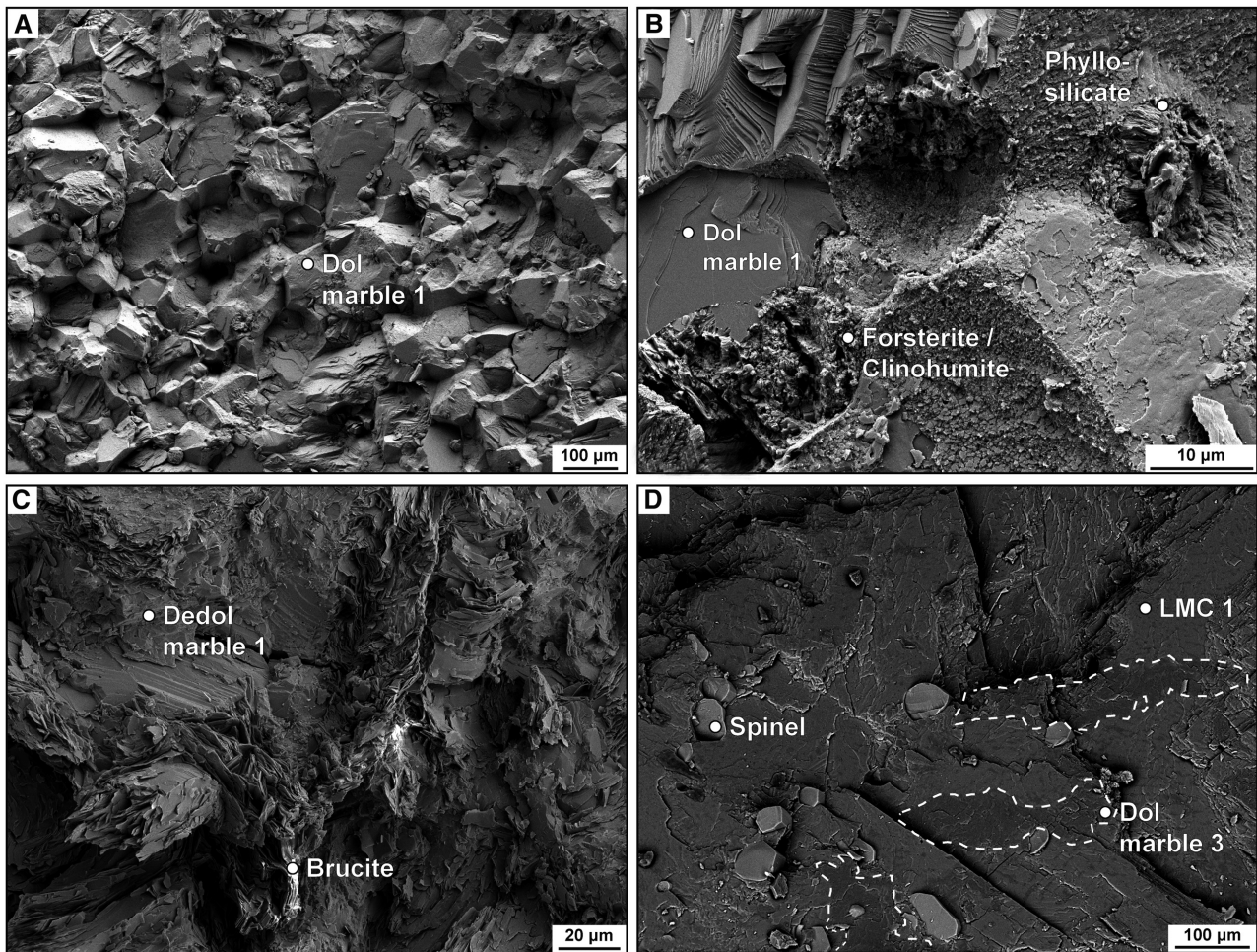
Fig. 6. Scanning electron microscope images from the Contrin Formation at the contact metamorphic aureole of the Predazzo Intrusion. (A) Dol marble 1 matrix with spherical-shaped magnesium silicates. (B) Close-up of (A). Note the spherical forsterite grains which are in transition to clinohumite. (C) Dedol marble 1 fabric with brucite. Note platy crystal habitus of brucite. (D) LMC 1 vein with elongated Dol marble 3 grains and spinel crystals.
