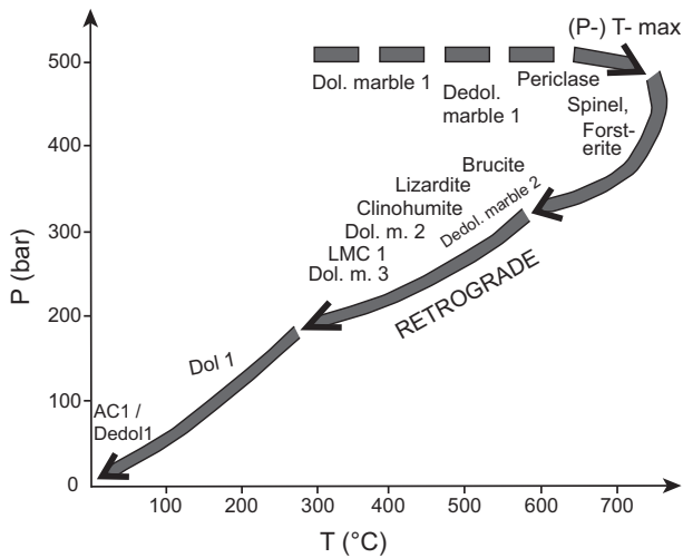
Fig. 11. Metamorphic pathway for contact metamorphosed Contrin Formation dolostones at Canzoccoli quarry. Pressure and temperature data from Ferry et al. (2002).
