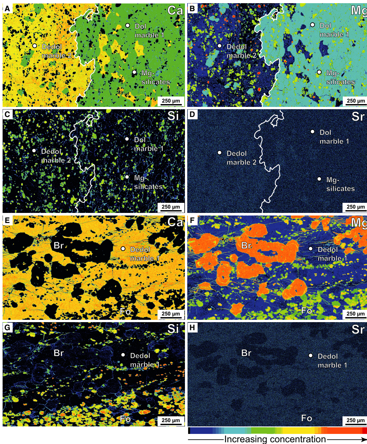
Fig. 5. Microprobe element maps of the contact metamorphosed Contrin Formation near the Predazzo Intrusion. (A) to (D) Sharp contact from dolomite marble 1 (right) to dedolomite marble 2 (left). Note the generally low strontium content that is mainly accumulated in calcitic Dedol marble 2. (E) to (H) Dedol marble 1 containing about 30 vol.% brucite. Note magnesium mobilization along grain boundaries and tiny fissures. The strontium content is generally low and mainly accumulated in calcitic Dedol marble 1. Br, brucite; Fo, forsterite. (A) and (E) Calcium map. (B) and (F) Magnesium map. (C) and (G) Silicon map. (D) and (H) Strontium map.
