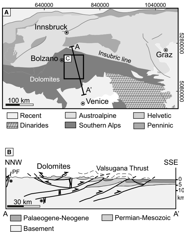
Fig. 1. Regional geological framework of the study area. (A) Map of the Dolomite Mountains in the south-eastern Alps (modified from Hardebol et al. , 2015). (B) A cross-section in the south-eastern Alps including the Dolomites based on Doglioni (1987) and modified from Hardebol et al. , 2015. (C) Distribution of sedimentary and igneous rocks covering the Latemar and Monte Agnello carbonate buildups near Predazzo in northern Italy. The study areas are marked by black boxes: 1 = contact aureole; 2 = Latemar slope; 3 = Latemar interior. Modified from Carmichael et al. (2008).
