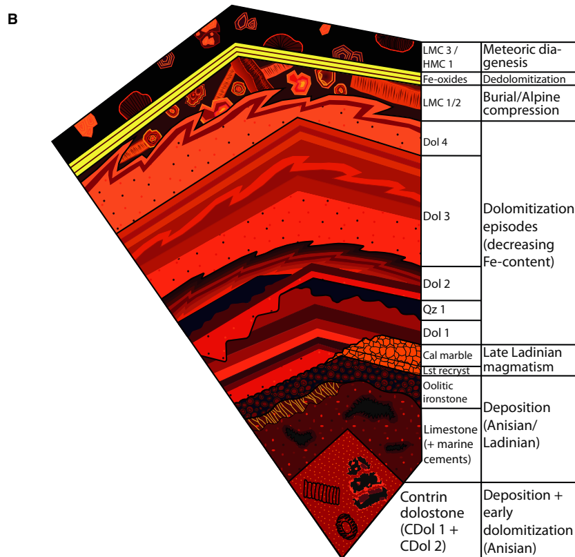
Fig. 10. Complete successions of metamorphic and diagenetic phases with typical cathodoluminescence colours related to their diagenetic and tectonic environment of precipitation or formation. (A) Contact metamorphic succession of the Contrin Formation dolostones. Non-luminescent phases are marked in black. (B) The paragenetic succession of the Sciliar Limestones. The remaining pore space is marked in black.
