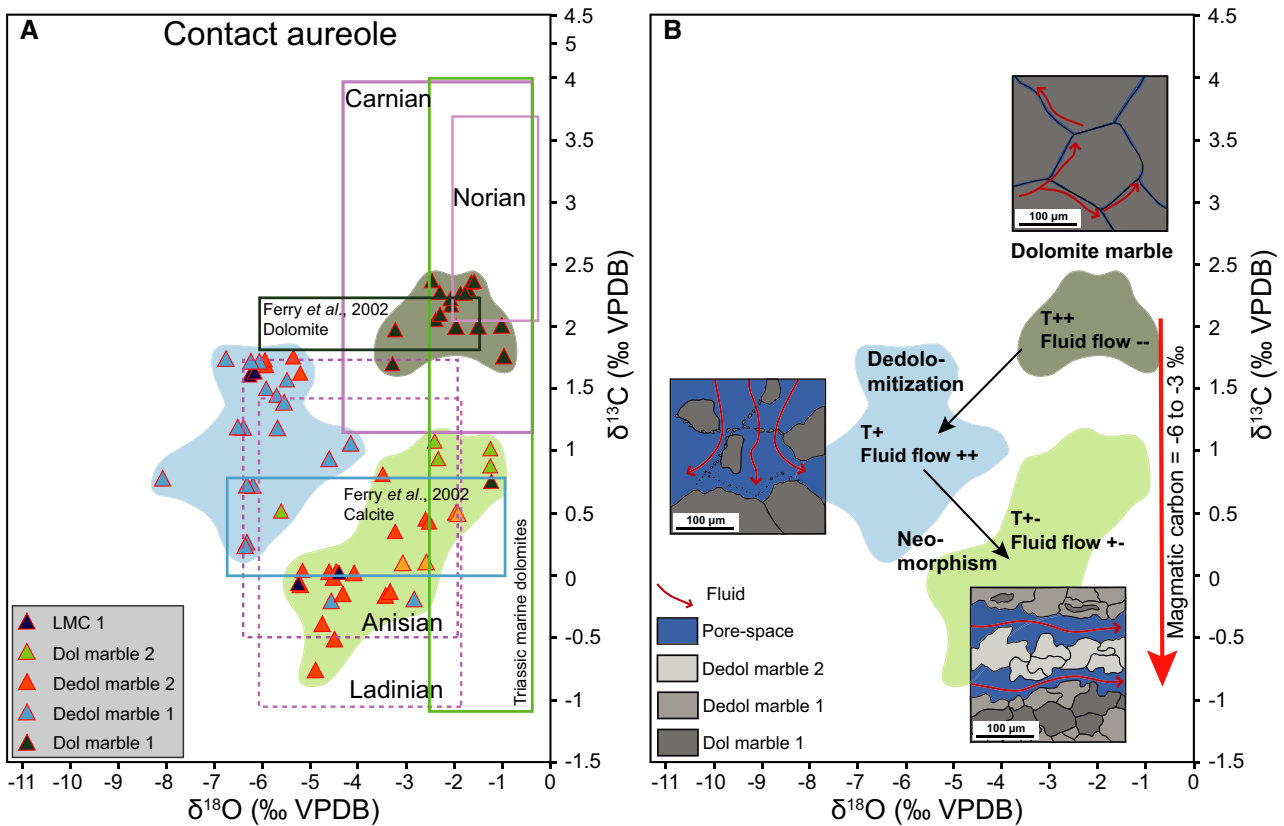
Fig. 13. Cross-plot of \delta^{18}\text{O} and \delta^{13}\text{C} data for dolomite and calcite phases from the contact aureole. (A) The isotopic composition of Middle/Late Triassic marine calcite is indicated in the solid purple and dashed purple boxes (from Korte et al. , 2005; Grossman, 2012; Saltzman & Thomas, 2012; Veizer & Prokoph, 2015). The range of seawater associated with early diagenetic Middle/Late Triassic dolostones is indicated in the light green box (from Geske et al. , 2012; Chatalov, 2018; Rieder et al. , 2019). Data from previous studies (intrusion: Ferry et al. , 2002; Latemar: Jacquemyn et al. , 2014) is marked in dark green (dolomite) and blue (calcite) boxes. The annotated trends indicate a shift in \delta^{13}\text{C} of about -2\text{‰} from Dol marble 1 towards Dedol marble 2. (B) Data from (A) is set in the context of available pore space, mineralogical processes, metamorphic temperatures and fluid flow.
