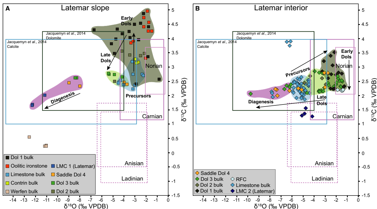
Fig. 17. Cross-plots of \delta^{18}\text{O} and \delta^{13}\text{C} data for all analyzed dolomite and calcite phases from (A) Latemar slope and (B) Latemar interior. The isotopic composition of Middle/Late Triassic marine calcite is indicated by the solid purple and dashed purple boxes (from Korte et al. , 2005; Grossman, 2012; Saltzman & Thomas, 2012; Veizer & Prokoph, 2015). Data from Jacquemyn et al. (2014) is marked in dark green (dolomite) and blue (calcite) boxes. The annotated trends indicate a shift in \delta^{13}\text{C} of about -2\text{‰} from Dol 1 towards Dol 3 and 4 in (A) and a shift in \delta^{13}\text{C} of about -1\text{‰} from Dol 1 towards Dol 3 and 4 in (B).
