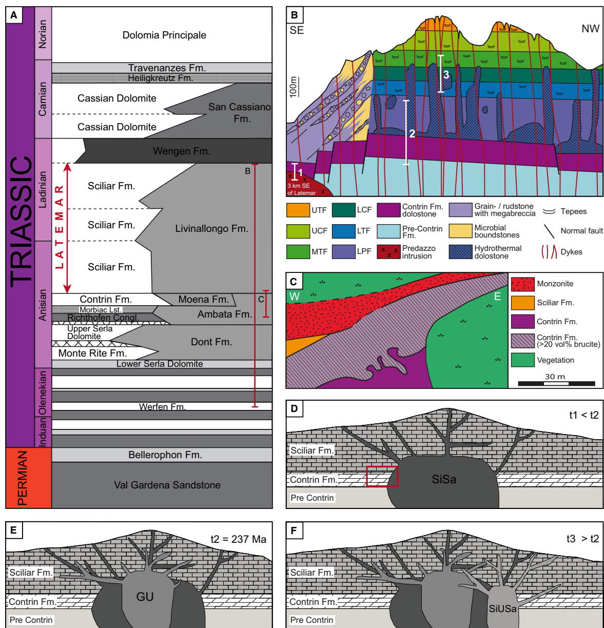
Fig. 2. (A) Stratigraphic chart of the Dolomite Mountains, including ranges for study areas 'B' and 'C' (modified from Jacquemyn, 2013; Jacquemyn et al. , 2014). See Fig. 1 for study area locations. (B) Dyke-perpendicular cross-section across the Latemar buildup including relation to the Predazzo Intrusion, located about 2 to 3 km south-east. The south-east Latemar slope is excluded from this area. UTF, Upper Tepee Facies; UCF, Upper Cyclic Facies; MTF, Middle Tepee Facies; LCF, Lower Cyclic Facies; LTF, Lower Tepee Facies; LPF, Lower Platform Facies. Array 1 (white line) covers the metamorphosed Contrin Formation at the Predazzo Intrusion contact aureole. Array 2 covers the Latemar slope, which consists of Lower Platform Facies and Contrin Formation. Array 3 covers the partly dolomitized Latemar interior, which consists of Lower Cyclic Facies, Lower Tepee Facies and the upper part of the Lower Platform Facies. Modified from Preto et al. (2011) and Jacquemyn (2013). (C) Geological schematic of Canzoccoli quarry at the contact with the Predazzo Intrusion. Modified from Ferry et al. (2002). (D) to (F) Conceptual schematics of the Predazzo Intrusion petrological evolution modified from Casetta et al. (2018a). (D) The first intrusive pulse consists of shoshonitic silica saturated rocks. The position of the Canzoccoli quarry at the contact aureole is marked with a red rectangle. (E) The second pulse is represented by the intrusion of a granitic/syenogranitic unit that was dated as t_2 = 237 Ma by Mundil et al. (1996). (F) The final pulse crops out in the eastern part of the complex and consists of shoshonitic silica undersaturated rocks. Note: The Predazzo Intrusion does not sit directly below the Latemar mountain. Sciliar Formation carbonates in (D) to (F) comprise the hardly accessible and largely eroded direct vicinity of the intrusion. See text for SiSa, GU and SiUSa.
