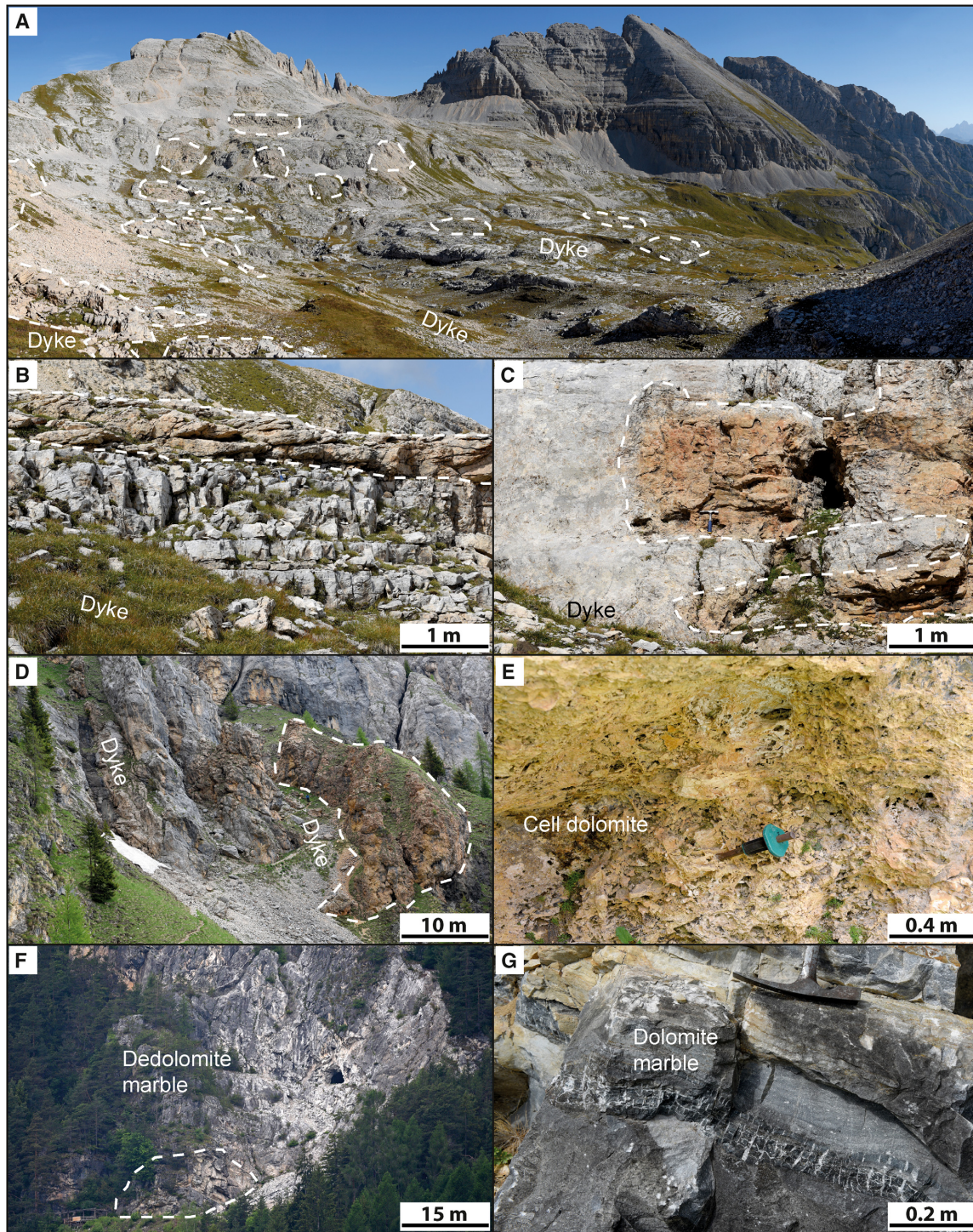
Fig. 3. Overview of dolostone occurrences at the Latemar isolated platform (A) to (E) and the contact with the Predazzo Intrusion (F) to (G). Dolostone occurrences are marked by dashed lines. (A) to (C) Latemar interior (array 3 in Fig. 2B). Hydrothermal dolostones occur as patches with sharp contacts to host limestone and dykes (A). The width in the centre is about 500 m. Hydrothermal dolostones often occur as facies bound (B) or as isolated bodies with sharp and often brittle centimetre to decimetre thick transition zones (C). (D) and (E) Latemar slope (array 2 in Fig. 2B). (D) Dolostone body morphologies appear similar to the Latemar interior but contain different dolomite cements such as cell dolomite displayed in (E). (F) and (G) Contact metamorphosed Contrin Formation dolostones at the Predazzo Intrusion (array 1 in Fig. 2B) were largely dedolomitized (F), but some dolomite marble (G) with visible later metamorphic and tectonic overprint was preserved. Dolostone – dolomite marble in (F) – bodies are indicated by dashed lines.
