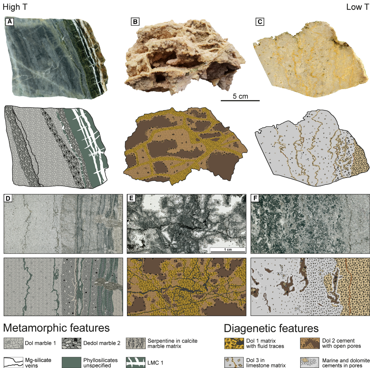
Fig. 12. A sequence illustrating decreasing temperature with increasing distance to the Predazzo Intrusion and displaying rock types representing the three target areas and some of their characterizing metamorphic and diagenetic features. (A) and (D) Dolomite marble from the Contact aureole. Note foliation of magnesium silicates cut by LMC 1. (B) and (E) 'Cell dolomite' dolostone from the Latemar slope. Besides massive replacement dolostone, this type is only present in this area. Note high Dol 2 cement content in Dol 1 matrix dolostone and fluid traces. (C) and (F) The gradual transition from Lower Teepee Facies limestone to Dol 3 replacive dolostone. Note Dol 3 vein increase towards the dolostone and vugs occluded by marine cements, Dol 3 and LMC 1 (Latemar).
