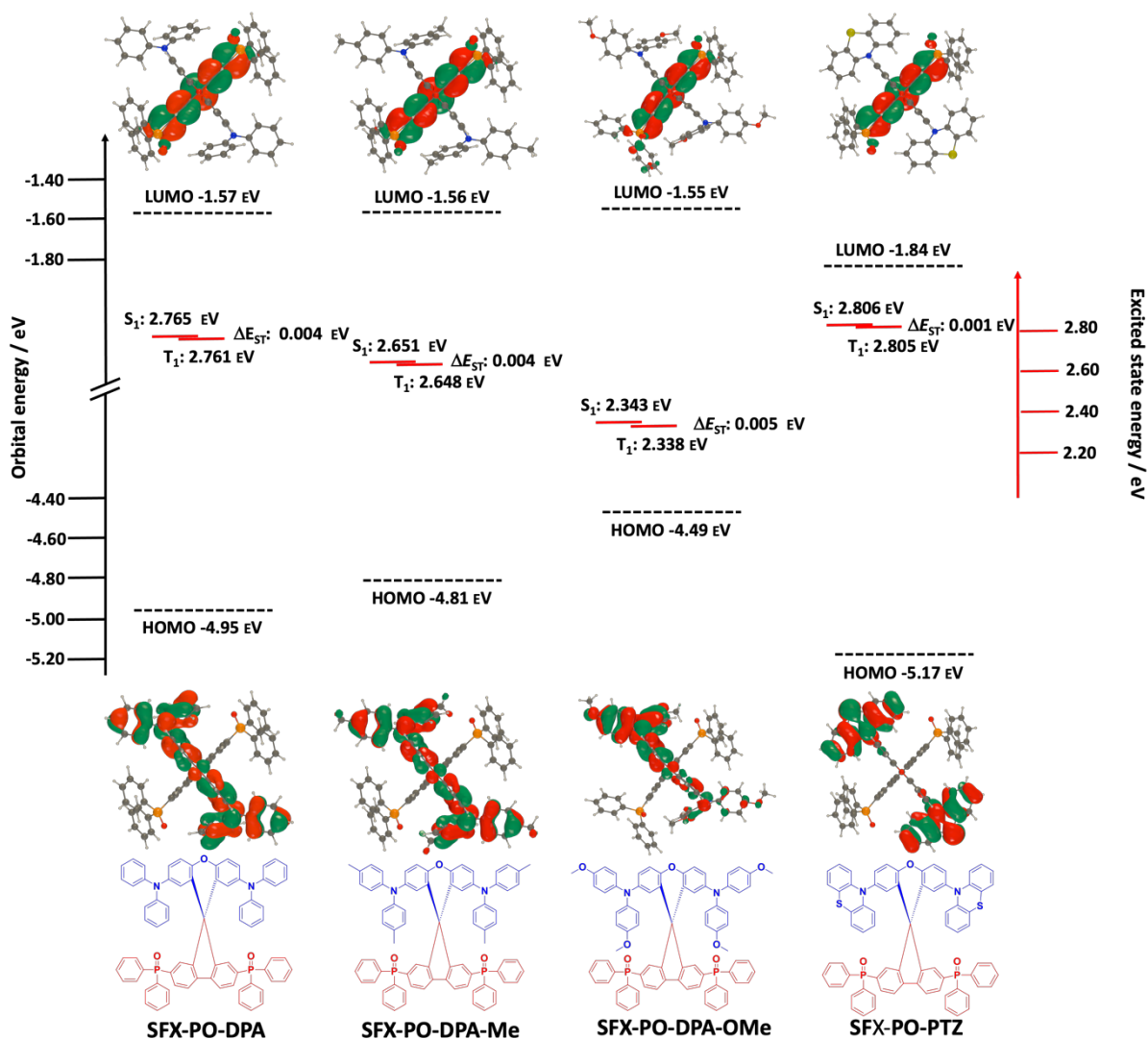
Figure 6. Calculated HOMO, LUMO (as obtained at DFT PBE0 6-31G(d,p) level) S_1 and T_1 energies (as obtained at TDA-DFT PBE0 6-31G(d,p) level), and contour plots of the HOMO and LUMO orbitals of SFX-PO-DPA, SFX-PO-DPA-Me, SFX-PO-DPA-OMe and SFX-PO-PTZ.
