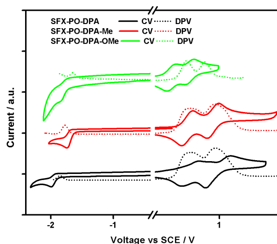
Figure 4. Cyclic Voltammograms and Differential Pulse Voltammograms of SFX-PO-DPA , SFX-PO-DPA-Me and SFX-PO-DPA-OMe (Oxidation and reduction was performed in degassed DCM and DMF, respectively; scan rate: 100 mV s -1 ).
