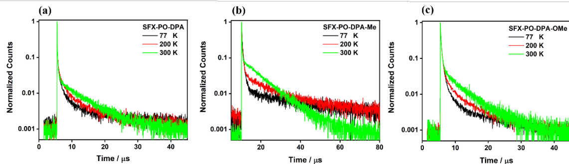
Figure 8. Temperature-dependent time-resolved PL decay traces of doped films in mCP with (a) 10 wt% SFX-PO-DPA (b) 15 wt% SFX-PO-DPA-Me and (c) 10 wt% SFX-PO-DPA-OMe ( \lambda_{\text{exc}} = 378 nm).
