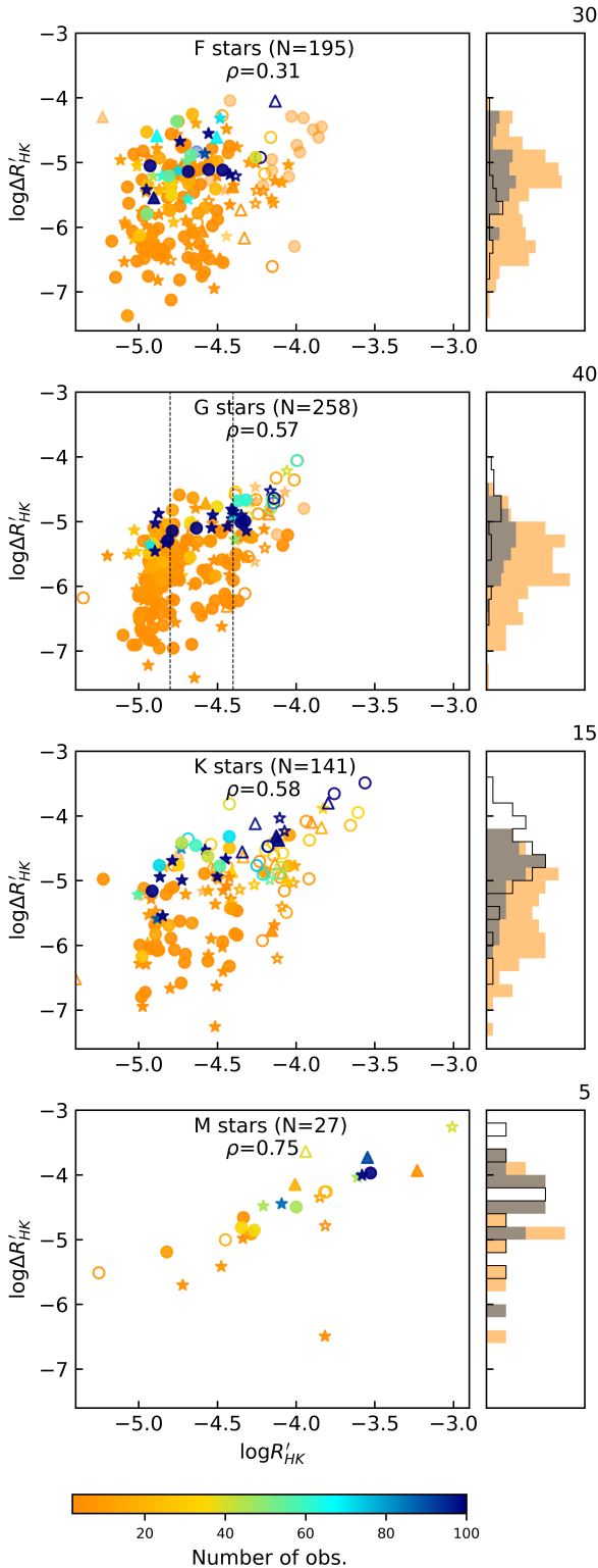
Figure 5. Amplitude of chromospheric activity variability versus mean chromospheric activity for samples of F, G, K and M stars. Marker shapes and fill-styles are the same as in Figure 1. Marker color scales with the number of observations. The histograms to the right of the plots indicate the distributions of \log \Delta R'_{HK} for the entire main sequence sample (orange), main sequence stars with \geq 10 observations (grey), and young stars (black line). The dashed lines correspond to the reduced population of G stars from Figure 4.
