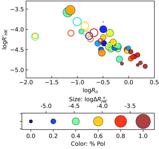
Figure D1. Mean \log R'_{HK} versus the theoretical Rossby number taken from See et al. (2019a) , where marker colour shows the fractional poloidal field and marker size scales with chromospheric activity variability.
