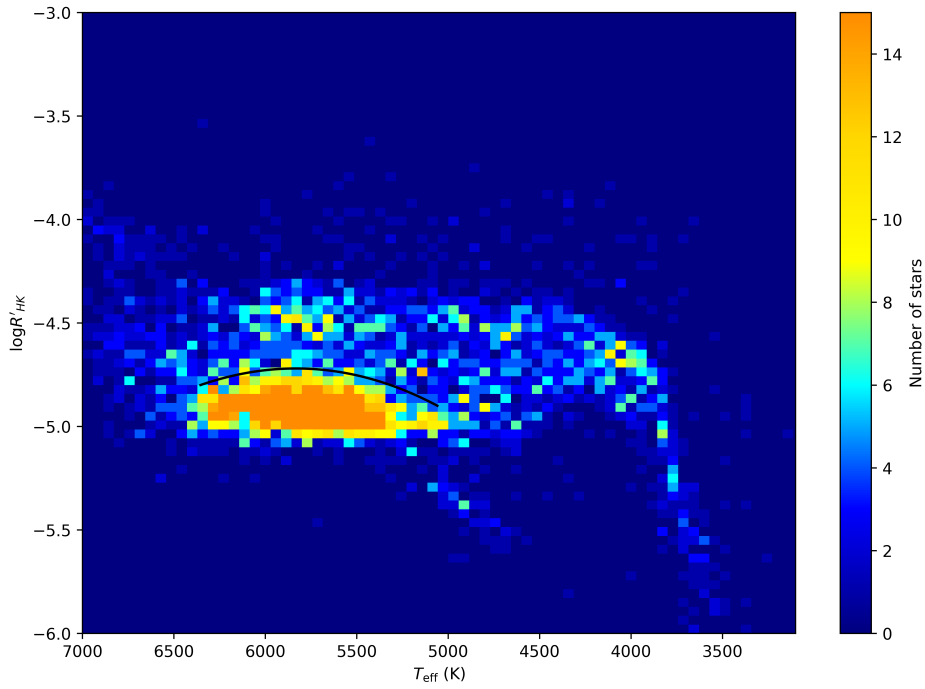
Figure 9. Two-dimensional histogram indicating the number of stars in Figure 8 populating equal-sized temperature and \log R'_{HK} bins. For targets that are common to both PolarBase and the published data we take the mean of all available \log R'_{HK} values for Figure 9. The black curve we have drawn is intended to draw the eye to the densely populated region we discuss in section 5.4, and corresponds to the black curve shown in Figure 8.
