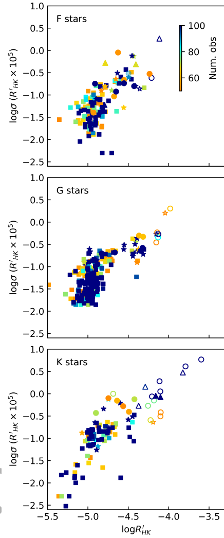
Figure C1. Activity variability versus mean activity level for our data and the HARPS sample studied by Gomes da Silva et al. (2020). Squares indicate data from Gomes da Silva et al. (2020), while circles, stars and triangles show our data, with marker styles the same as in Figure 1. For stars common to both studies we have shown our results only. We have filtered the data to show only stars with \geq 50 observations, and marker color scales with the number of observations.
