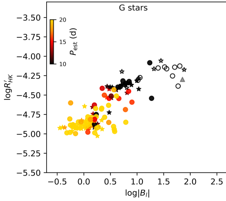
Figure B1. Mean chromospheric activity versus mean longitudinal magnetic field strength for G stars, where color scales with the estimated rotation period, P_{\text{est}, i=60^\circ} . Marker shapes/styles are the same as in Figure 1.
