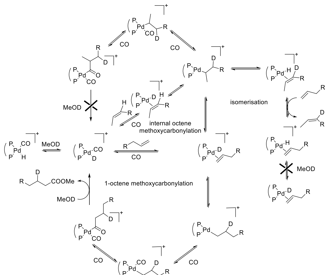
Figure 36: Reactions occurring during the tandem isomerization-methoxycarbonylation reaction of alkenes catalyzed by Pd complexes of 1,2-DTBPMB, \text{P} \text{---} \text{P} . Based on Refs. 77, 161
