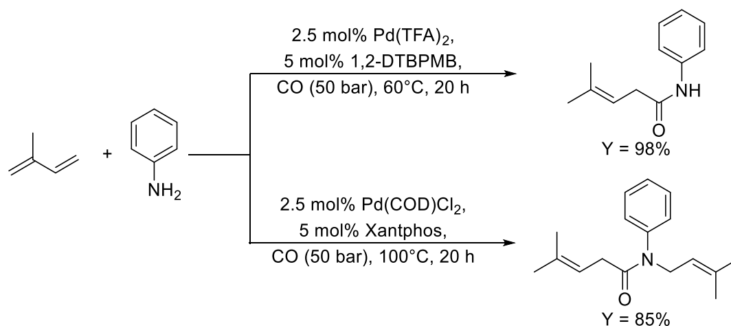
Figure 43: the role of 1,2-DTBPMB in aminocarbonylation of dienes. Adapted from Ref. 169 . Copyright [2014] American Chemical Society.
