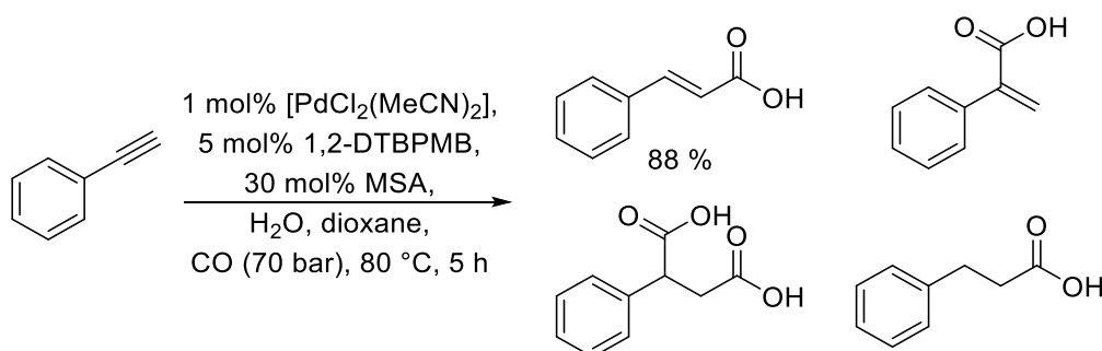
Figure 34: Pd/1,2-DTBPMB mediated hydroxycarbonylation of phenyl acetylene. Adapted with permission from Ref. 5 . Copyright [2010] Royal Society of Chemistry.
