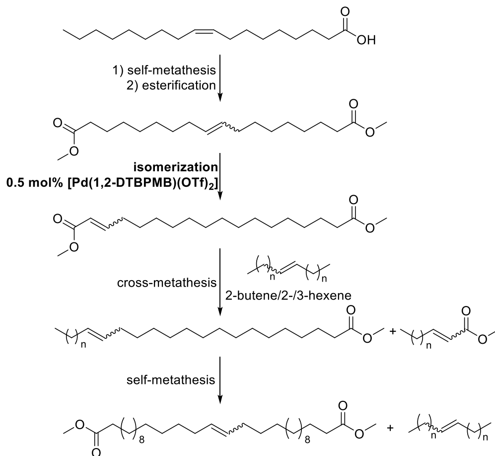
Figure 61: metathesis and isomerization of fatty acid (methyl esters) for synthesis of ultra-long-chain \alpha,\omega -diesters ( n = 0, 1, 2 ). Adapted with permission from Ref. 208 . Copyright [2017] John Wiley and Sons.
