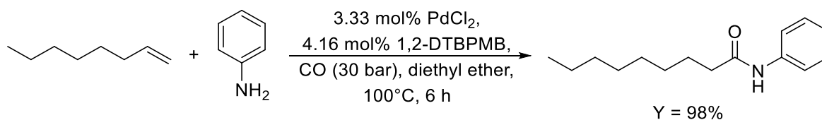
Figure 41: Pd/1,2-DTBPMB mediated aminocarbonylation of 1-octene. Adapted with permission from Ref. 168 . Copyright [2014] Royal Society of Chemistry.
