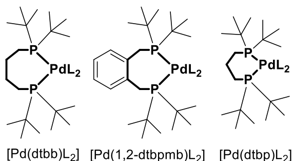
Figure 58: Ring strain in Pd-complexes of DTBB (left), 1,2-DTBPMB (middle), DTBP (right).
