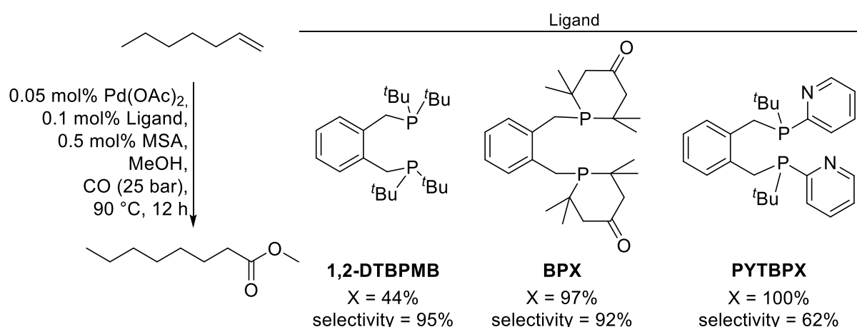
Figure 79: Comparison of 1,2-DTBPMB, BPX and PYTBPX in the methoxycarbonylation of 1-heptene as model compound for hyperbranched oligoethenes. 228
