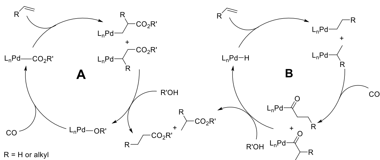
Figure 7: The two proposed general catalytic cycles for alkoxy carbonylation of ethene and alkenes respectively: A : carbomethoxy mechanism, B : hydride mechanism. Adapted with permission from Ref. 51 . Copyright [1991] Elsevier.
