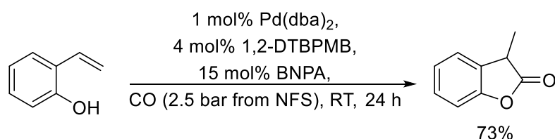
Figure 54: Pd/1,2-DTBPMB mediated intramolecular methoxycarbonylation of 2-vinylphenol using N -formylsaccharin as CO surrogate. Adapted with permission from Ref. 188 . Copyright [2018] John Wiley and Sons.
