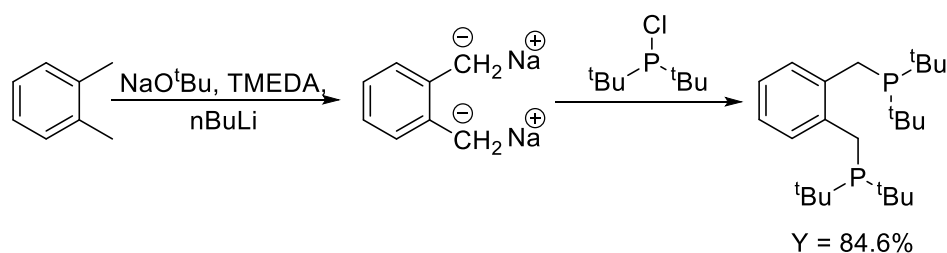
Figure 5: procedure for the synthesis of 1,2-bis(di- tert -butylphosphinomethyl)benzene starting from o-xylene. 14
