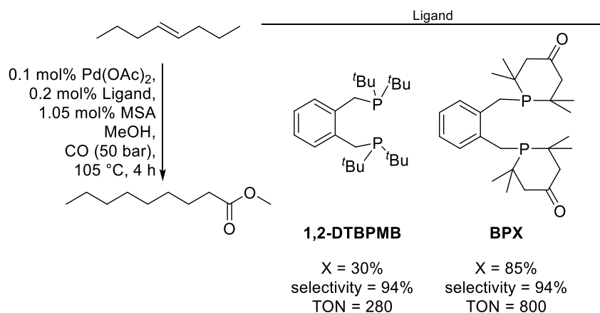
Figure 75: Comparison of 1,2-DTBPMB and BPX in the methoxycarbonylation of trans -4-octene. 226
