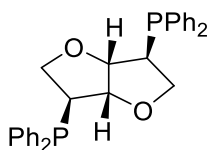
Figure 15: 1,4:3,6-dianhydro-2,5-dideoxy-2,5-bis(diphenylphosphino)-L-iditol (DDPPI) as non-chelating diphosphine. 92
