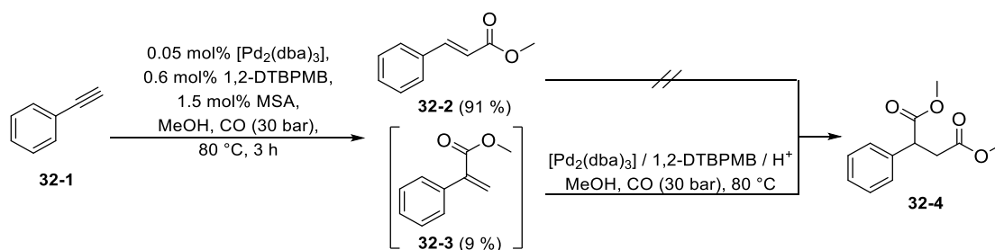
Figure 32: Pd/1,2-DTBPMB mediated methoxycarbonylation of phenylacetylene. Adapted with permission from Ref. 5 . Copyright [2010] Royal Society of Chemistry.
