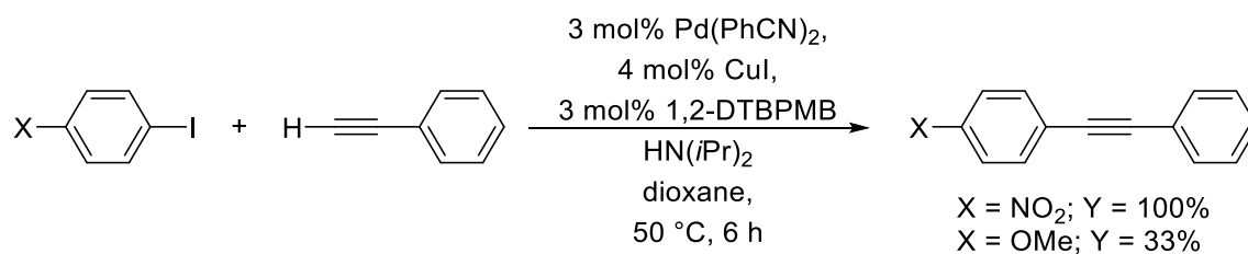
Figure 67: Pd/1,2-DTBPMB mediated Sonogashira reaction. Adapted with permission from Ref. 216 . Copyright [2007] Elsevier.
