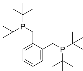
Figure 2: Chemical structure of 1,2-bis(di- tert -butylphosphinomethyl)benzene.
