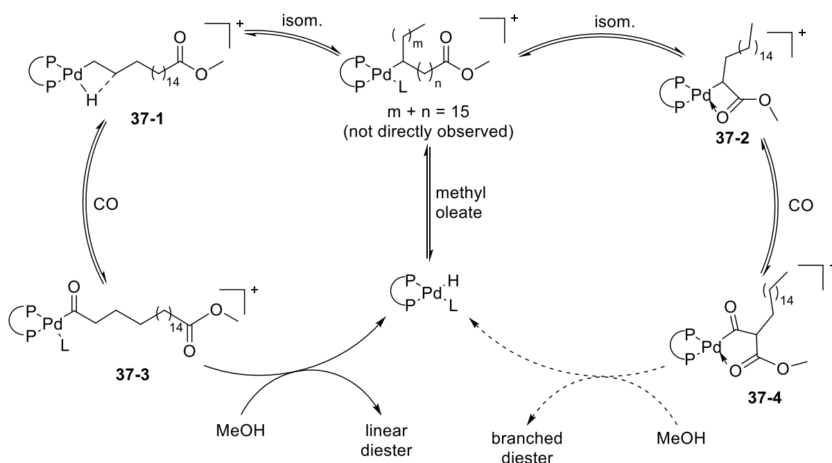
Figure 37: Proposed isomerization and alkoxyacylation mechanism of methyl oleate. 164 P ^ —P = 1,3-bis(di- tert -butylphosphino)propane. Reproduced from Ref. 164 . Copyright [2012] American Chemical Society..
