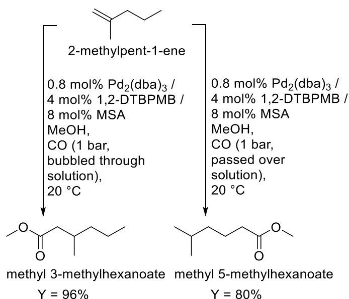
Figure 18: dependence of Pd/1,2-DTBPMB mediated isomerization on CO availability. 77
