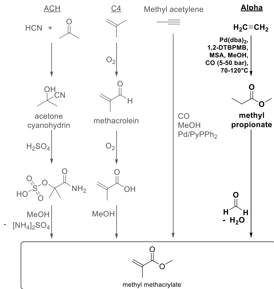
Figure 6: Lucite's Alpha process, Methoxycarbonylation of ethene to methyl propionate and conversion to methyl methacrylate as alternative to ACH-, methylacetylene- and C4-routes.
