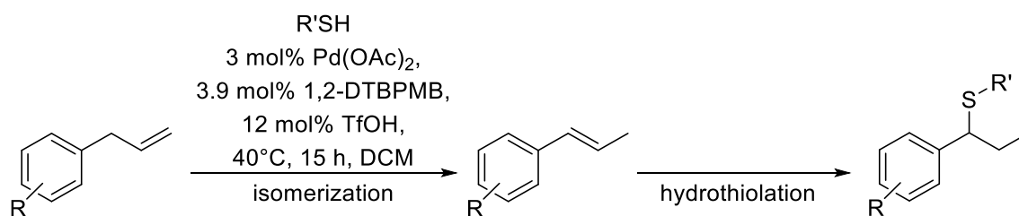
Figure 62: Pd/1,2-DTBPMB mediated tandem isomerization/hydrothiolation of allylarenes. Adapted from Ref. 209 . Copyright [2019] American Chemical Society.
