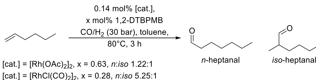
Figure 47: hydroformylation of 1-hexene using 1,2-DTBPMB as ligand. 174
