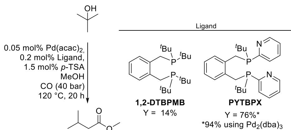
Figure 78: Comparison of 1,2-DTBPMB and its o -pyridyl derivative in the carbonylation of tert -butanol. 179
