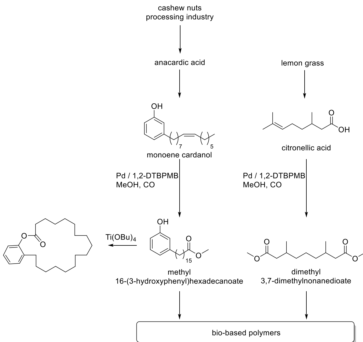
Figure 29: Pd / 1,2-DTBPMB mediated methoxycarbonylation of natural oils. 144,145
