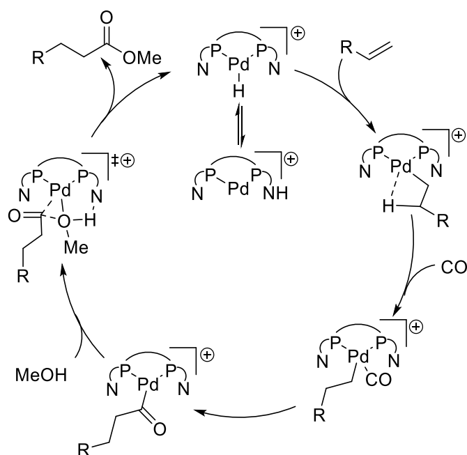
Figure 81: Proposed mechanism for the alkoxy carbonylation using ligand 79-e . Reproduced with permission from Ref. 230 . Copyright [2018] Royal Society of Chemistry.
