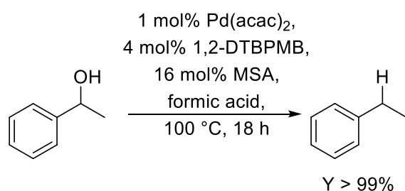
Figure 56: Pd/1,2-DTBPMB mediated transfer hydrogenolysis of benzylic alcohols. Adapted with permission from Ref. 201 . Copyright [2018] John Wiley and Sons.
