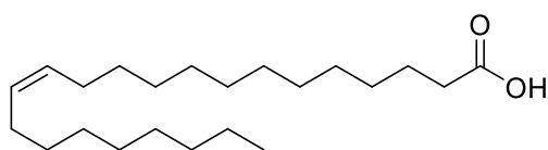
Figure 26: Erucic acid.
