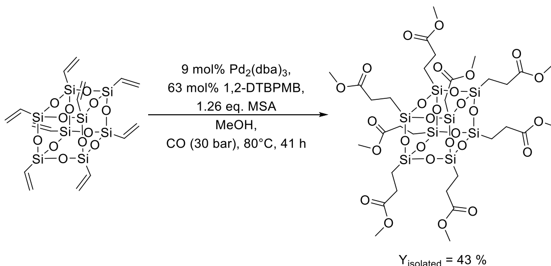
Figure 14: Preparation of OMPO via methoxycarbonylation reaction. Adapted with permission from Ref. 88 . Copyright [2006] Elsevier.
