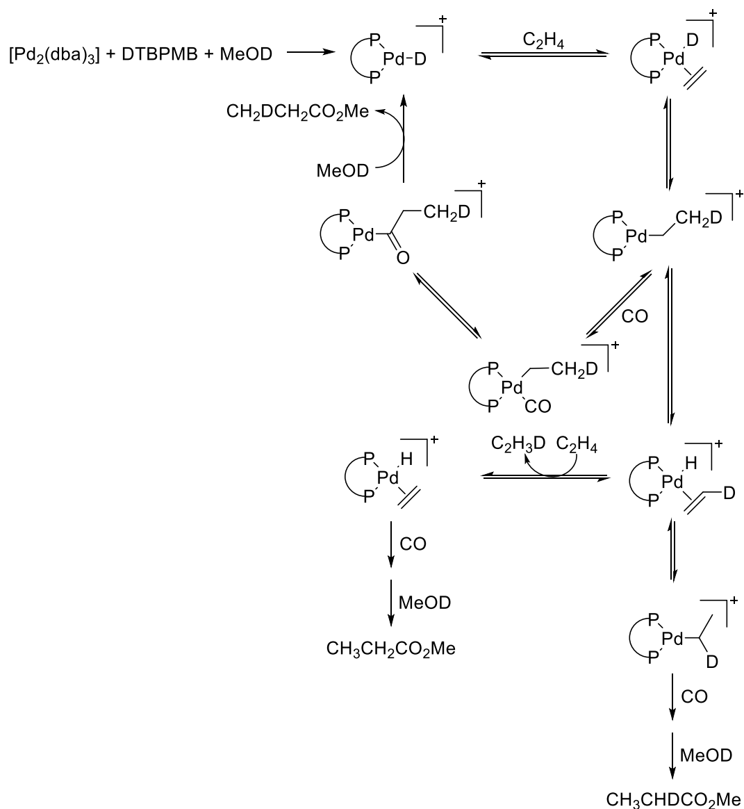
Figure 8: Proposed hydride mechanism for the formation of H/D-methyl propanoate from CO, ethene and MeOD catalyzed by Pd/1,2-DTBPMB system. P—P = 1,2-DTBPMB. Reproduced with permission from Ref. 62 . Copyright [2002] Royal Society of Chemistry.
