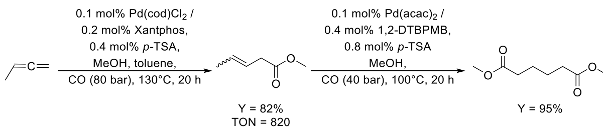
Figure 22: Xantphos-mediated methoxycarbonylation of 1,2-butadiene and subsequent 1,2-DTBPMB-mediated methoxycarbonylation of the intermediate pentenoic acid ester. Adapted from Ref. 124 . Copyright [2015] American Chemical Society.
