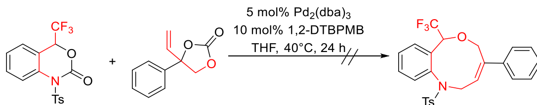
Figure 65: Approach of Pd/1,2-DTBPMB mediated double decarboxylative cycloaddition. Adapted with permission from Ref. 211 . Copyright [2018] Royal Society of Chemistry.
