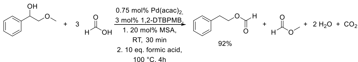
Figure 57: Pd/1,2-DTBPMB mediated reductive rearrangement of 2-methoxy phenylethanol. 202
