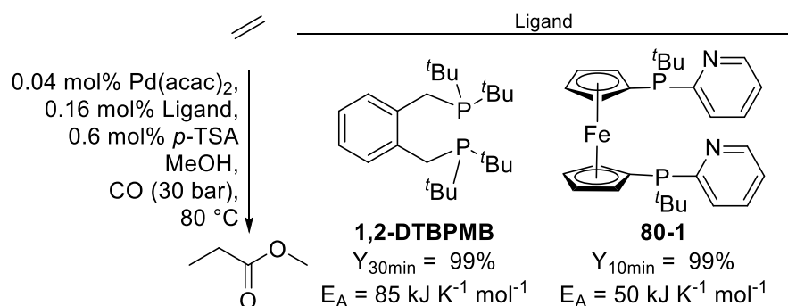
Figure 80: Comparison of 1,2-DTBPMB and the novel ferrocene derivative 79-1 in the methoxycarbonylation of ethene. 229
