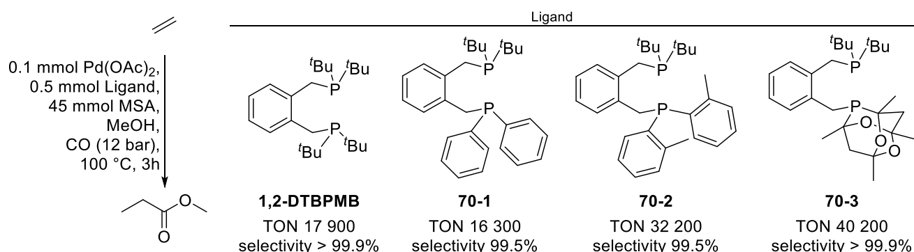
Figure 70: comparison of 1,2-DTBPMB derivatives in the methoxycarbonylation of ethene.
