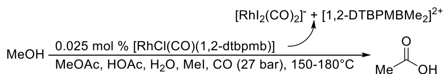
Figure 48: Rh/1,2-DTBPMB mediated methanol carbonylation to acetic acid and decomposition to Monsanto catalyst. 175
