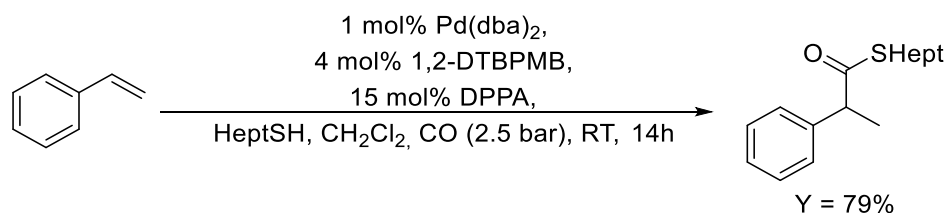
Figure 49: Pd/1,2-DTBPMB mediated thiocarbonylation of styrene. Adapted from Ref. 180 . Copyright [2016] American Chemical Society.
