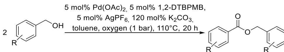
Figure 69: Oxidative esterification of benzylic alcohols. Adapted with permission from Ref. 218 . Copyright [2011] John Wiley and Sons.
