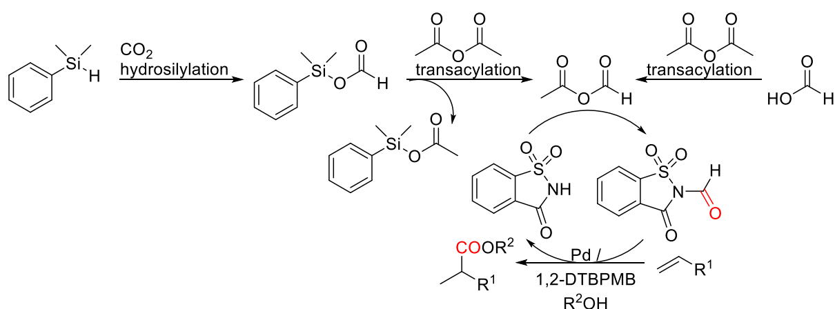
Figure 53: N -formylsaccharin as CO surrogate in the Pd / 1,2-DTBPMB mediated methoxycarbonylation. Adapted with permission from Ref. 187 . Copyright [2015] Royal Society of Chemistry.
