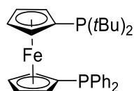
Figure 50: DTBDPPF as optimized ligand for successful thiocarbonylation of styrene
