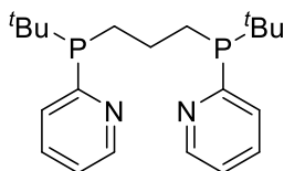
Figure 33: 1,3-bis( tert -butyl(pyridin-2-yl)phosphanyl)propane.
