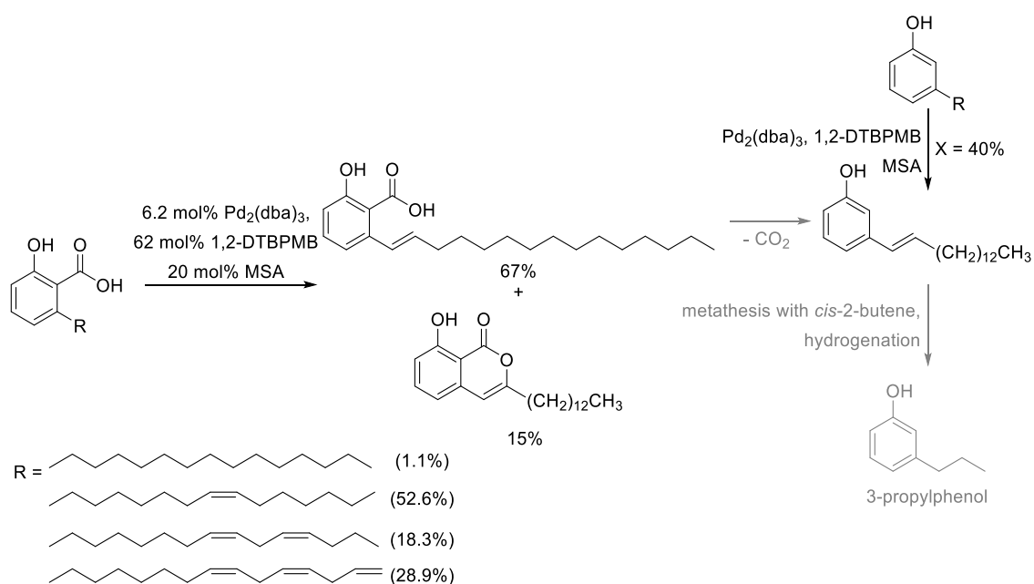
Figure 60: Pd/1,2-DTBPMB mediated isomerization of anacardic acid and cardanol. 206
