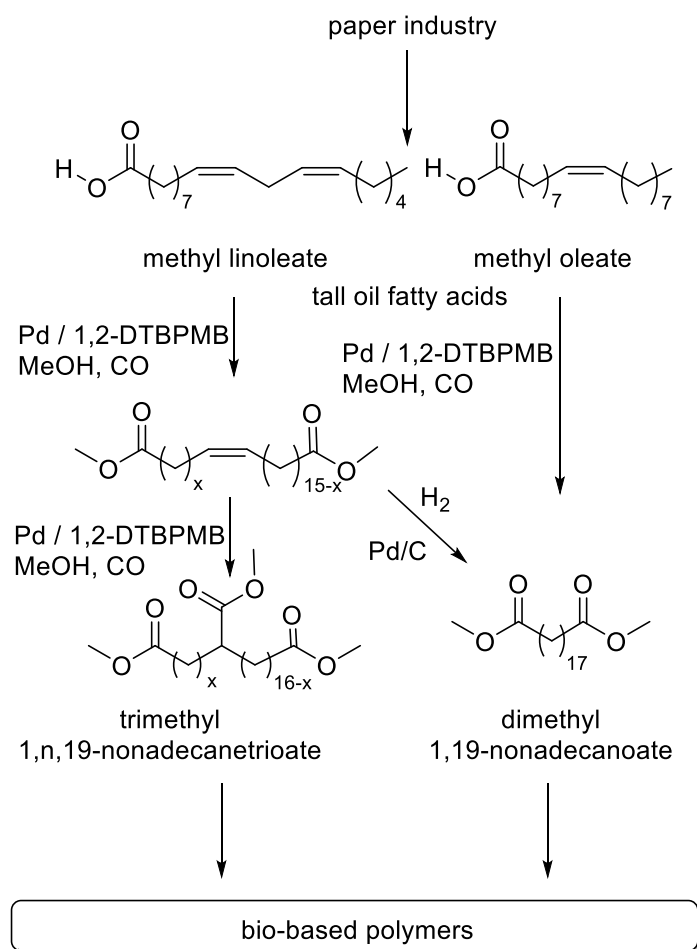
Figure 28: The role of 1,2-DTBPMB in the production of bio-based polymers from tall oil. 127
