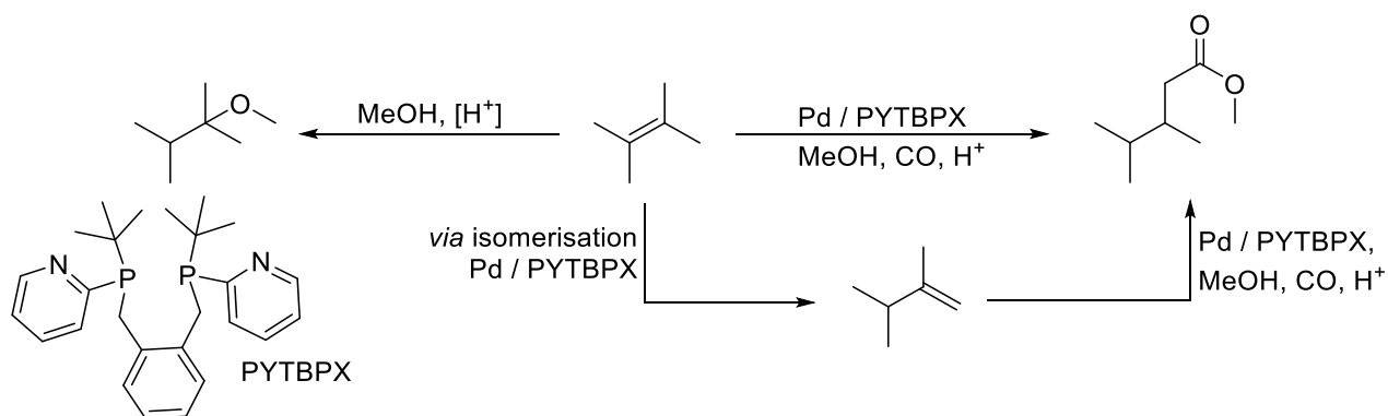
Figure 76: Pd/PYTBPX mediated Methoxycarbonylation of tetramethylethene. 227
