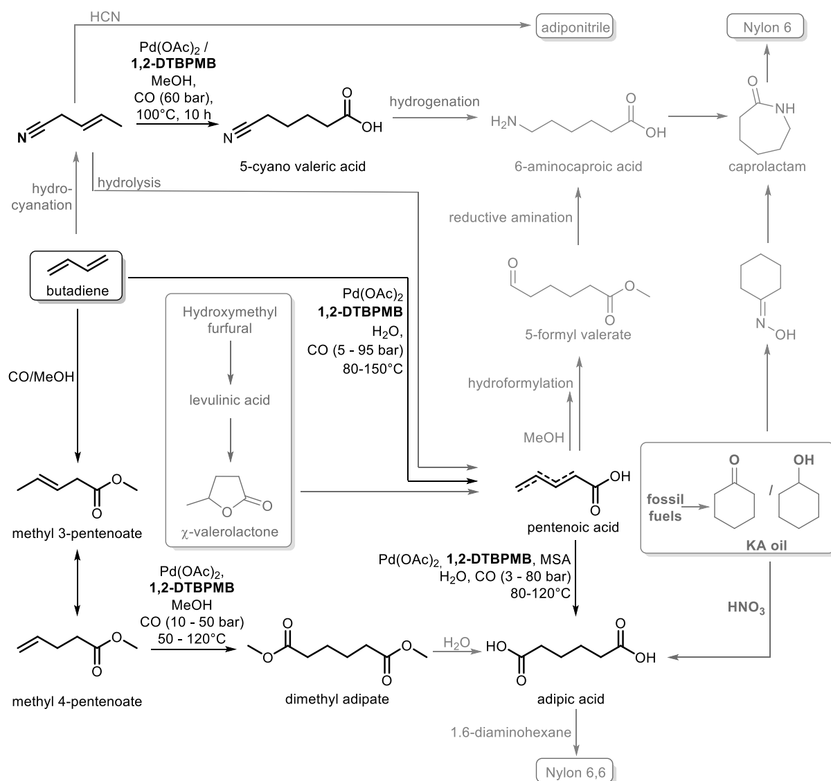
Figure 21: the role of 1,2-DTBPMB for the production of C6 polymer building blocks. For references, see text.
