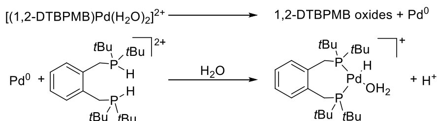
Figure 40: Formation of a Pd/1,2-DTBPMB hydride species as a two-step process in the hydroxycarbonylation. 138
