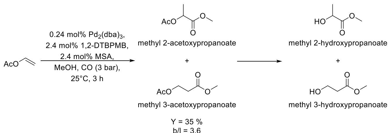
Figure 13: The methoxycarbonylation of vinyl acetate as an intermediate step in the production of methyl lactate. Adapted with permission from Ref. 69 . Copyright [2006] John Wiley and Sons.
