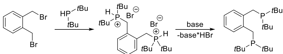
Figure 3: First reported general procedure for the synthesis of 1,2-bis(di-tert-butylphosphinomethyl)benzene via phosphonium salt. 3,11
