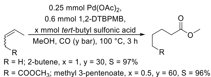
Figure 17: Methoxycarbonylation of 2-butene/methyl 3-pentenoate, indicating isomerization activity of 1,2-DTBPMB. 76
