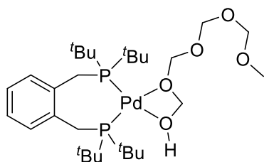
Figure 52: Exemplary coordination of \text{MeO}(\text{CH}_2\text{O})_4\text{H} as model compound to Pd/1,2-DTBPMB. Adapted from Ref. 186
