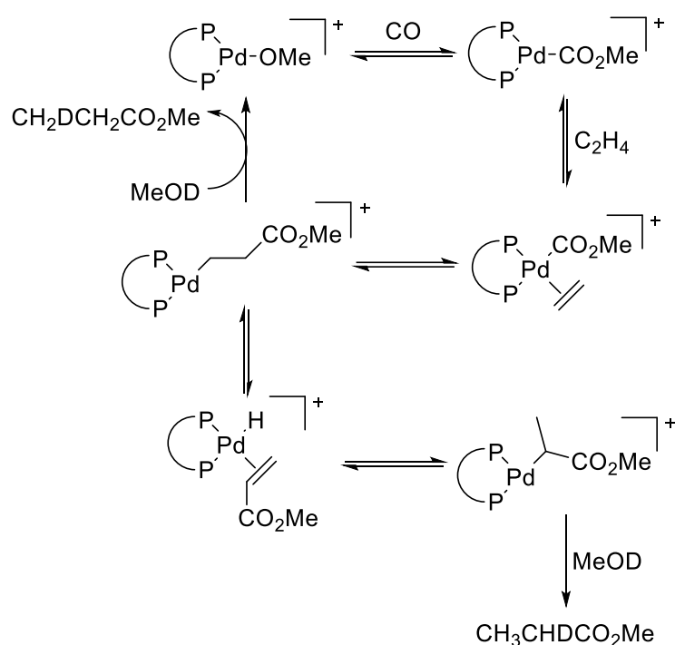
Figure 9: Proposed carbomethoxy mechanism for the formation of variously deuterated methyl propanoate from CO, ethene and MeOD catalyzed by Pd/1,2-DTBPMB system. P—P = 1,2-DTBPMB. Reproduced with permission from Ref. 62 . Copyright [2002] Royal Society of Chemistry.
