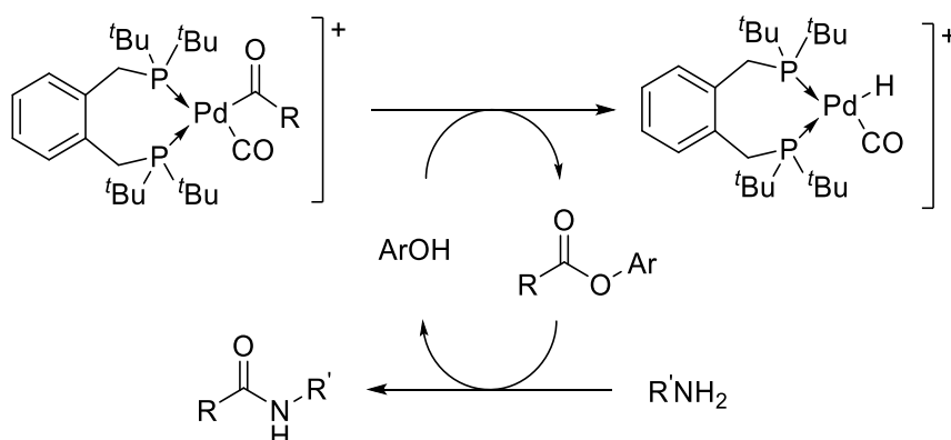
Figure 42: role of 2-Naphthol in Pd/1,2-DTBPMB mediated aminocarbonylation. Reproduced with permission from Ref. 168 . Copyright [2014] Royal Society of Chemistry.
