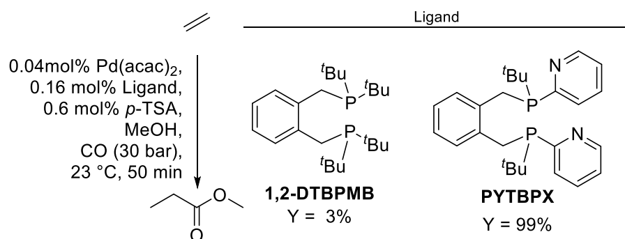
Figure 77: Comparison of 1,2-DTBPMB and its o -pyridyl derivative in the methoxycarbonylation of ethene at room temperature. 227
