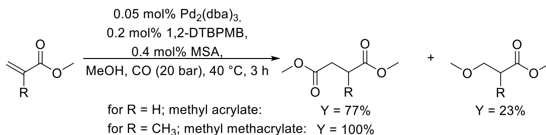
Figure 19: Methoxycarbonylation of methyl acrylate. Adapted with permission from Ref. 98 . Copyright [2004] Royal Society of Chemistry.
