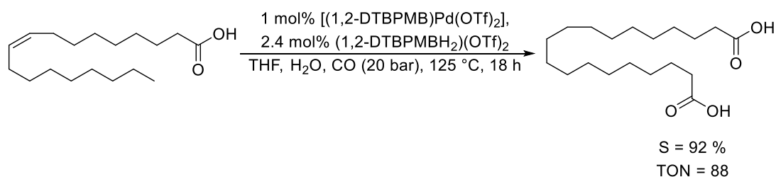
Figure 25: Pd/1,2-DTBPMB mediated isomerizing hydroxycarbonylation of oleic acid in THF. 138
