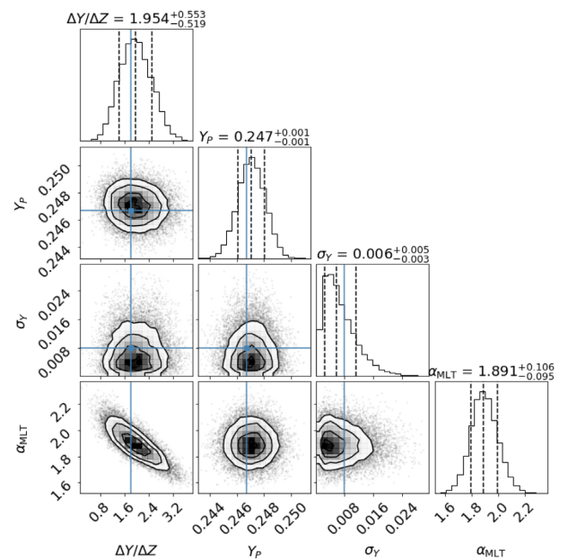
Figure C3. The same as Fig. C2 but for the MP model.
