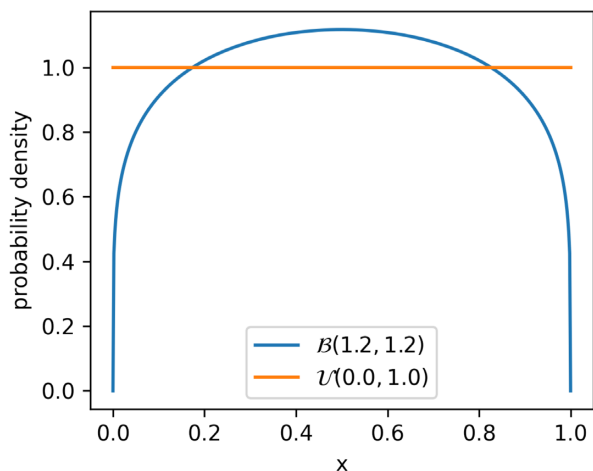
Figure B1. A beta distribution ( B ) with \alpha = \beta = 1.2 for some parameter x and a uniform distribution ( U ) from 0 to 1.
