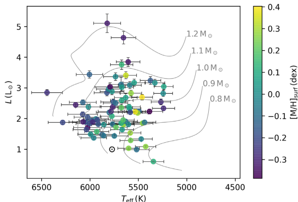
Figure 1. The luminosity, L against effective temperature, T_{\text{eff}} of the sample of 81 Kepler dwarfs, and subgiants studied in this work. Each star is coloured according to metallicity. The grey lines depict evolutionary tracks with [\text{M}/\text{H}]_{\text{init}} = 0.0 dex, Y_{\text{init}} = 0.28 , and \alpha_{\text{MLT}} = 1.9 for different stellar masses. The current position of the Sun is shown by the \odot symbol.
