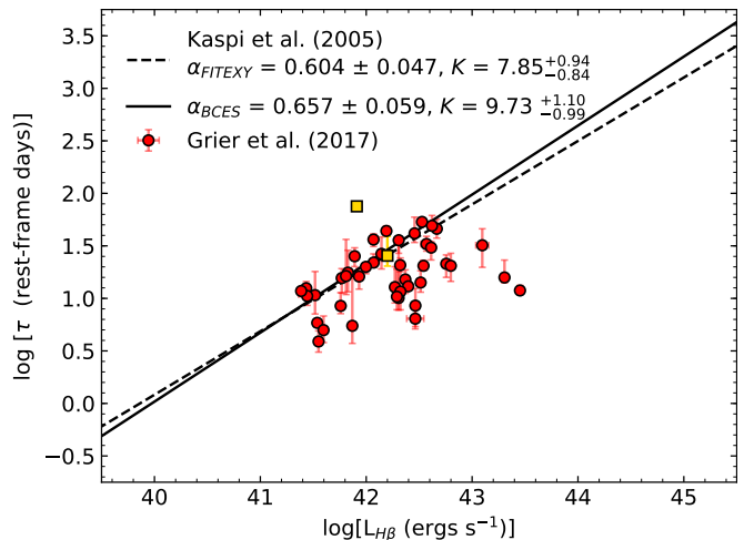
FIG. 4.— The R - L(H\beta) relation for the 44 SDSS-RM AGN, with H\beta time lags from Grier et al. (2017) and broad-line H\beta luminosity from Shen et al. (2019). Black solid and dashed lines show the relation between H\beta time lags and L_{H\beta} from Kaspi et al. (2005) for two different fitting methods. The SDSS-RM AGN have lags that fall below the R - L(H\beta) relation.
