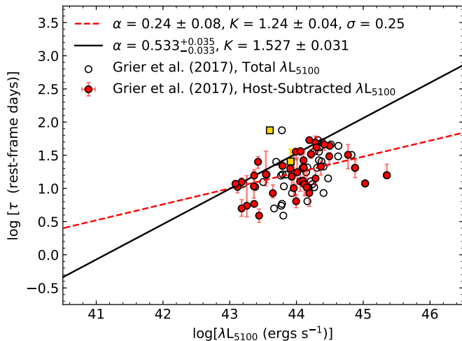
FIG. 3.— The R - L relation for 44 AGN in the SDSS-RM survey, with H\beta time lags from Grier et al. (2017) and \lambda L_{5100} from Shen et al. (2015a). Out of the 44 lags, 32 were measured using JAVELIN and 12 were measured using CREAM. The open circles have \lambda L_{5100} that includes host-galaxy light, while the solid red circles have AGN luminosities ( \lambda L_{5100} ) that are host-subtracted using principal component analysis of the coadded spectra. Our best-fit line for the red (host-subtracted) points is shown as the red dashed line, with a slope \alpha = 0.24 \pm 0.08 and a normalization of K = 1.24 \pm 0.04 that both differ from the Bentz et al. (2013) best-fit R - L relation (shown as the black solid line) by > 3\sigma . The two square points were excluded from the fitting (see text for details). The SDSS-RM AGN generally have lags that are shorter than expected from the Bentz et al. (2013) R - L relation at a given host-subtracted \lambda L_{5100} .
