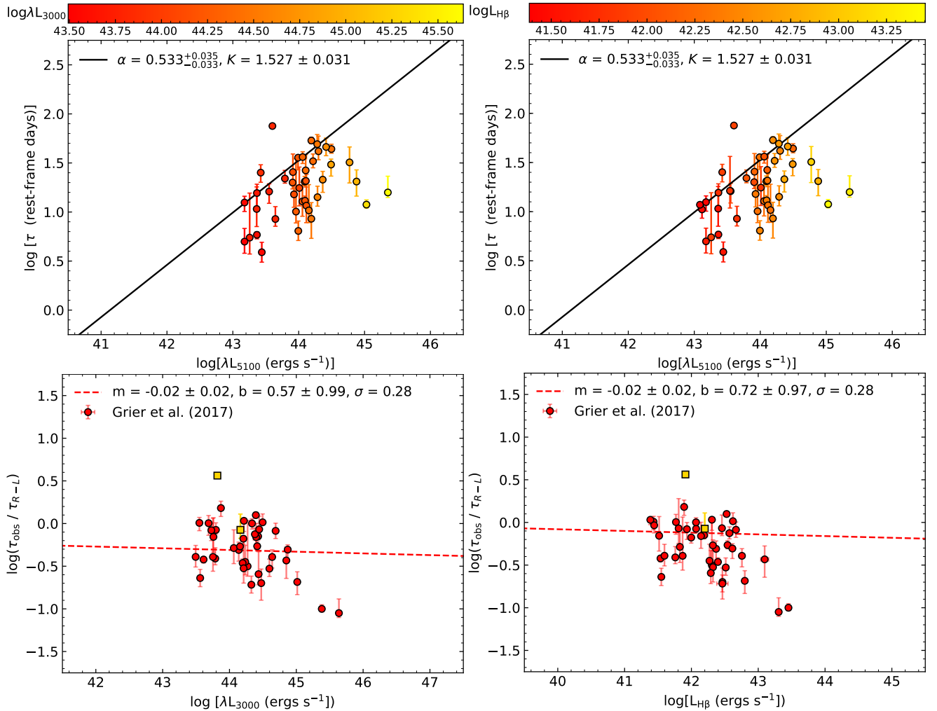
FIG. 12.— Left: The R-L relation of SDSS-RM AGN color-coded by \lambda L_{3000} and the R-L offset \tau_{\text{obs}}/\tau_{R-L} versus \lambda L_{3000} , a luminosity measurement closer to the ionizing UV luminosity than the \lambda L_{5100} used in the R-L relation. The sample spans a fairly narrow range of \lambda L_{3000}/\lambda L_{5100} (top left) and the R-L offset is not anti-correlated with \lambda L_{3000} (slope 1\sigma from zero and Spearman’s \rho = -0.28 and p = 0.09 ). Right: The R-L relation of SDSS-RM AGN with the H\beta broad-line luminosity and the R-L offset versus the H\beta broad-line luminosity, a proxy for the ionizing luminosity that drives H\beta recombination. Once more the sample spans a fairly narrow range of L_{H\beta}/\lambda L_{5100} , and the R-L offset and L_{H\beta} are not significantly correlated with a slope m that is 1\sigma consistent with zero, and Spearman’s \rho = -0.36 and p = 0.02 , with excess scatter of \sim 0.25 dex about the best-fit line.
