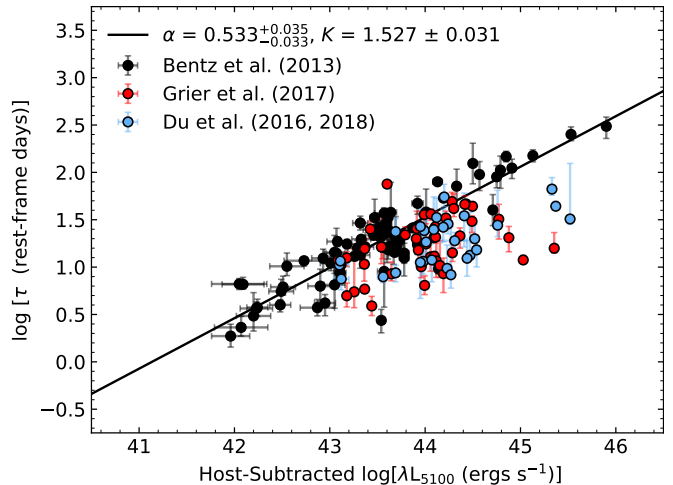
FIG. 1.— The R-L relation for H\beta time lags from Bentz et al. (2013), Grier et al. (2017), and Du et al. (2016, 2018). The black line shows the R-L relation from Bentz et al. (2013), with a slope \alpha = 0.533 and a normalization K = 1.527 . The lag measurements from SDSS-RM (Grier et al. 2017) and SEAMBH (Du et al. 2018) frequently lie below the R-L relation established by Bentz et al. (2013).
