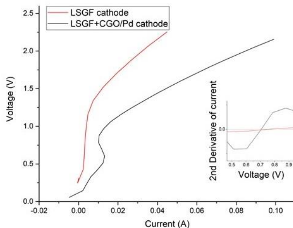
Figure 10 Comparison between polarization curves at 600 °C of electrolysers with anode LSGF, electrolyte LSGM and cathode as indicated in legend, cathode is fed with 50% H 2 O in N 2 and anode is fed with air.
