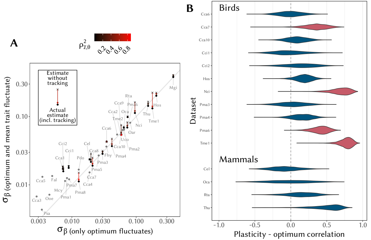
Figure 3: Phenotypic tracking of fluctuations in the optimum. A: Standard deviation of the selection gradient \beta_t (dots: actual values \sigma_{\beta} ; crosses: computation assuming no tracking, i.e. \rho_{\bar{z},\theta} = 0 in Equation 3) against the standard deviation expected when using optimum fluctuations only (i.e. \sigma_{\bar{z}} = 0 in Equation 3). Arrows show the direction of the change when accounting for tracking, and the red scale indicates the actual value of \rho_{\bar{z},\theta}^2 . Note that long arrows tend to be red, while short arrows tend to be grey. For datasets with minority support for an optimum compared to the directional models, only greyed-out dots are displayed. The identity line is depicted in grey. B: For the 15 datasets with predominant support for an optimum and repeated measures, posterior distributions (coming from propagated Bayesian uncertainty) of the correlation coefficients between shifts in the optimum and shifts in the average phenology for individuals measured in two consecutive years. In light red: the distribution does not contain zero in the 95% highest density posterior interval. The dataset codes are explained in Table S1.
