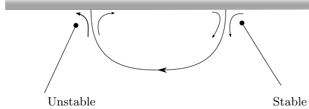
FIGURE 13. Schematic diagram showing the structure of streamlines for a steady state solution with a rotating core of fluid in a region of closed streamlines. The stable and unstable streamline configurations are marked on the diagram. This diagram can also be compared with the streamlines shown in figure 9.
