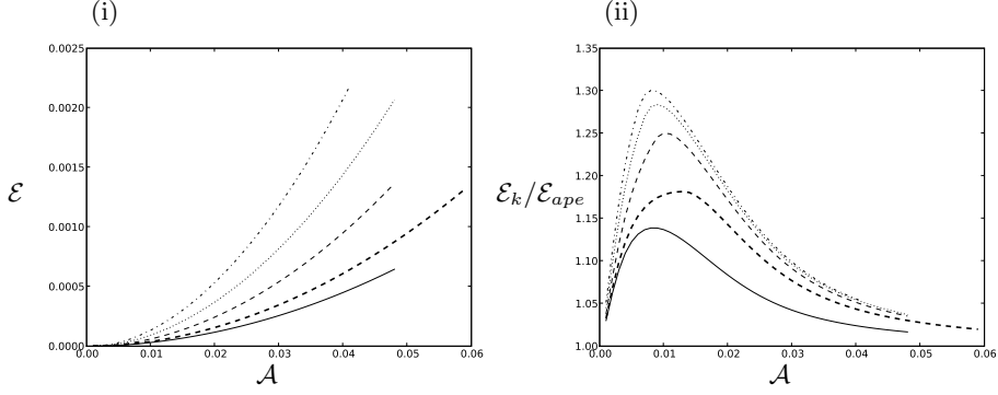
FIGURE 17. (i) The total energy \mathcal{E} and (ii) the ratio of kinetic energy to available potential energy \mathcal{E}_k/\mathcal{E}_{ape} versus \mathcal{A} for the set of cases given in table 2.
