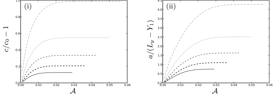
FIGURE 14. (i) Non-dimensionalised wave speed versus the amplitude of the wave \mathcal{A} . (ii) Shows a typical measure of amplitude used in many previous studies ( a/(L_y - Y_1) , where a is the maximum deflection of the streamline which coincides with the height Y_1 upstream) plotted against the current amplitude measure \mathcal{A} . The plot is for parameter values and line styles as given in table 1.
