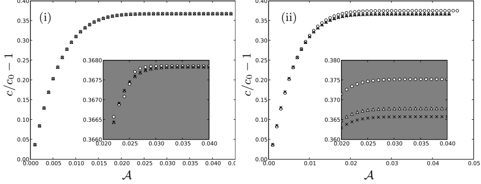
FIGURE 3. Plots of scaled wave speed c/c_0 - 1 versus amplitude \mathcal{A} . (i) Shows the effect of changing the resolution of the computation while keeping the smoothing distance \delta/L_y = 2/128 fixed. This smoothing length corresponds to two grid lengths in the standard resolution. (ii) Shows the effect of changing the resolution (as in plot (i)) where the smoothing is set always to be \delta = 2\Delta y , that is, two grid lengths of the given resolution. In each case the symbols correspond to \circ = (512 \times 64) , \triangle = (1024 \times 128) and \times = (2048 \times 256) in resolution. The underlying setup is three layers with Y_1/L_y = 0.81 , Y_2/L_y = 0.86 and N_0^2 = N_2^2 = 0 , N_1^2 = 1 . In both plots the grey regions are zoomed regions from the main plot to better see the differences between each of the curves.
