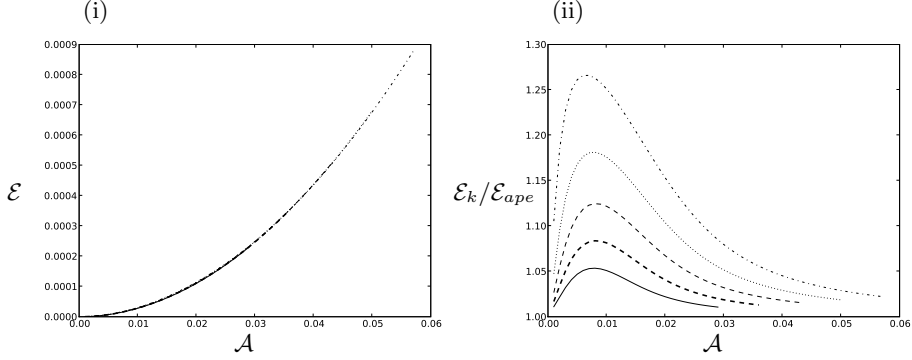
FIGURE 16. (i) The total energy \mathcal{E} (kinetic plus available potential energy, see equation (3.3)) contained in the wave plotted as a function of wave amplitude \mathcal{A} . (ii) The ratio of kinetic energy to available potential energy \mathcal{E}_k/\mathcal{E}_{ape} versus \mathcal{A} . The parameters and line styles are given in table 1.
