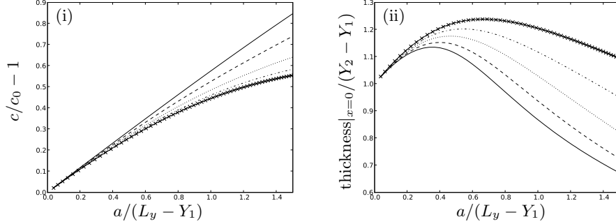
FIGURE 6. (i) Non-dimensionalised wave speed versus amplitude and (ii) pycnocline thickness at the midpoint of the wave versus amplitude. In both plots the amplitude measure is that used in Fructus & Grue (2004), (to compare to their figure 9(c)). The stratification is such that Y_1/L_y = 0.81 and Y_2/L_y = 0.94 , N_0^2 = 0 , N_1^2 = 1 . The different curves represent different values of N_2 : N_2 = 0 (-x), 0.5 (-.), 0.7 (...), 0.87 (- -), 1.0 (-).
