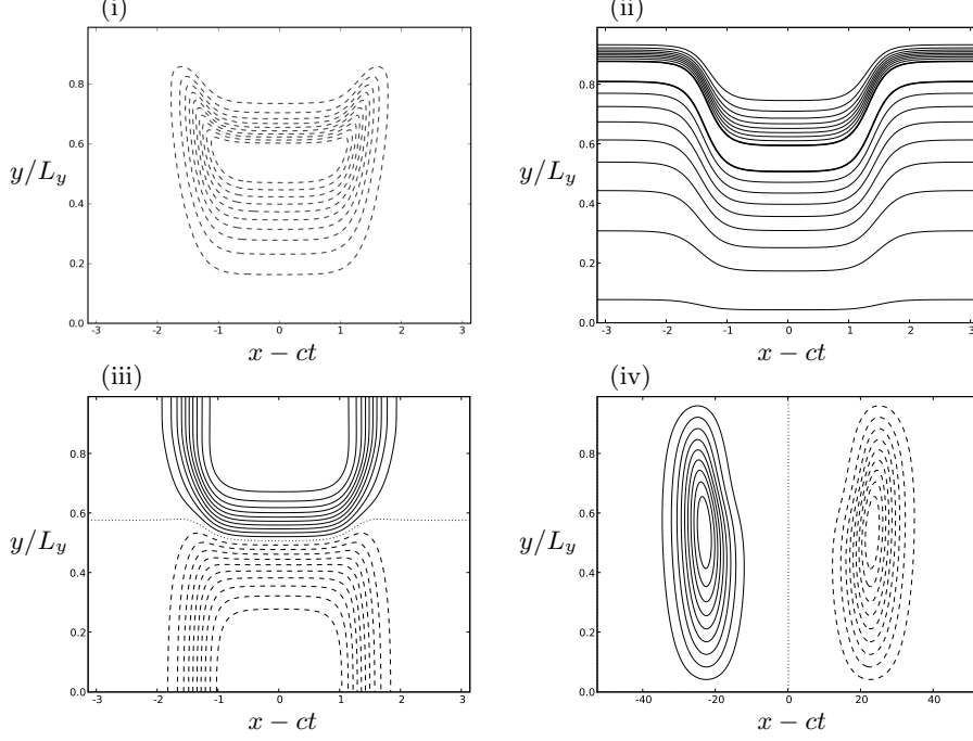
FIGURE 21. (i) \zeta (ii) N^2 (iii) u - c and (iv) v for a wave with amplitude \mathcal{A} = 0.0395 , in a background stratification given by equation (3.9), with \alpha_0 = 3 , \beta_0 = 30 , and Y_0 = 0.9 . The contours are solid for positive values, dashed for negative and dotted for the zero contour where it is shown. The contours shown are (i) -0.1 \rightarrow -1.0 with contour interval 0.1, (ii) 0.1 \rightarrow 0.9 with contour interval 0.1 and the 0.9 contour picked out in bold, (iii) and (iv) contours are evenly spaced working from the zero contour, with contour intervals 0.005 and 0.001 respectively.
