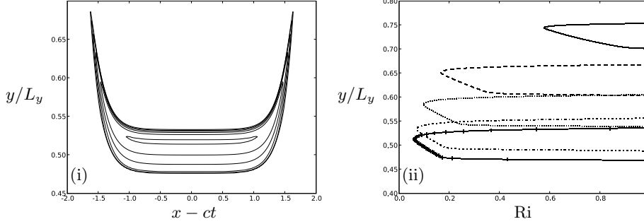
FIGURE 5. Plots of the Richardson number defined as in the main text. The stratification in both plots is such that Y_1/L_y = 0.81 and Y_2/L_y = 0.94 , N_0^2 = N_2^2 = 0 , N_1^2 = 1 . (i) Shows contours of Ri for a wave with amplitude \mathcal{A} = 4.4 \times 10^{-2} the outer contour is for Ri = 0.25, and six contours are presented, evenly spaced in Ri down to the contour Ri = 0.065. The outer two (in some regions three) contours are almost indistinguishable since Ri changes sharply at the edge of the wave. (ii) Shows Ri along cross-sections through the middle ( x = 0 ) of waves with amplitudes \mathcal{A} = 5 \times 10^{-3} (—), 1 \times 10^{-2} (---), 1.5 \times 10^{-2} (⋯), 2.2 \times 10^{-2} (— · —), 4.4 \times 10^{-2} (—+—). of N^2(Y) was set to be one grid length as this more closely matches the stratification in Fructus & Grue (2004) (this sharper transition was found to be important in determining pycnocline thickness, shown in plot (ii) of figure 6). In order to reproduce the curves given in Fructus & Grue (2004), the extension for N^2(Y) for closed streamlines outlined in (2.22) has been used. The current figure can be compared with figure 9(c) of Fructus & Grue (2004). Plot (i) of figure 6 shows the non-dimensionalised wave speed against the measure of amplitude used by Fructus & Grue (2004), namely a/(L_y - Y_1) , where a is once again the maximum deflection of the streamline which coincides with the height Y_1 upstream. The wave speed in plot(i) has been non-dimensionalised by dividing through by the linear long wave speed c_0 . In plot (ii) the thickness of the pycnocline (the region bounded by the streamlines traced from heights Y_1 and Y_2 upstream) at the wave midpoint is shown. Once again the plot is against the amplitude measure preferred
