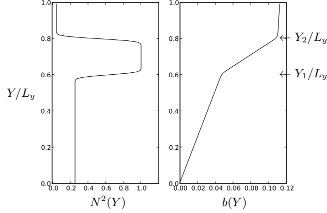
FIGURE 2. Plots of the profiles of N^2 (left) and b (right) for a layered stratified fluid with smoothing as defined in equation (3.1). The parameters used are N_0^2 = 0.25 , N_1^2 = 1 , N_2^2 = 0.04 , Y_1/L_y = 0.6 , and Y_2/L_y = 0.8 with a smoothing distance \delta = 0.015625 , and a domain aspect ratio L_y/2\pi = 0.05 .
