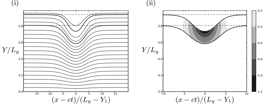
FIGURE 4. (i) The streamfunction \tilde{\psi} and (ii) scaled vorticity \zeta/(2\hat{N}) , for a three layer wave with layer height Y_1/L_y = 0.81 and Y_2/L_y = 0.94 , and N_0^2 = N_2^2 = 0 , N_1^2 = 1 . The wave shown has amplitude \mathcal{A} = 0.011 , and is matched in setup and amplitude to that shown in figure 6 of Fructus & Grue (2004). The bold lines are streamlines coinciding with the heights Y_1/L_y and Y_2/L_y at the domain edge, while dashed lines mark the layer heights Y_1/L_y and Y_2/L_y .
