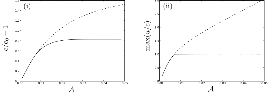
FIGURE 8. (i) Shows the non-dimensional wave speed versus the amplitude of the wave \mathcal{A} . (ii) Shows the maximum dimensionless horizontal velocity u/c versus \mathcal{A} . In both plots the approach outlined in (2.23) having a uniform density core is shown by a solid line, while that outlined in (2.22) is shown by a dashed line. The background stratification for these waves is Y_1/L_y = 0.81 , Y_2/L_y = 0.94 , and N_0^2 = 0 , with N_2^2 = N_1^2 = 1 , as in figure 7 above.
