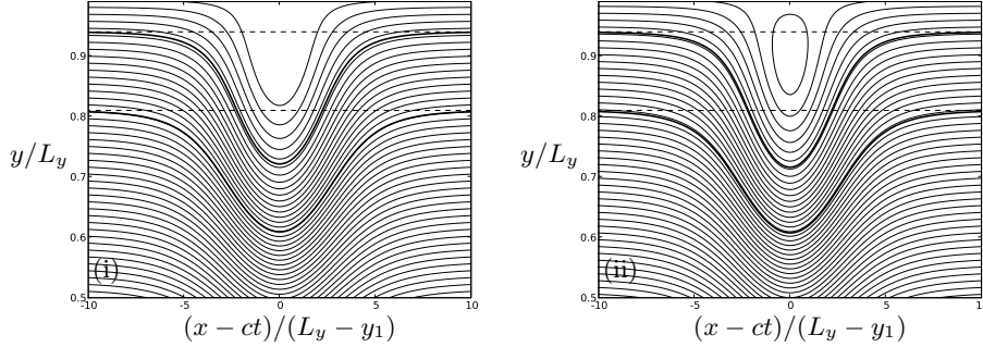
FIGURE 7. Plots of the streamlines for a wave with amplitude \mathcal{A} = 0.009 , with equal intervals of 2 \times 10^{-4} chosen for the levels of the streamfunction. Only the top half of the domain is shown. The underlying stratification for the computations is Y_1/L_y = 0.81 , Y_2/L_y = 0.94 , and N_0^2 = 0 , with N_2^2 = N_1^2 = 1 , giving a two layered structure. Both layer heights are plotted although the upper layer height does not correspond to a change in stratification. The layer heights Y_1/L_y and Y_2/L_y are plotted with dashed lines. (i) Is a calculation performed with the procedure outlined by (2.23), while (ii) was obtained by use of (2.22). (ii) Corresponds to the larger amplitude case plotted by Fructus & Grue (2004) in their figure 15.
