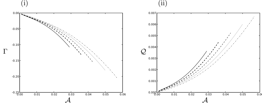
FIGURE 18. (i) Circulation \Gamma (see equation 3.6) and (ii) buoyancy anomaly Q (see equation 3.7) versus \mathcal{A} . In both plots the parameters and the line styles used are given in table 1.
