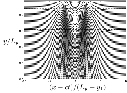
FIGURE 9. Plots of the streamlines for a wave with amplitude \mathcal{A} = 0.009 , with equal intervals of 2 \times 10^{-4} chosen for the levels of the streamfunction. Only the top half of the domain is shown. The underlying stratification and line styles are as for figure 7. This wave has a constant density but non-zero constant vorticity core as discussed in section 2.1.
