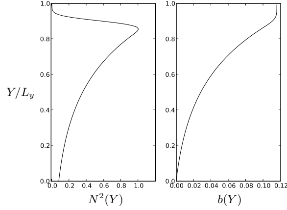
FIGURE 20. Plots of both the profiles of N^2(Y) and b(Y) for a fluid stratified according to 3.9. The parameters used for the plot have values: \alpha_0 = 3 , \beta_0 = 30 , and Y_0 = 0.9 , and the domain has aspect ratio 0.05.
