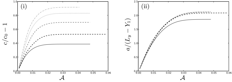
FIGURE 15. (i) Non-dimensionalised wave speed against the amplitude of the wave \mathcal{A} . (ii) Shows a typical measure of amplitude used in many previous studies ( a/(L_y - Y_1) , where a is the maximum deflection of the streamline which coincides with the height Y_1 upstream) plotted against the current amplitude measure \mathcal{A} . The plot is for parameter values and line styles as given in table 2.
