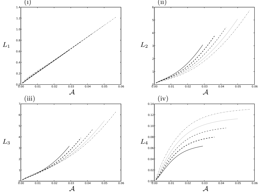
FIGURE 19. (i)-(iv) Length scales L_1 - L_4 as defined in the text. Parameter values and the line styles used for the plots are taken from table 1.
