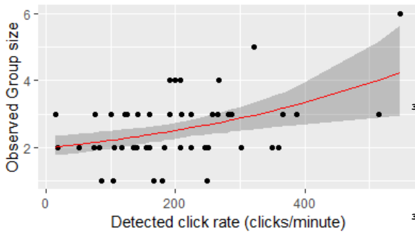
345 Figure 1: Observed group sizes and corresponding detected click rate (black dots), along with the modelled relationship (red line), and the model's bootstrap 95% percentile interval for the mean group size (grey area).
