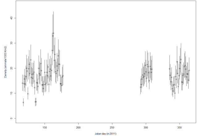
Figure 2: Daily density estimates with the corresponding bootstrap 95% confidence intervals.
