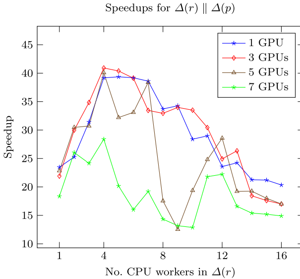
Fig. 5 Speedup figures for the image convolution configuration \Delta(r) \parallel \Delta(p) , with 0 CPU and a different number of GPU workers for \Delta(p)
