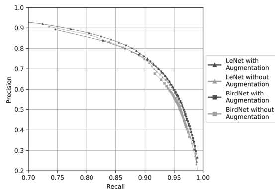
Figure 3. Precision-recall curves of LeNet and BirdNet with and without data augmentation. LeNet with and without data augmentation had average precisions of 0.903 and 0.898, respectively. BirdNet with and without data augmentation had average precisions of 0.891 and 0.830, respectively.
