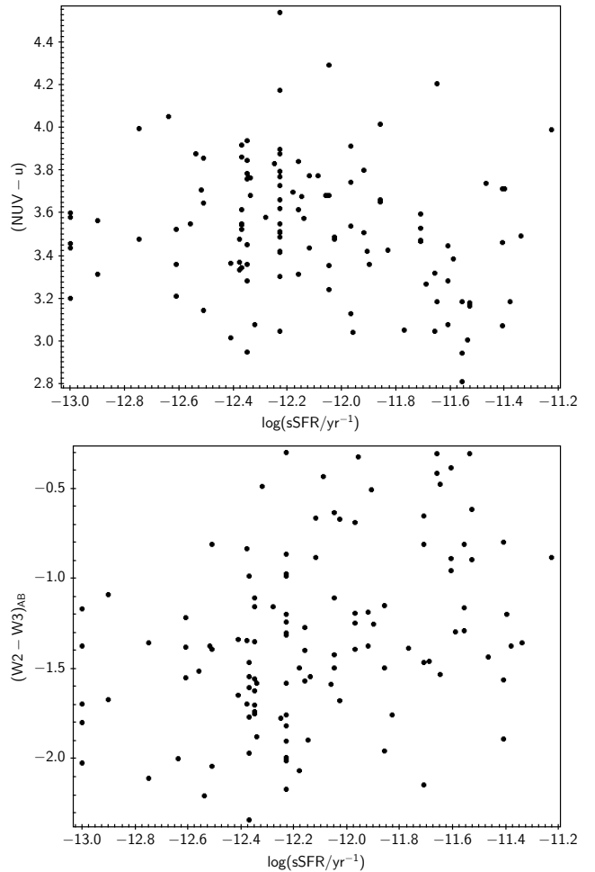
Figure 6. MAGPHYS derived specific star formation rates (averaged over the last 0.1 Gyr) plotted against rest-frame (\text{NUV}-u) colour (top panel) and (W2-W3)_{AB} (bottom panel) for our final NUV+WISE red sequence sample.
