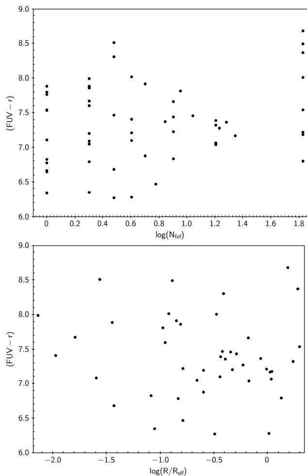
Figure 11. (FUV-r) colour versus the host galaxy group multiplicity (top panel) and versus radial distance, normalised by group effective radius, (bottom panel) for the final NUV+ WISE red sequence sample.
