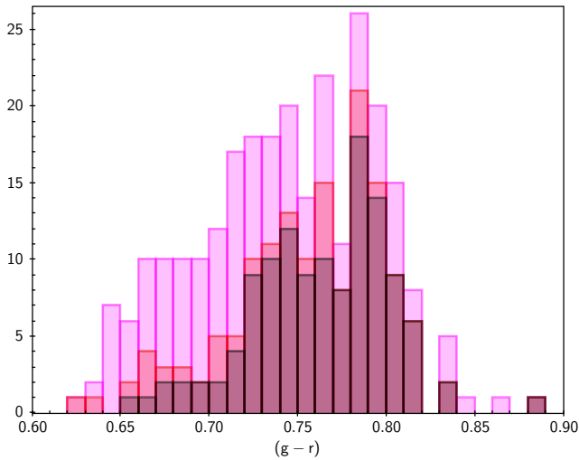
Figure 5. Histograms of the optical rest-frame ( g-r ) colours for the various red sequence selections, colour coded as before. The final NUV+WISE sample has a significantly narrower range compared to the original sequence, but simply choosing galaxies redder than, say, 0.72 would still include potential weak star formers (pink and red histograms) in addition to the members of our ‘best’ sample (dark red histogram with black outlines). Photometric errors are around 0.03 magnitudes.
