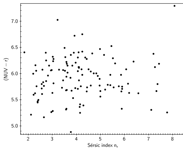
Figure 12. Distribution of rest-frame (NUV-r) colour for the NUV+ WISE red sequence galaxies as a function of r -band Sérsic index.
